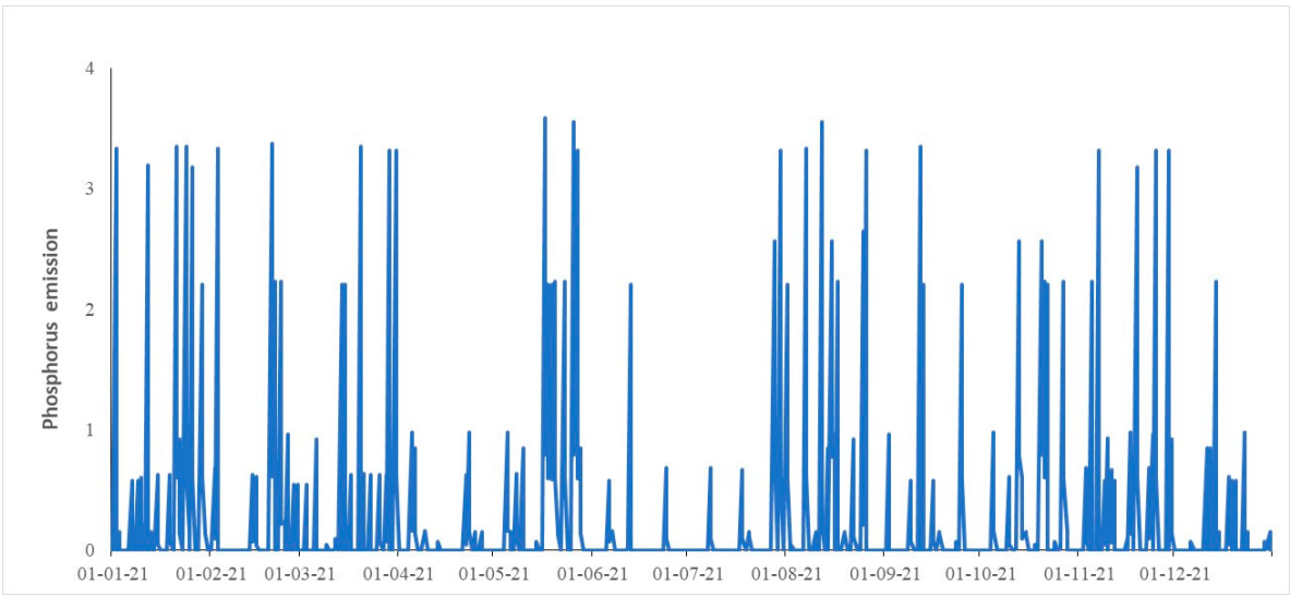
Figure 6. Predicted daily dynamics of total phosphorus discharge from fertilizer loading to the marine environment. should be placed in the main text near to the first time they are cited.
