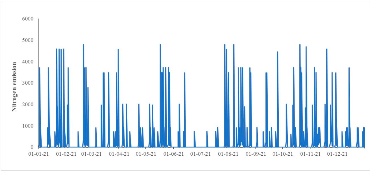
Figure 5. Predicted daily dynamics of total nitrogen discharge from fertilizer loading to the marine environment.
