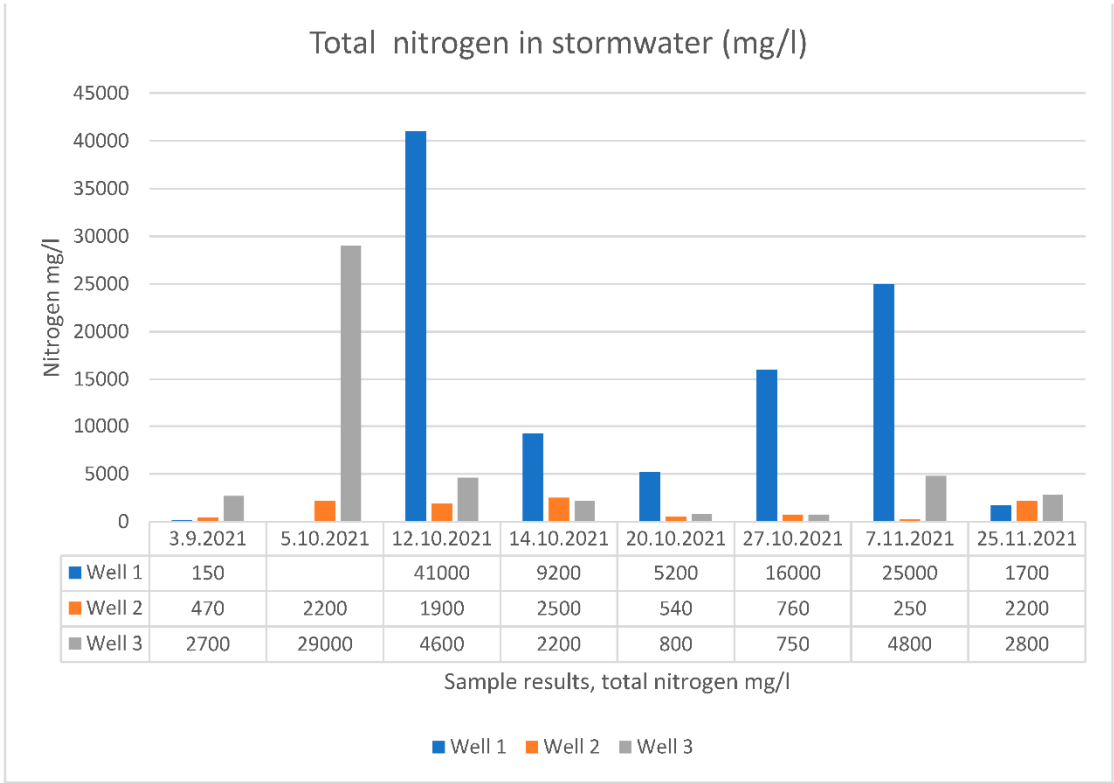
Figure 1. Total Nitrogen concentration in stormwaters (mg/l). Well 1 displays highest nitrogen concentrations.
