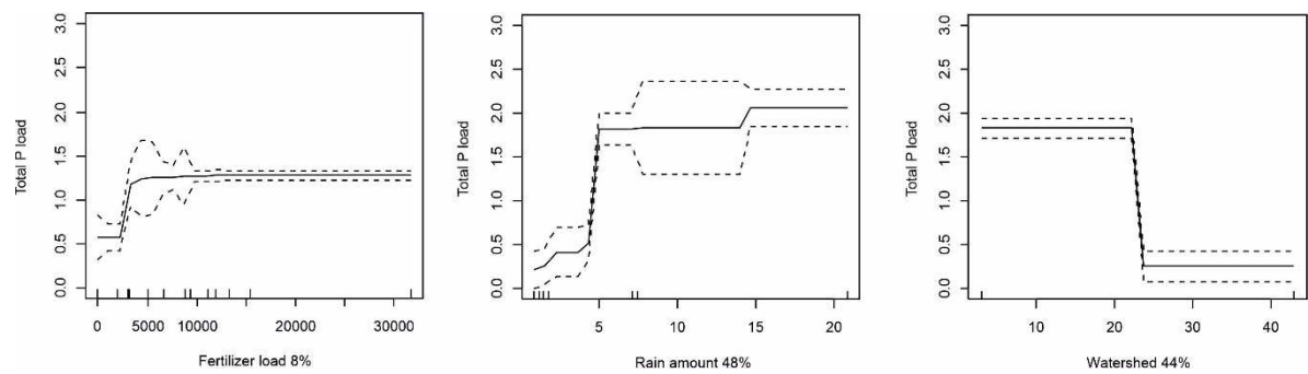
Figure 4. Standardized functional-form relationships showing the effect of environmental variables on total phosphorus discharge from fertilizer loading to the marine environment, whilst all other variables are held at their means. The relative contribution of variables in the BRT model is indicated by the variable name. Upward tickmarks on x-axis show the frequency of distribution of data along this axis.
