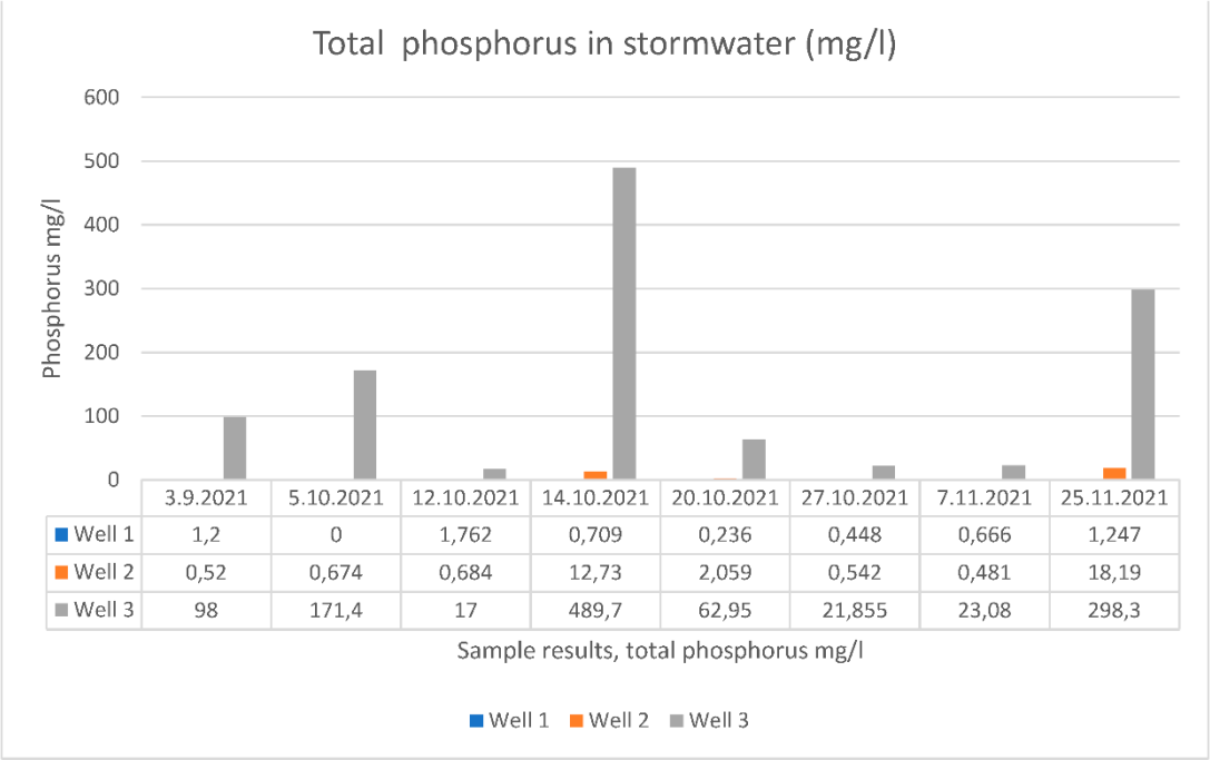
Figure 2. Total phosphorus in stormwaters (mg/l). Well 3 displays highest concentrations as most of the phosphorus fertilizers are loaded in that area.
