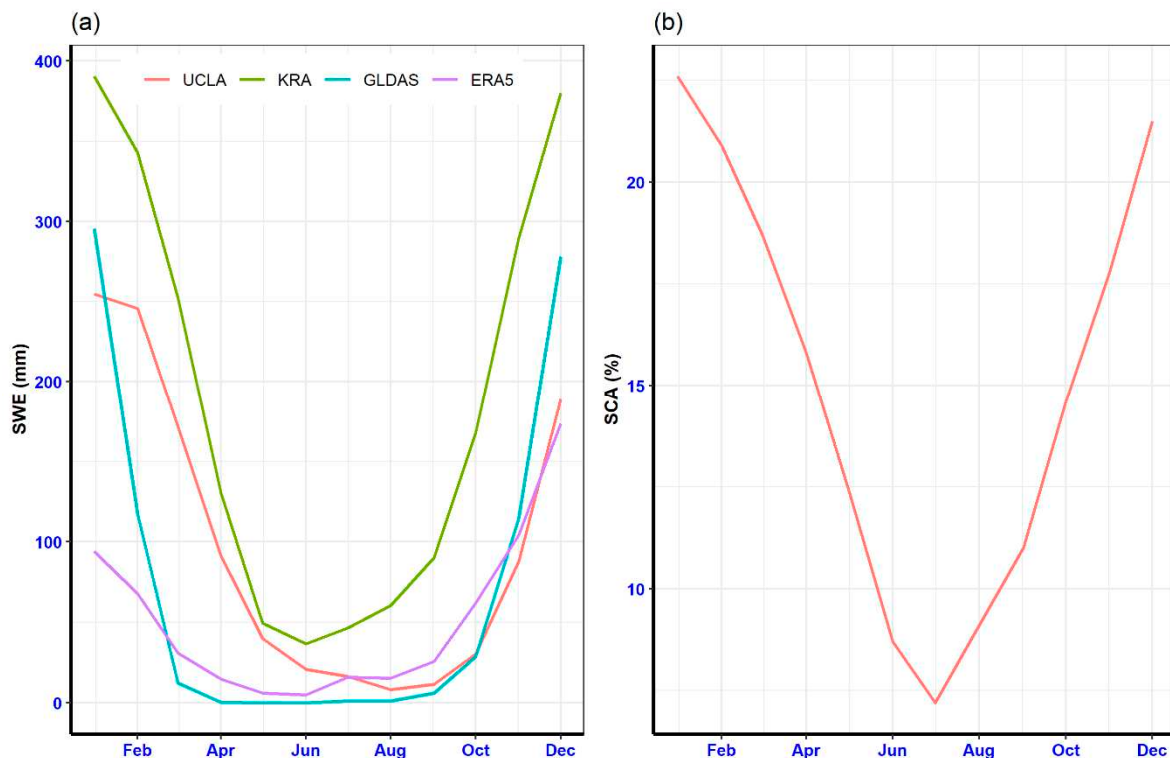
Figure 5. Inter-product comparison of spatially averaged SWE at monthly scale (a) global SWE products and (b) MODIS snow cover area (SCA) in the CRB.
