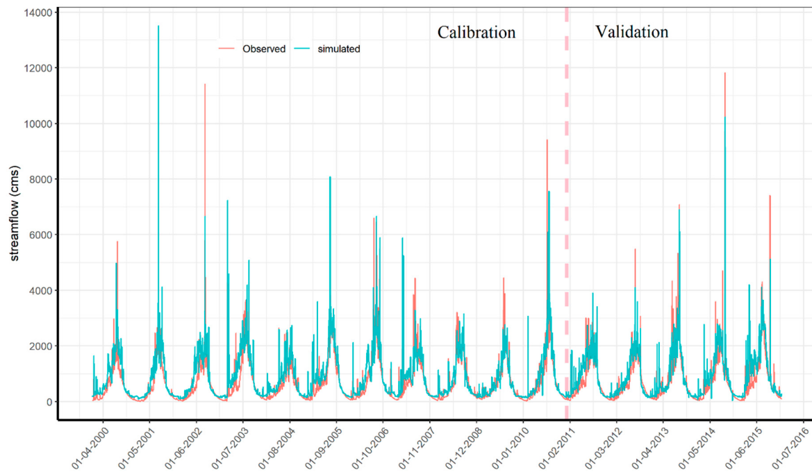
Figure 9. Daily streamflow simulation using single variable calibration approach during calibration (2000 to 2011) and validation (2011-2015) in the CRB.
