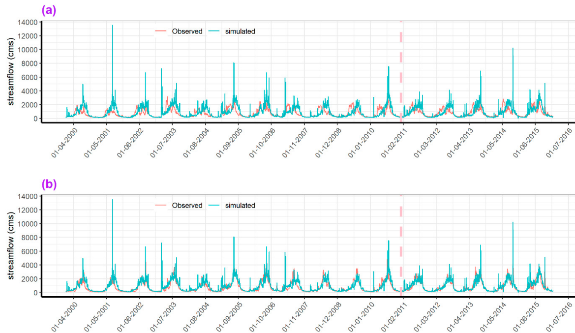
Figure 11. Daily streamflow simulation with multi-variable calibration approach using observed streamflow and snow reference data from (a) UCLA-SWE and (b) KRA-SWE in the CRB.
