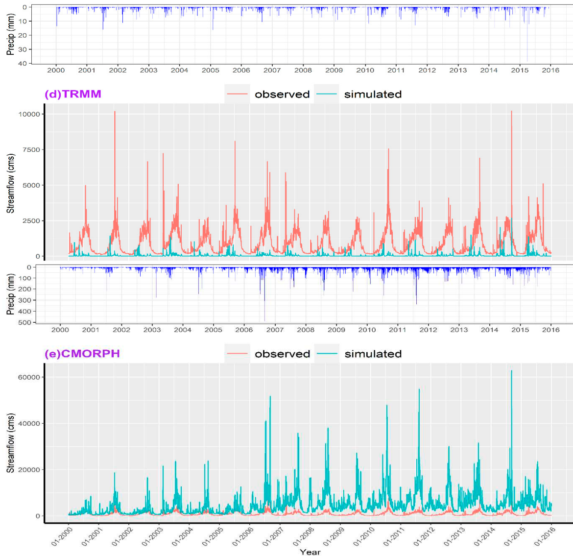
Figure 7. Model performance with various precipitation datasets for daily streamflow during 2000-2015. Streamflow simulation is conducted with default SWAT parameters by input data from the satellite and reanalysis precipitation products such as (a) ERA5-Land (b) CPCUPP (c) APHRODITE (d) TRMM (e) CMORPH.
