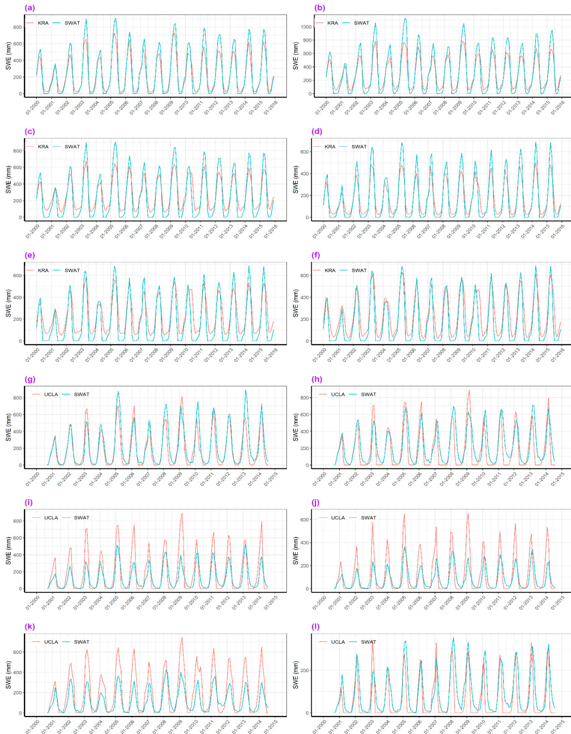
Figure 13. Simulated SWAT-SWE using KRA-SWE and UCLA-SWE product in selected sub-basins for KRA-SWAT SWE (a-f) and UCLA-SWAT(g-l) in selected sub-basins (BSN01, BSN02, BSN05, BSN12, BSN13, and BSN17) of the CRB.
