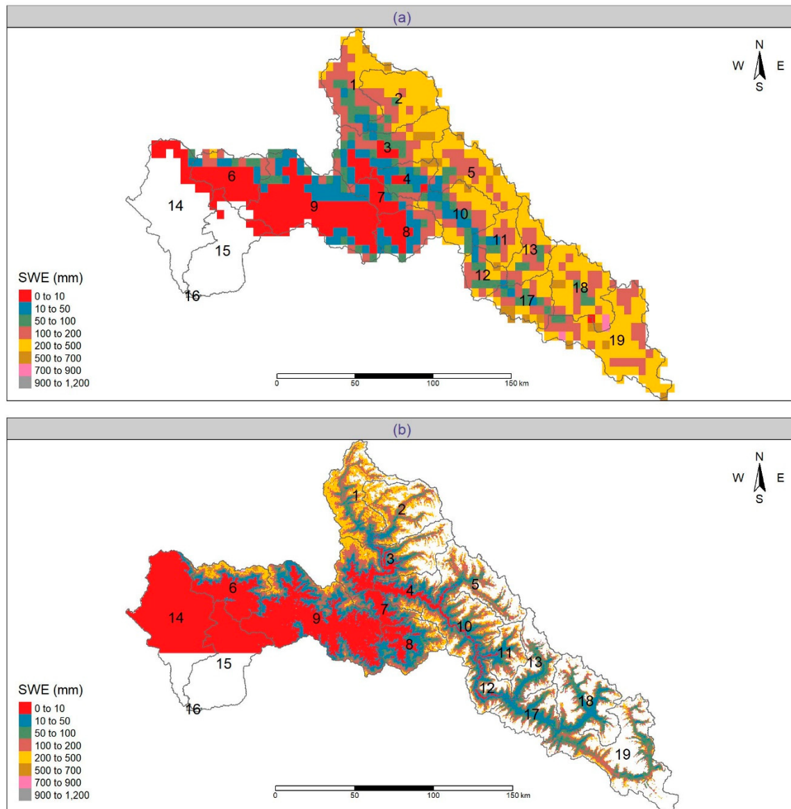
Figure 6. Comparison of spatial distribution of SWE in each sub-basin (a) UCLA-SWE (b) KRA-SWE in the Chenab River Basin (CRB).
