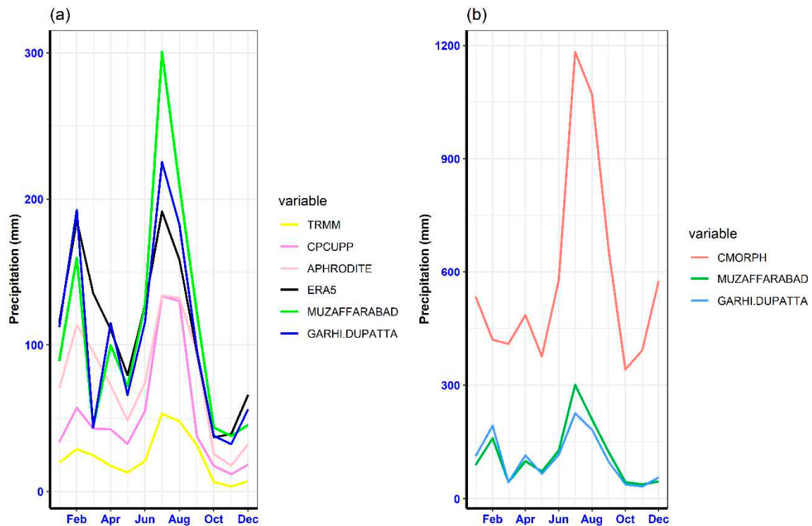
Figure 4. Monthly precipitation comparison of satellite gridded and Reanalysis precipitation (SGRP) products with station data (a) TRMM, CPCUPP, APHRODITE, ERA5 with station data (b) CMORPH with station data.
