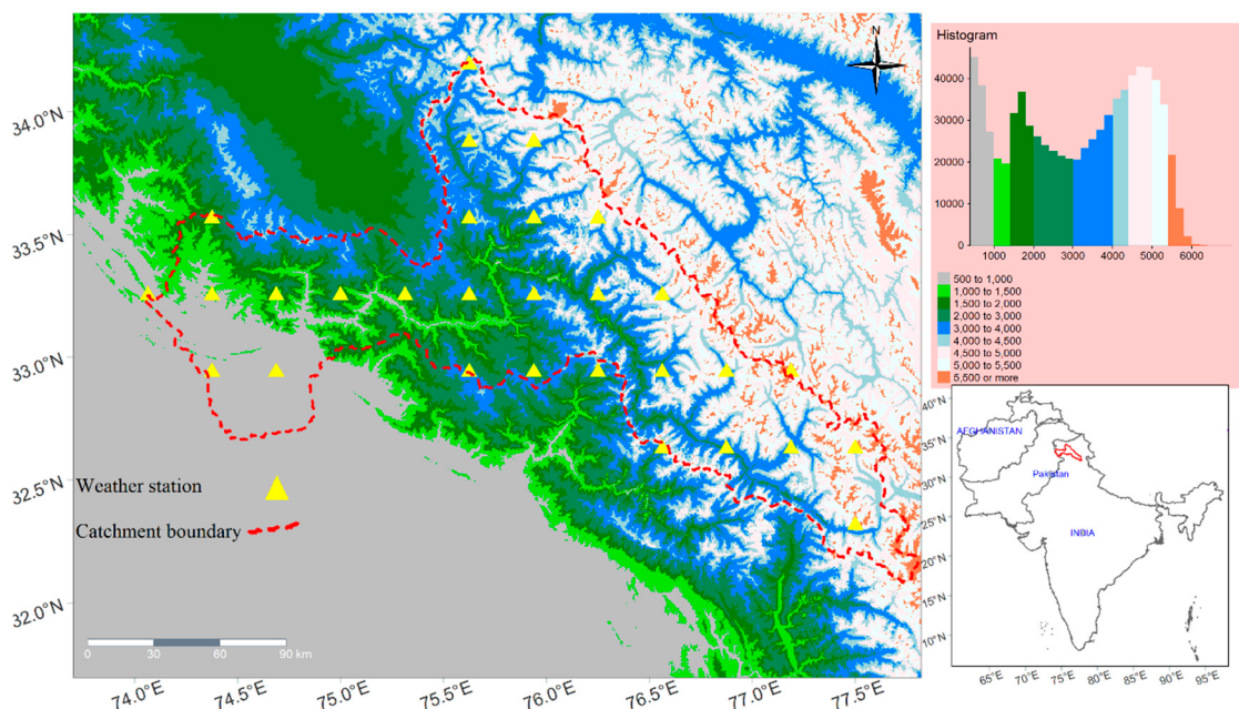
Figure 1. Study area map of the Chenab River Basin (CRB) and weather station points used to extract data from satellite and reanalysis products.
