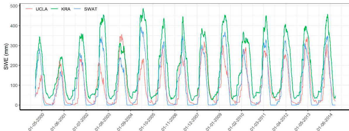
Figure 10. Comparison of simulated SWE (SWAT-SWE) with UCLA-SWE and KRA-SWE in the CRB with single variable calibration approach.
