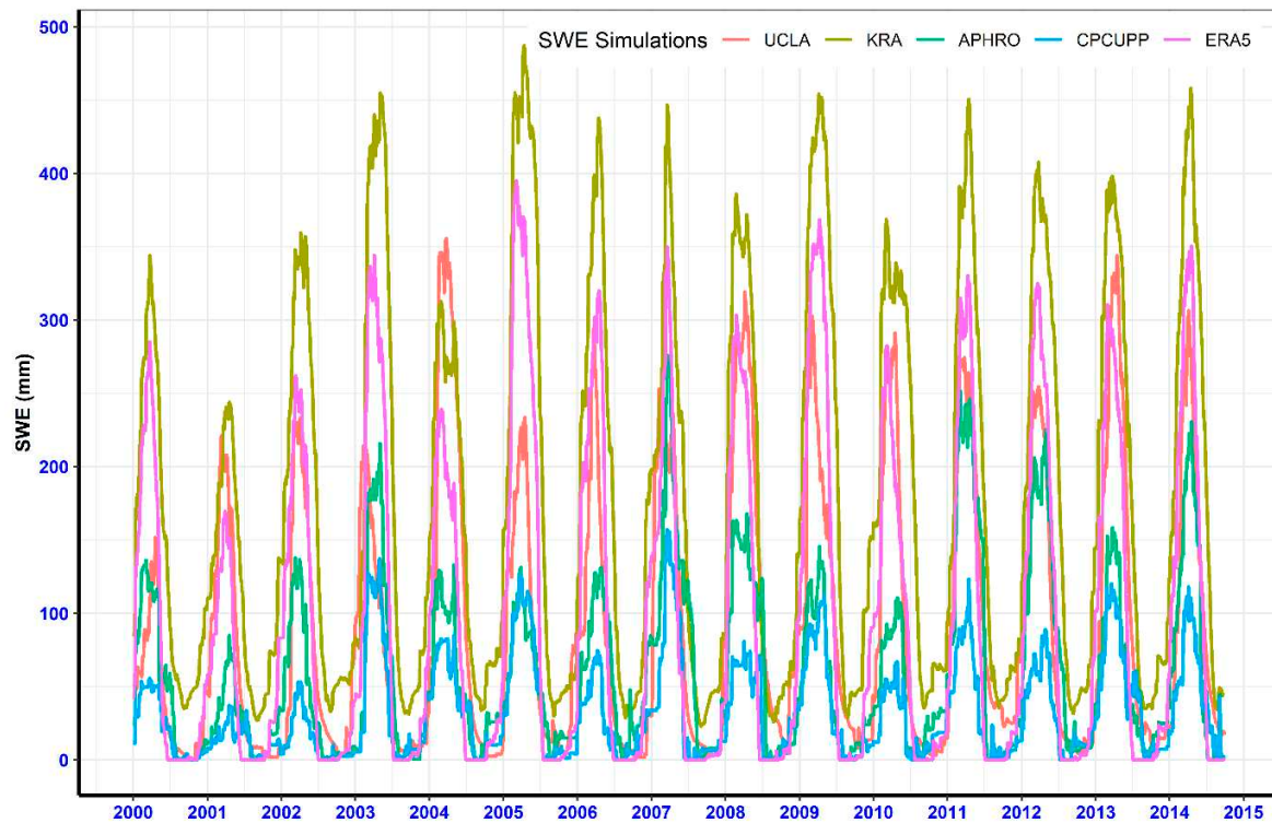
Figure 8. Daily snow water equivalent (SWE) simulation with SWAT model run with precipitation data from APHRODITE, CPCUPP and ERA5-Land and comparison with SWE products (UCLA and KRA) in the CRB. TRMM and CMORPH data is not shown here due to their poor performance.
