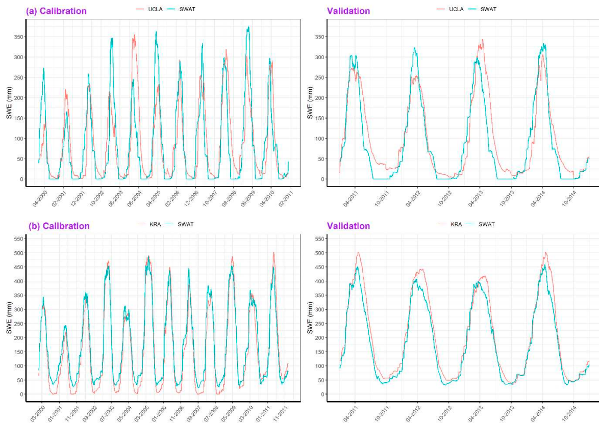
Figure 12. Comparison of simulated SWE (SWAT-SWE) with UCLA-SWE and KRA-SWE in the CRB. In panel (a), simulated SWE using UCLA-SWE product during calibration and validation period while panel (b), simulated SWE using KRA SWE product during calibration and validation period are shown.
