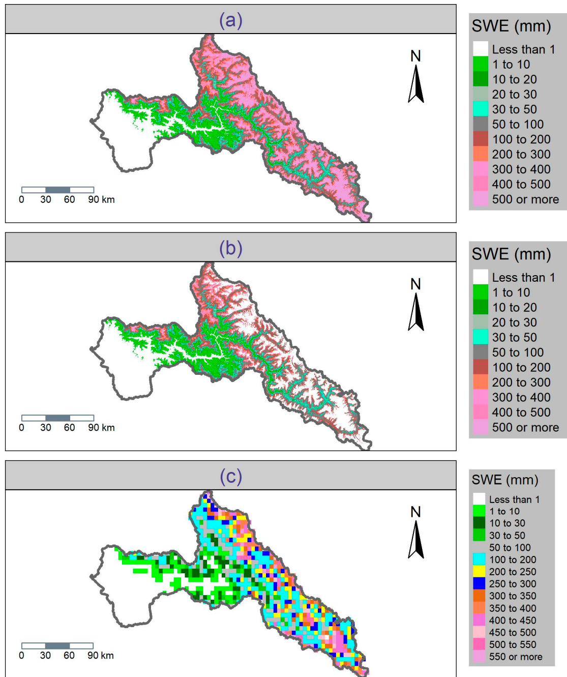
Figure 3. Snow water equivalent (SWE) products (a) UCLA SWE (without masking non-seasonal snow/ice) (b) UCLA SWE (masking non-seasonal snow/ice pixels) (c) KRA SWE in the CRB. In legend, values less than 1 are considered as no data or masked area.
