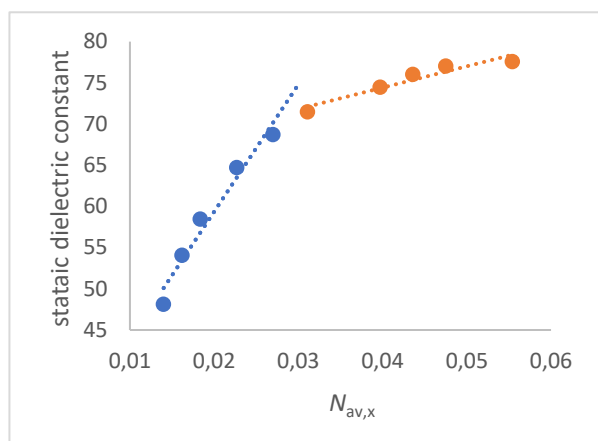
Figure S7. Correlation of the static dielectric constant of DMSO /water mixtures [143] as function of N_{av,x} (mol/cm³). 37
