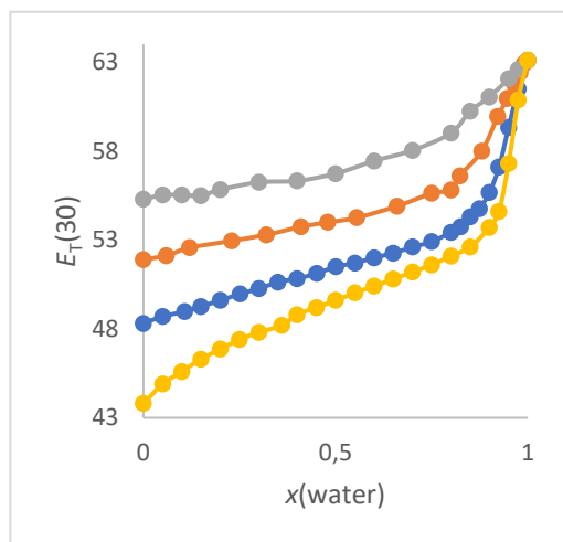
Figure S10. Correlations of E_T(30) as function of x(\text{water}) for methanol/water (grey), ethanol/water (red), 2-propanol/water (blue), and 2-methyl-2-propanol/water (yellow) mixtures. Data from [2, 17-19].
