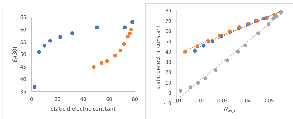
Figure S8a (left panel). Correlation of E_T(30) (kcal/mol) as function of the static dielectric constant \epsilon_r for DMSO/water (red) [143] and 1,4-dioxane/water mixtures [152] (blue); Figure S8b (right panel). Correlation of the static dielectric constant \epsilon_r as function of N_{av,x} (mol/cm³) for several co-solvent/water mixtures including the pure co-solvents, 1,4-dioxane/water mixtures [154]: \epsilon_r = 1827 N_{av,x} - 25 ; n = 11 ; r = 0.996 (grey dots), 1,2-ethanediol/water mixtures, \epsilon_r = 975 N_{av,x} + 25 ; n = 11 ; r = 0.994 (blue dots) and the glycerol/water mixtures, \epsilon_r = 908 N_{av,x} - 29 ; n = 11 ; r = 0.999 (red dots) are used as independent reference. 39 40 41 42 43 44
