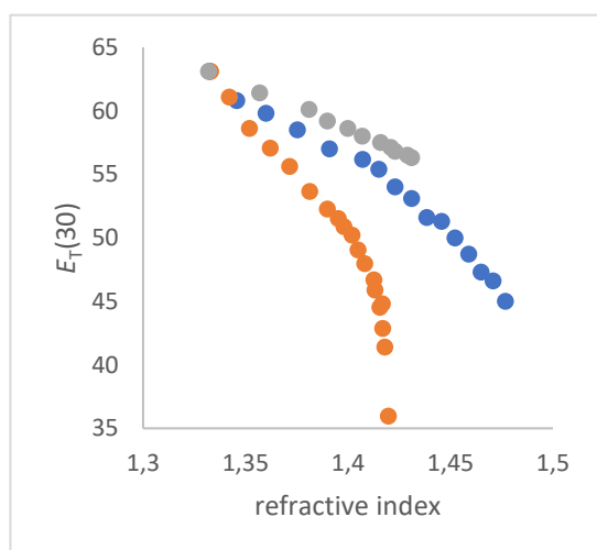
Fig. S2 Plots of E_T(30) (kcal/mol) as function of n_D^{20} for 1,2-ethanediol/water (grey), DMSO/water (blue) and 1,4-dioxane/water (red) mixtures.
