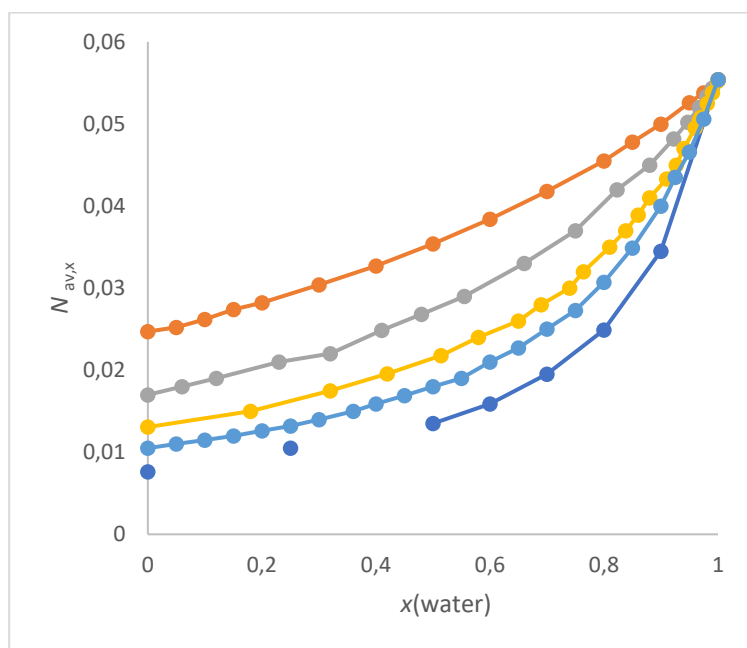
Figure S1. . Plots of N_{av,x} (sum of total OH dipoles) (in mol/cm 3 ) as function of x(\text{water}) for methanol/water (red dots), ethanol/water (grey dots) 2-propanol/water (yellow dots), 2-methyl-2-propanol/water (light blue dots); 2-n-butoxyethanol/water (deep blue) mixtures, physical data from references [ 198-202].
