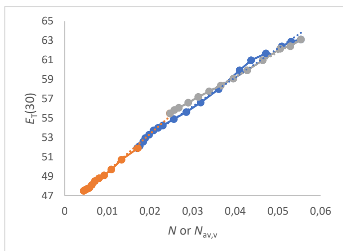
Figure S6. Overall correlation of E_T(30) (kcal/mol) as function of N for the homologous series of primary alcohols (red dots) as well as E_T(30) as function of N_{av,v} (mol/cm 3 ) for ethanol/water mixtures (blue dots) and methanol/water mixtures (grey dots). All E_T(30) data from [2] and [34].
