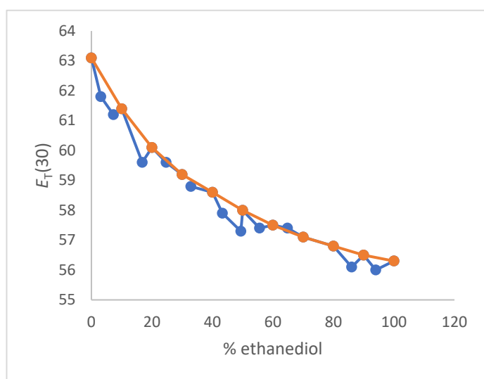
Figure S5. Comparison of E_T(30) (kcal/mol) as function of x(1,2\text{-ethanediol}) (in mol %) for 1,2-ethanediol/water mixtures, data from Kosower/Marcus [12] (red dots) (25 °C) ; data from O. Connor [15] (blue dots).
