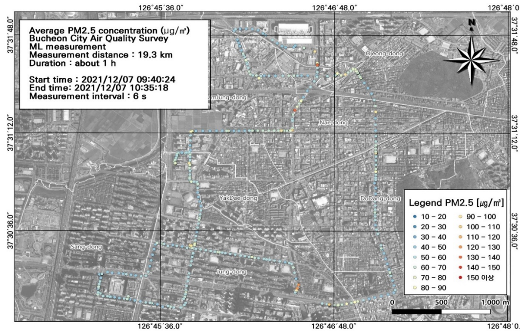
Figure 7. Spatial and temporal plots of ultrafine particulate matter ( PM_{2.5} ) concentrations measured by the mobile laboratory (ML): (a) December 6, first run; (b) December 6, second run; (c) December 6, third run; (d) December 6, fourth run; (e) December 6, fifth run; (f) December 7, first run; (g) December 7, second run.
