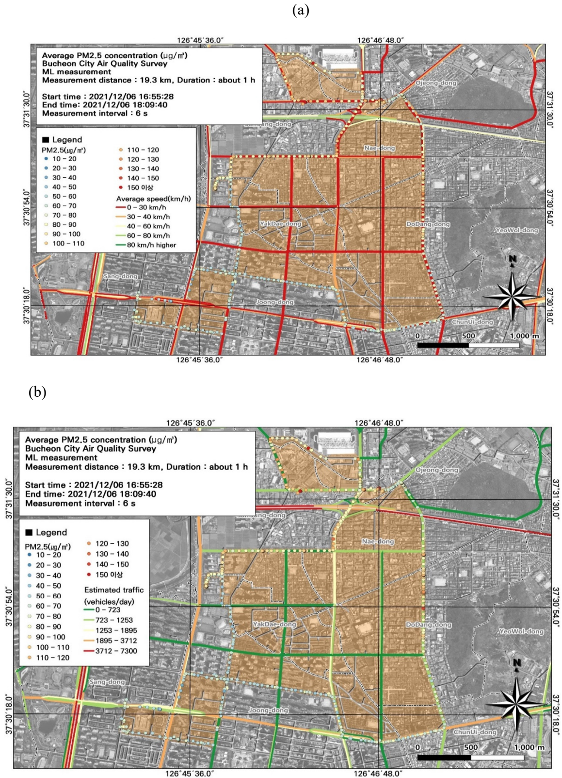
Figure 8. Association between ultrafine particulate matter (PM 2.5 ) concentrations with (a) average traffic speed and (b) estimated traffic volume during the evening rush hour from Figure 7(e).
