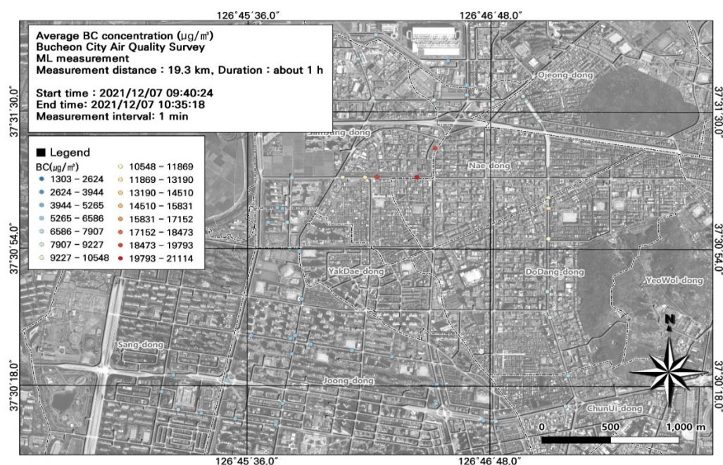
Figure 9. Spatial and temporal plots of ultrafine black carbon (BC) concentrations measured by the mobile laboratory (ML): (a) December 6, first run; (b) December 6, second run; (c) December 6, third run; (d) December 6, fourth run; (e) December 6, fifth run; (f) December 7, first run; (g) December 7, second run.
