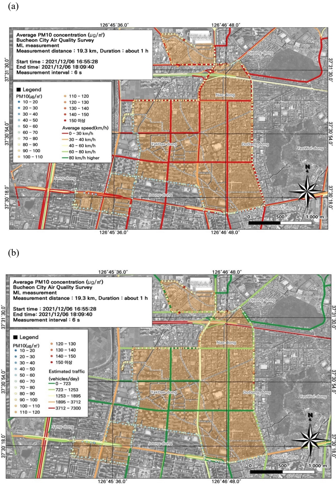
Figure 6. Association between ultrafine particulate matter (PM 10 ) concentrations with (a) average traffic speed and (b) estimated traffic volume during the evening rush hour from Figure 5(e).
