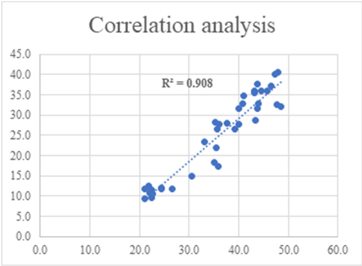
Figure 3. Correlation analysis of the fine particulate matter datasets obtained from the PMM-304 and Grimm 11-D instruments.
