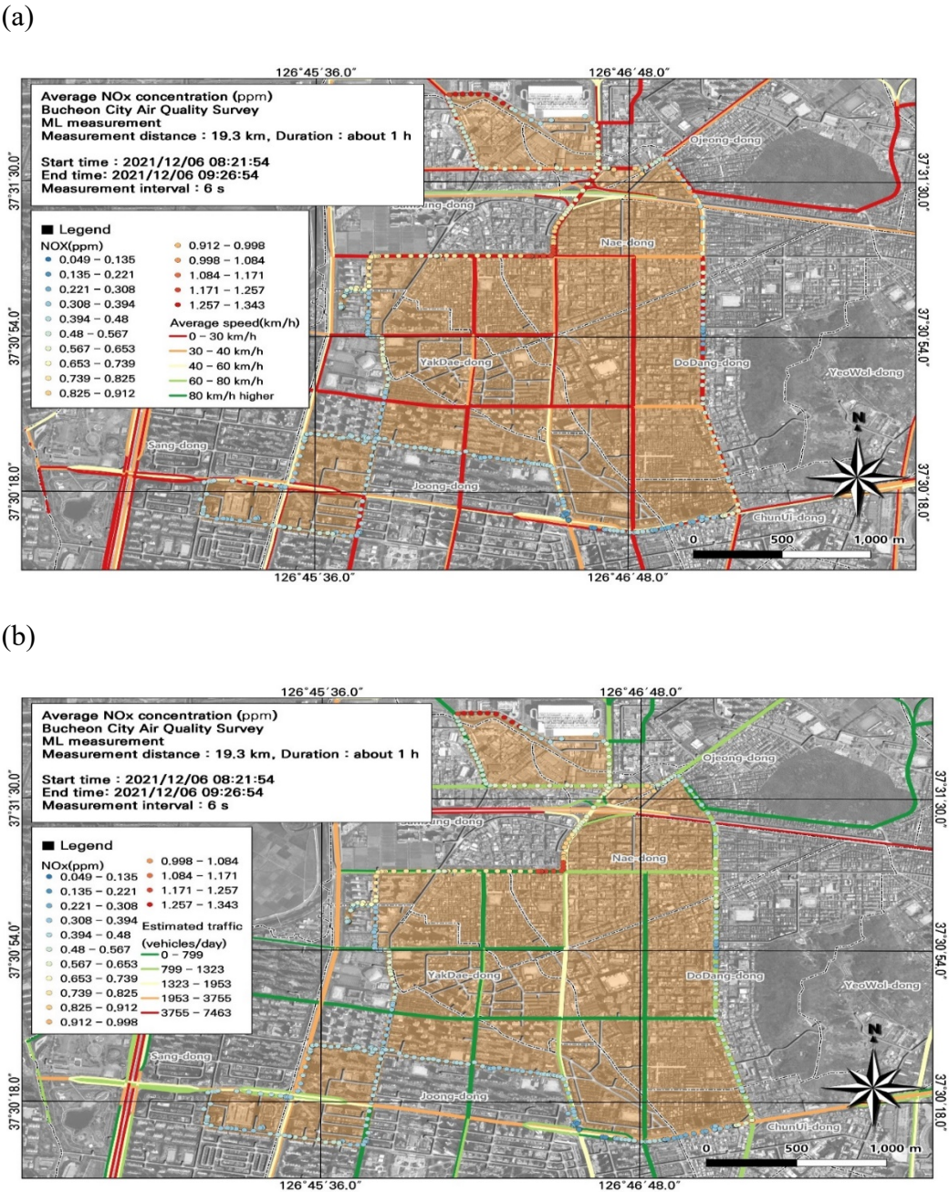
Figure 12. Association between nitrogen oxide (NO x ) concentrations with (a) average traffic speed and (b) estimated traffic volume during the morning rush hour from Figure 11(a).
