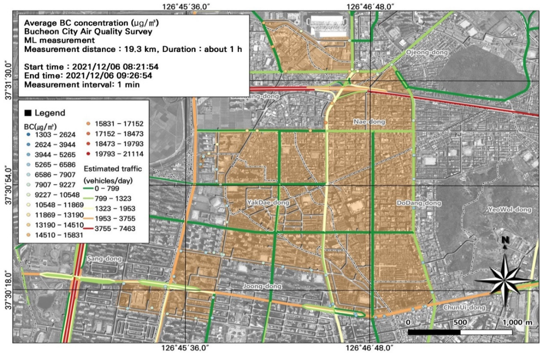
Figure 10. Association between black carbon (BC) concentrations with (a) average traffic speed and (b) estimated traffic volume during the morning rush hour from Figure 9(a).
