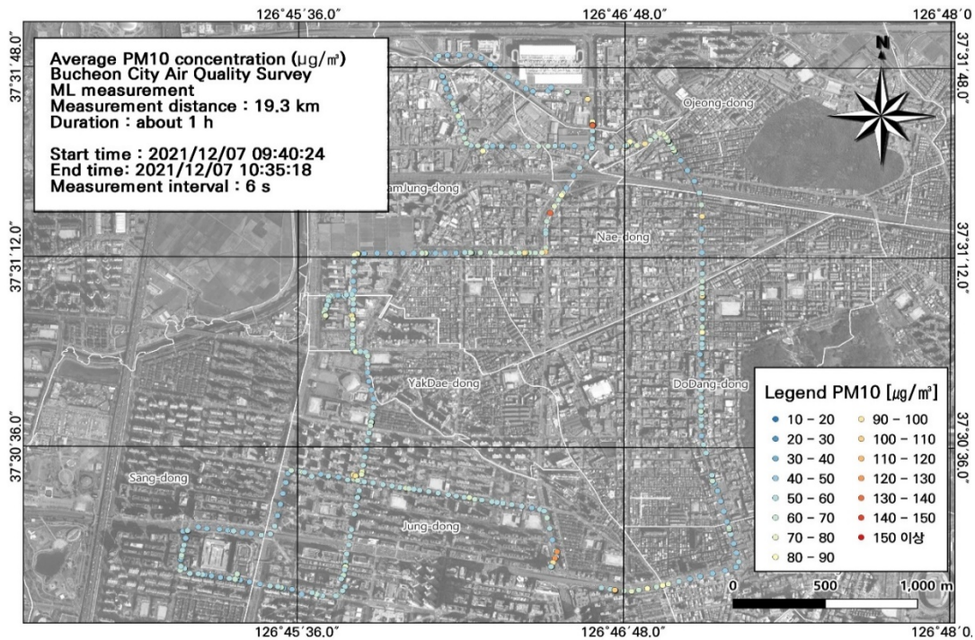
Figure 5. Spatial and temporal plots of ultrafine particulate matter ( \text{PM}_{10} ) concentrations measured by the mobile laboratory (ML): (a) December 6, first run; (b) December 6, second run; (c) December 6, third run; (d) December 6, fourth run; (e) December 6, fifth run; (f) December 7, first run; (g) December 7, second run.
