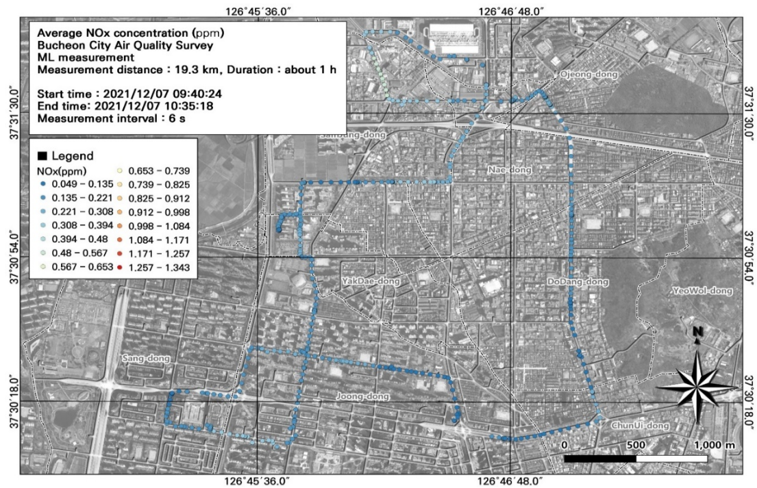
Figure 11. Spatial and temporal plots of nitrogen oxide (NO x ) concentrations measured by the mobile laboratory (ML): (a) December 6, first run; (b) December 6, second run; (c) December 6, third run; (d) December 6, fourth run; (e) December 6, fifth run; (f) December 7, first run; (g) December 7, second run.
