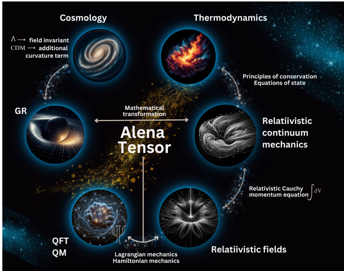
Figure 1. Alena Tensor framework
