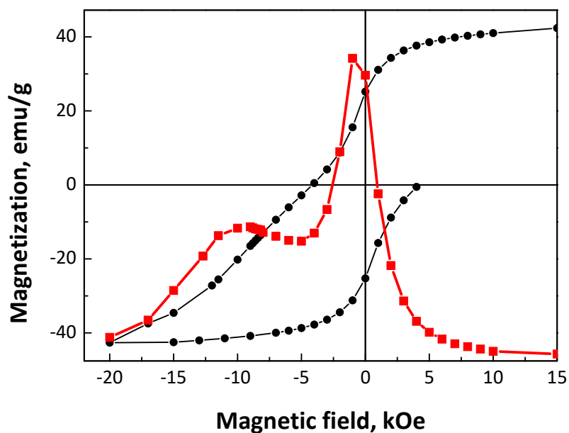
Figure S3. Magnetic hysteresis loop of the annealed at 700 °C for 2h sample, ( black line and symbols ), and the 1 st derivative of M vs H curve ( red line and symbols ). The derivative curve is shifted for sake of visualization.
