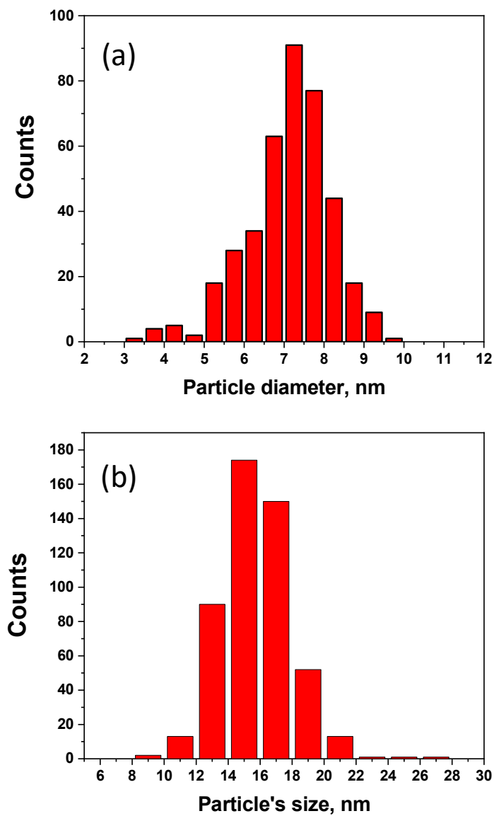
Figure S1. Size distribution histograms of as-made (a) and annealed at 700 °C / 7h (b) CoPt nanoparticles.
