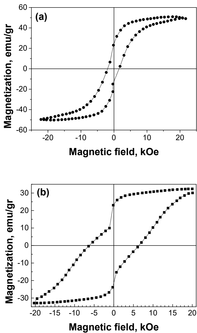
Figure S4. Room temperature hysteresis loops of CoPt nanoparticles after annealing at 675 °C for 1.5h (a) and 4h (b).
