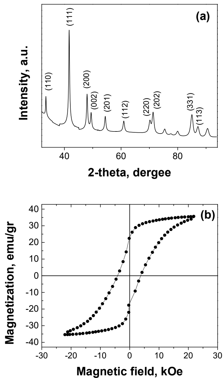
Figure S5. XRD pattern (a), and room temperature magnetic hysteresis loop (b), of equiatomic bimetallic CoPt nanoalloys, after annealing under reducing atmosphere at 700 °C for 4h.
