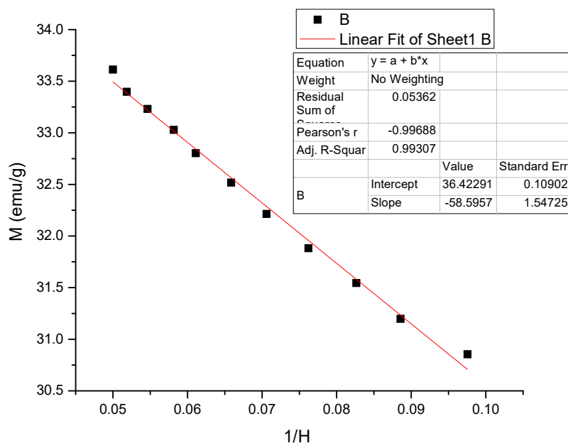
Figure S2. M vs. 1/H curve of CoPt nanoalloys annealed at 700 °C / 7h.
