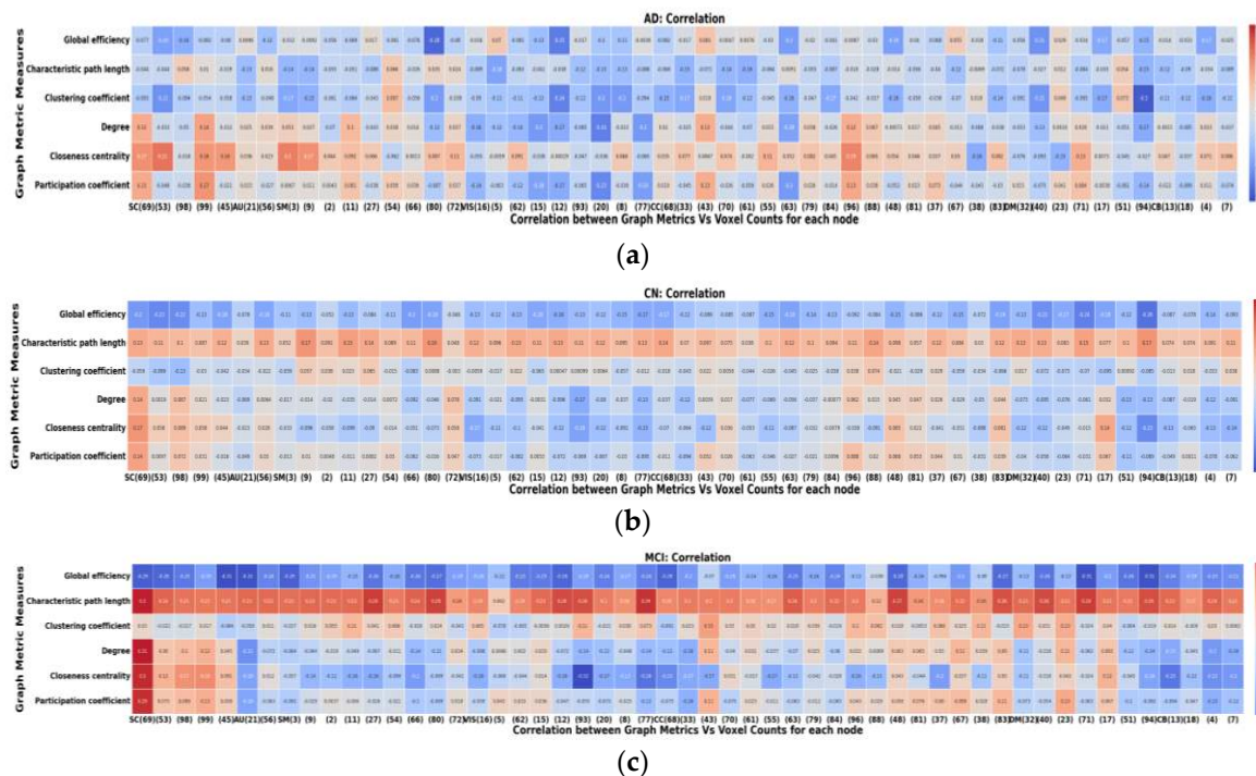
Figure 7. (a) correlation between node size and the global and local metrics in AD group. (b) Correlation between node size and the global and local metrics in HC. (c) Correlation between node size and the global and local metrics in MCI.
