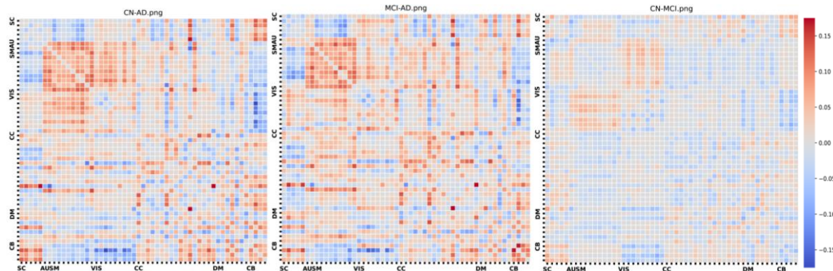
Figure 3. Group differences.
