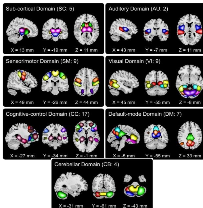
Figure 1. Fifty-three ICNs categorized into seven functional domains.
