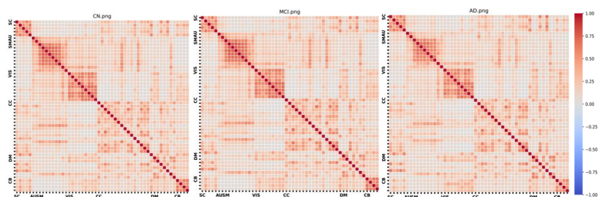
Figure 2. FNC matrices for each group.
