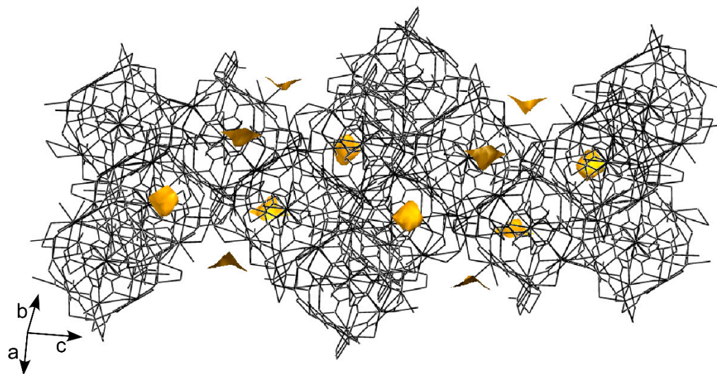
Figure 3. Crystal packing of compound 1 showing the isolated voids (golden solid) containing water molecules.
