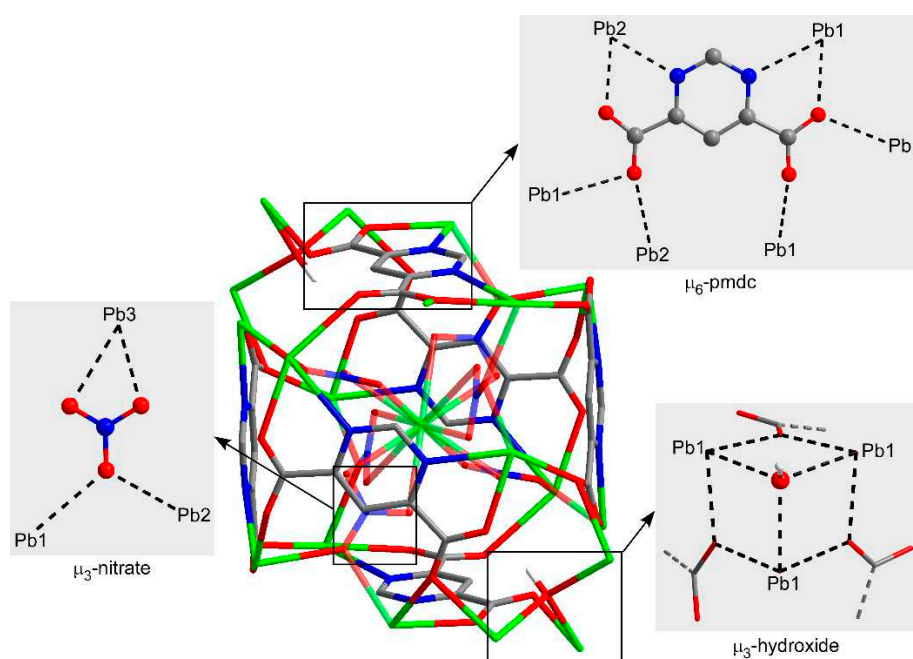
Figure 2. Coordination modes of the ligands within cubic building unit of compound 1. Colour codes: carbon, grey; hydrogen, white; nitrogen, blue; oxygen, red; lead, green.
