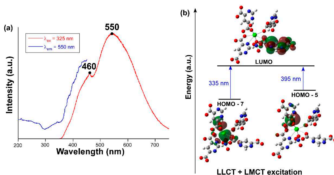
Figure 5. (a) Experimental excitation (blue) and emission (red) spectra of 1 at RT. (b) Schematic representation of the most relevant calculated excitations.
