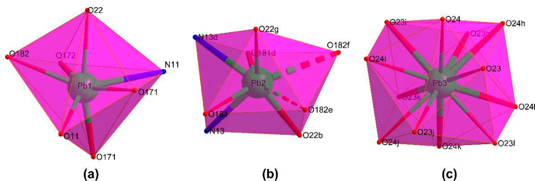
Figure 1. Coordination shells of the crystallographically independent metal ions: (a) Pb1, (b) Pb2 and (c) Pb3. Colour codes: nitrogen, blue; oxygen, red; lead, green.
