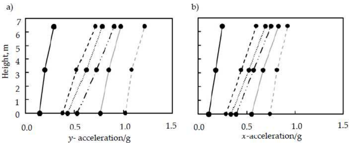
Figure 10. Reinforced prototype: a) y -acceleration profile, b) x -acceleration profile.
