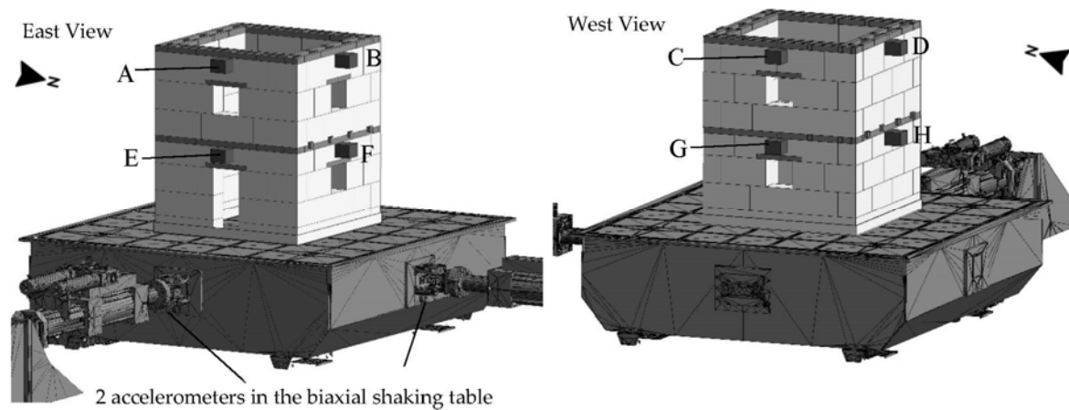
Figure 6. Location of accelerometers A to H.
