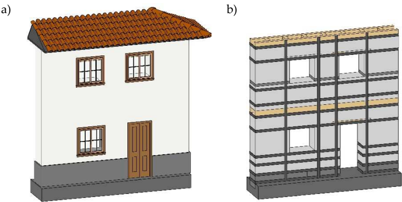
Figure 1. a) Typical façade of an Andean heritage earthen house b) Reinforcement of the earthen wall with steel plates.
