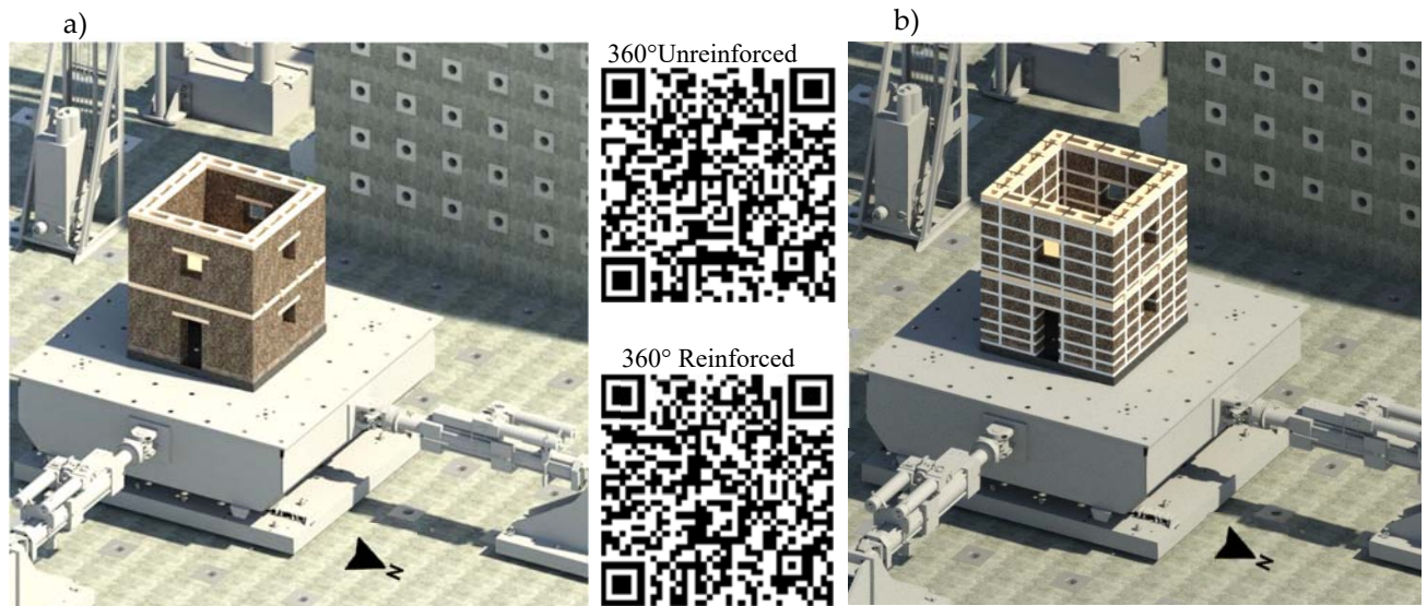
Figure 5. Test Set Up. a) Unreinforced model; b) reinforced model. Link for QR code 360° Unreinforced model: https://pano.autodesk.com/pano.html?mono=jpgs/183016e4-f29c-4ede-95c9-bfe33a7024d3&version=2 . Link for QR code 360° Reinforced model: https://pano.autodesk.com/pano.html?mono=jpgs/6d32568d-f123-4ce6-9d34-4675c3ce6dc1&version=2
