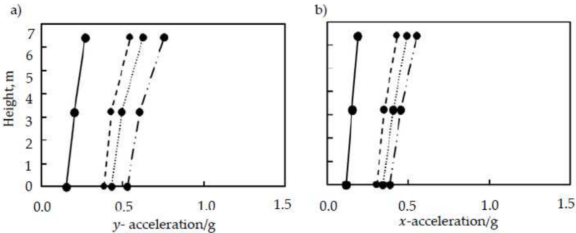
Figure 9. Un-reinforced prototype: a) y -acceleration profile, b) x -acceleration profile.
