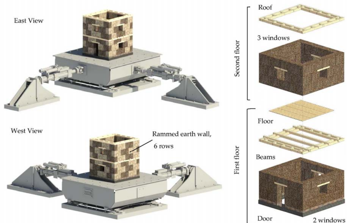
Figure 3. Two story scaled 1:4 earthen house tested.
