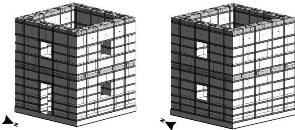
Figure 4. Reinforced 1:4 model with steel plates.
