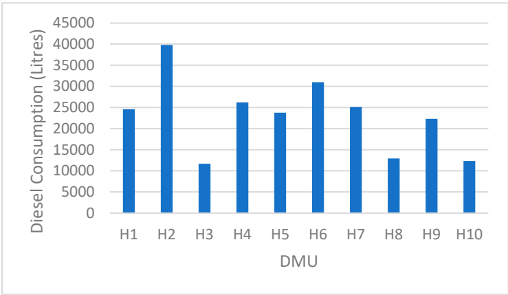
Figure 2. Annual Diesel Consumption of the DMUs.
