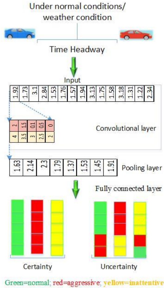
Figure 4. Driving behavior Identification.
