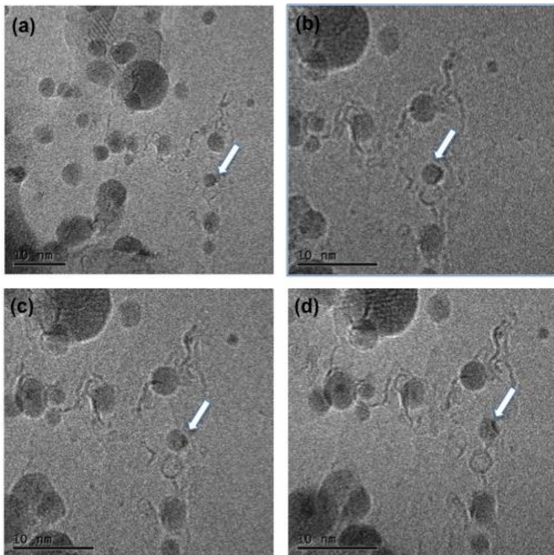
Figure 4. (a-d) Formation mechanism of CN@HDS on the step edges of few layer boron nitride sheets, it can also be seen the escape of FeNP from the CN@HDS.
