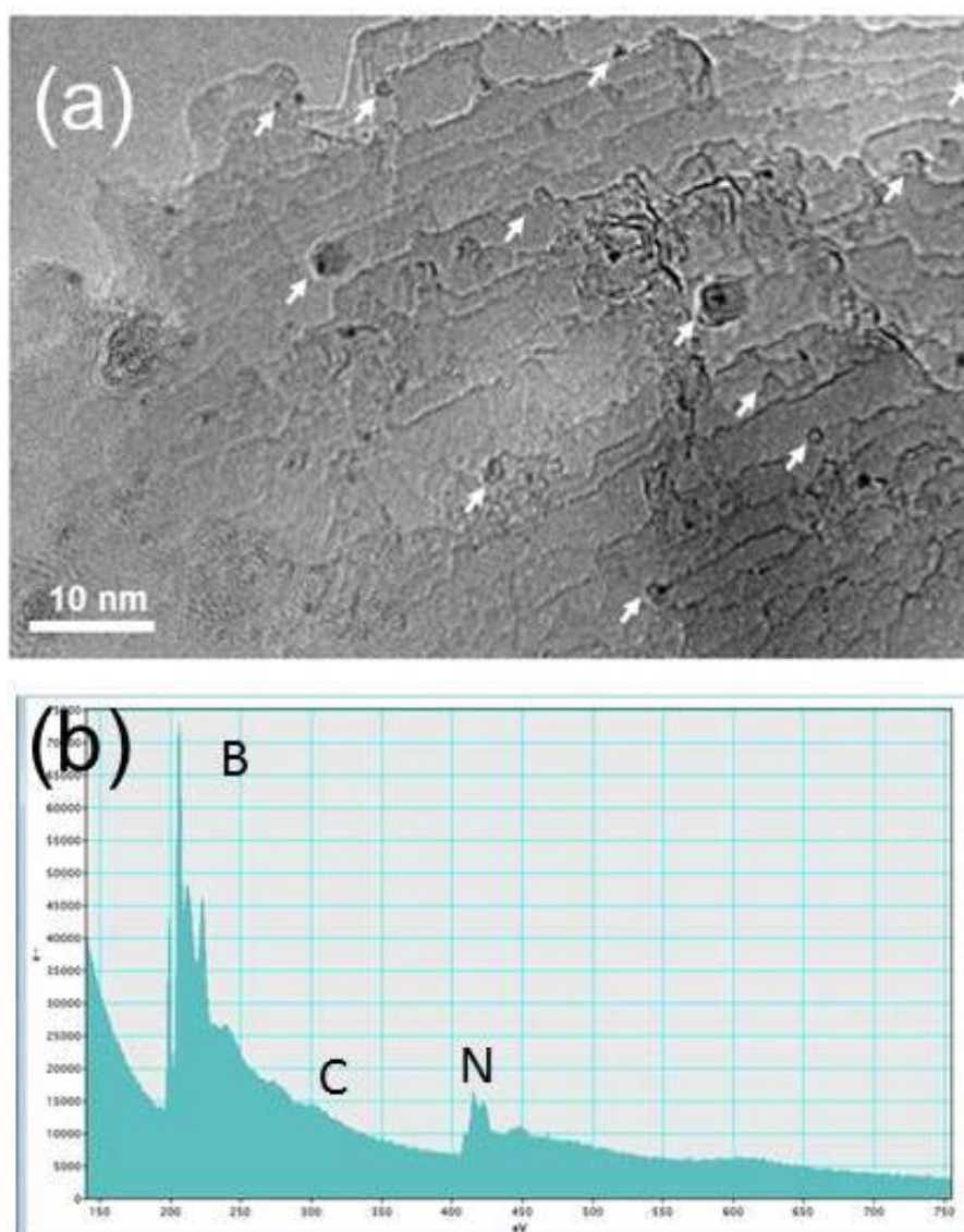
Figure 2. (a) Bright field TEM image showing the CN@HDS residing on the step edges on FLBN – image acquired at 850 °C, at c.a. 30 minutes of in situ heating in vacuum; (b) corresponding EELS of the half dome structure clearly shows the presence of the carbon peak at 284,5 eV which is weak compared to a pure carbon material, and the K-edge at 292 eV. Arrows denote CN@HDS, some of which are decorated with few atoms Fe cluster. The escape of the metal catalyst from CN@HDS is shown in real time on figure 4 and video file 2.
