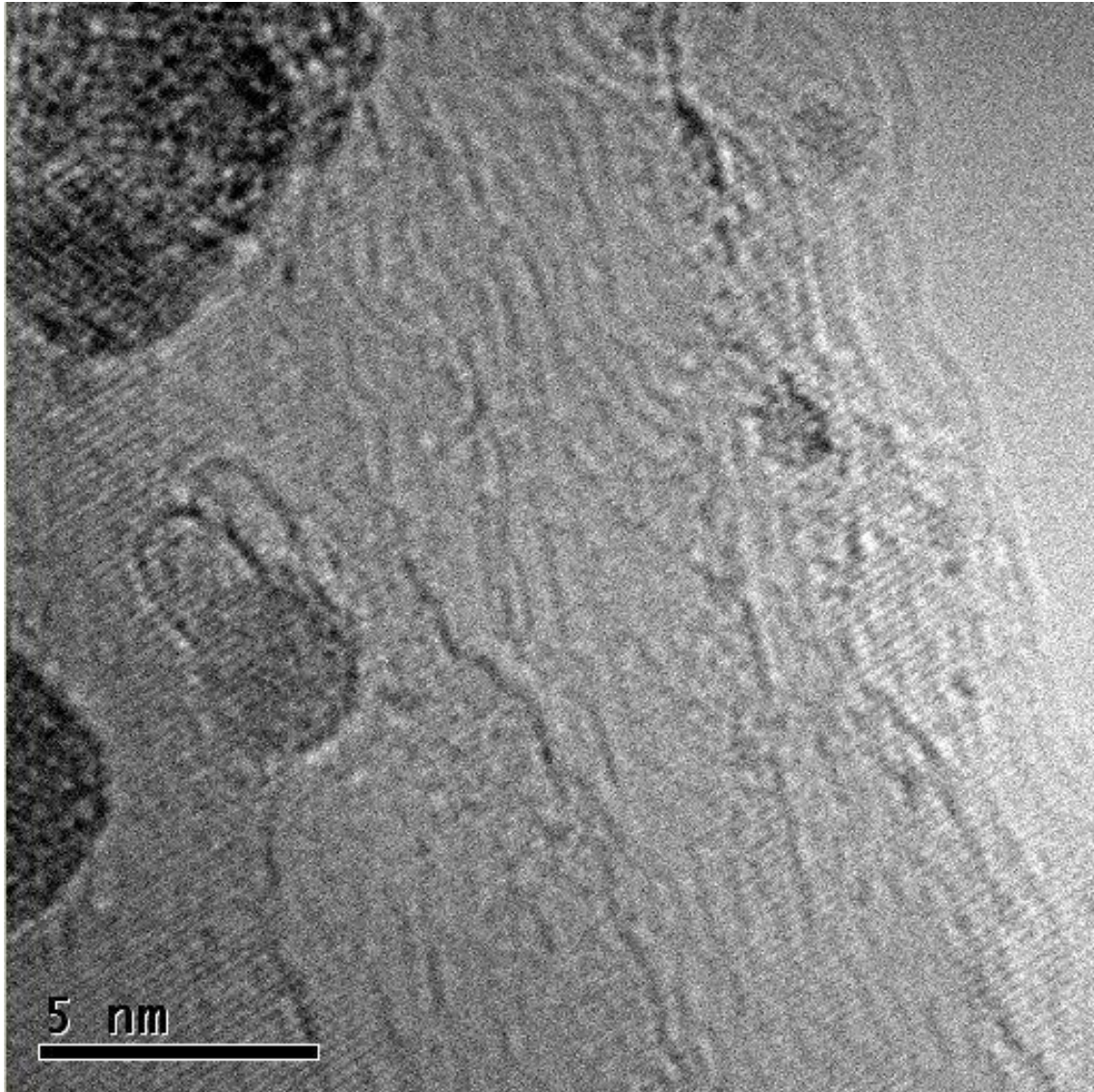
Figure 1. (a) Carbon nitride half dome structure CN@HDS protruding the iron particles (small particle, video file 1),.
