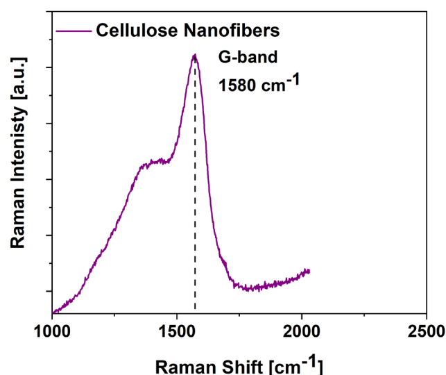
Figure 2. Raman spectrum of carbonized patterns created onto cellulose nanofibers thanks to the implementation of CO 2 laser writing.
