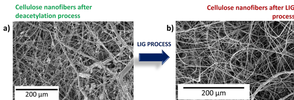
Figure 1. a) Morphological properties of cellulose nanofibers after deacetylation process, confirming the presence of NaOH salts onto nanofibers mats; b) the preservation of nanostructures also after the LIG process involved to create carbonized patterns onto nanofiber mats.
