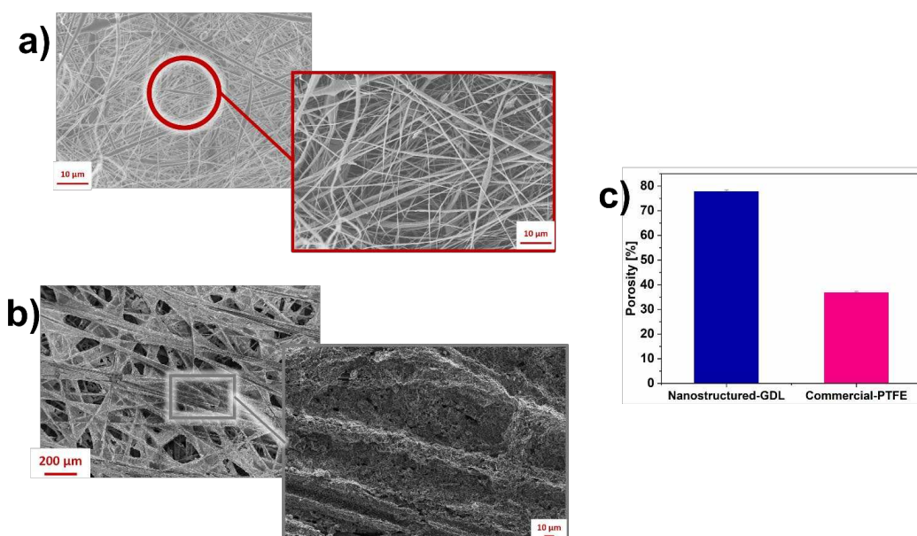
Figure 3. a) Morphological properties of nano-GDL, confirming high porosity of samples, as highlighted from higher magnification, underlined by red box; b) Morphological properties of commercial-PTFE; c) Evaluation of porosity distribution of nano-GDL compared with the one reached with commercial-PTFE.
