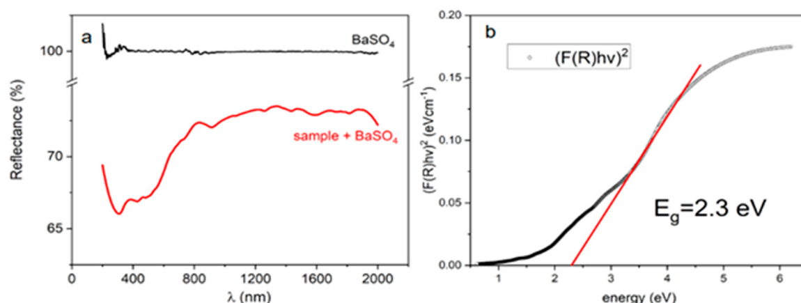
Figure 9. Diffuse reflectance spectrum of the InVO 4 single crystal (a) and Kubelka-Munk transformation for the direct band-gap [(F(R) \cdot hv)^2] (b).
