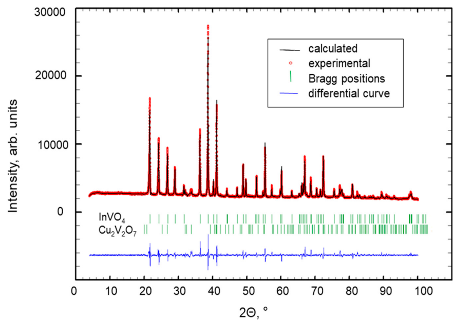
Figure 4. Powder XRD pattern for crushed InVO 4 crystals. The position of Bragg peaks for InVO 4 , for Cu 2 V 2 O 7 are indicated in green, the difference between calculated (black line) and experimental (red dots) intensities is represented in blue.
