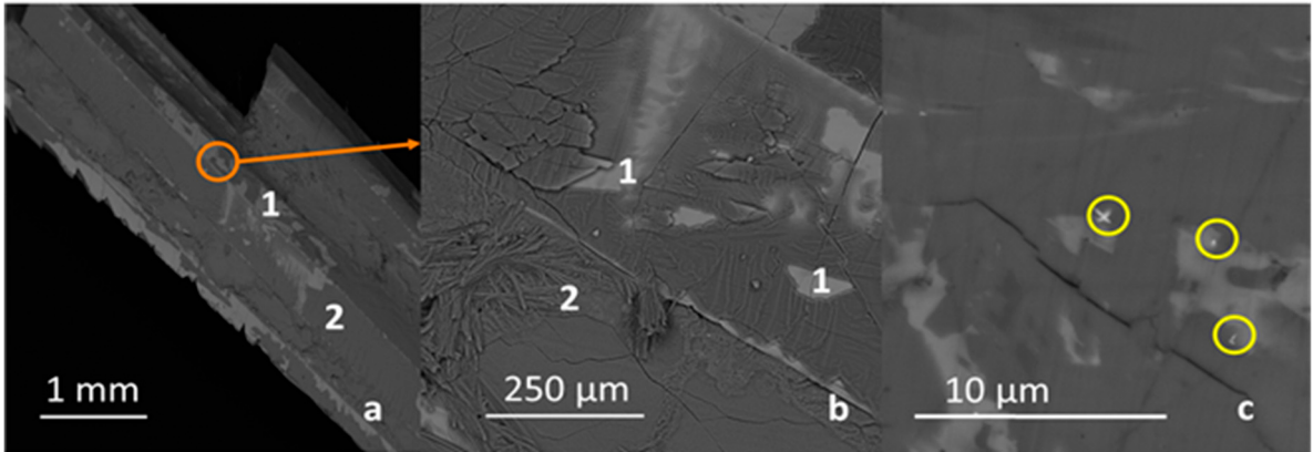
Figure 5. BSEM image of a typical \text{InVO}_4 crystal (a) and of crystal surface (b). Here 1– \text{InVO}_4 and 2– \text{Cu}_2\text{V}_2\text{O}_7 . (c) SEM image of the crystal surface. Tiny inclusions of Pt are highlighted by yellow circles.
