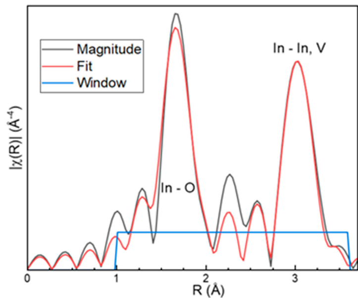
Figure 8. Part of the Fourier-transformed In K-edge EXAFS function of InVO 4 single crystal together with the same function based on the crystallographic model.
