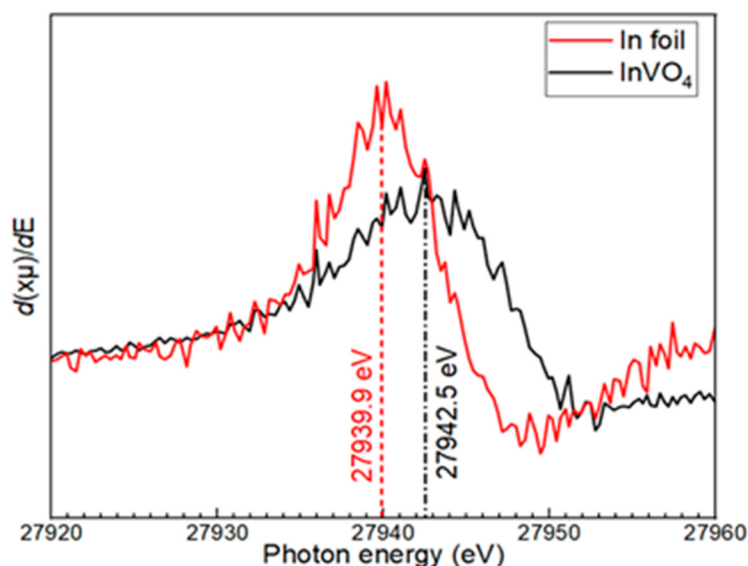
Figure 7. First derivative of In K-edge region of X-ray absorption spectra for InVO 4 and In foil.
