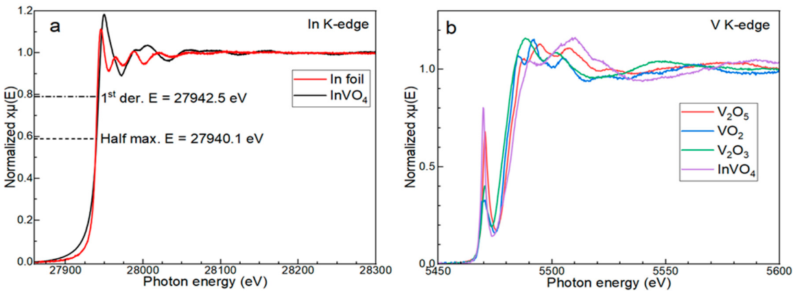
Figure 6. Normalized absorption of \text{InVO}_4 single crystal in (a) In and (b) V K-edge regions.
