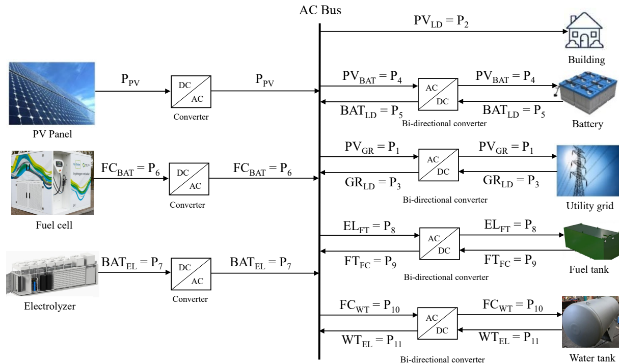
Figure 3. Hybrid MG Structure.
