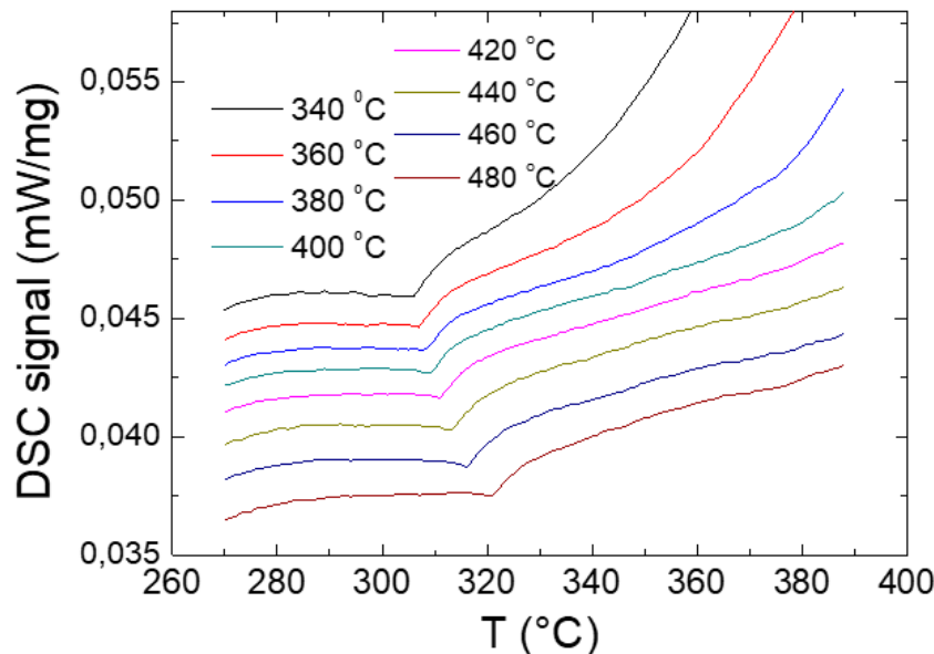
Figure 3. Examples of a DSC curves in vicinity of T_c and their variation with annealing measured in \text{Fe}_{73.8}\text{Cu}_1\text{Nb}_{3.1}\text{Si}_{13}\text{B}_{9.1} microwire.
