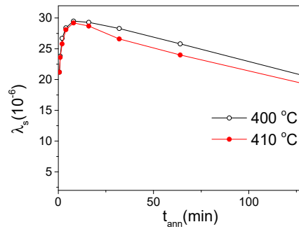
Figure 8. Effect of annealing conditions on magnetostriction, \lambda_s of \text{Fe}_{47}\text{Ni}_{27}\text{Si}_{11}\text{B}_{13}\text{C}_2 microwire.
