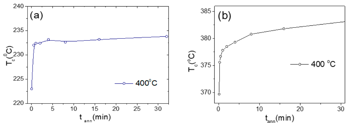
Figure 10. Effect of annealing conditions on T_c of Co_{67}Fe_{3.9}Ni_{1.5}B_{11.5}Si_{14.5}Mo_{1.6} (a) and Fe_{47}Ni_{27}Si_{11}B_{13}C_2 (b) microwires.
