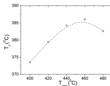
Figure 11. Effect of annealing temperature on T_c of Fe_{47}Ni_{27}Si_{11}B_{13}C_2 microwires.
