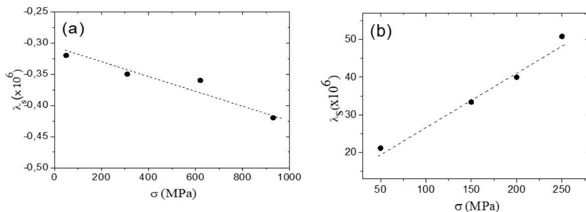
Figure 12. \lambda_s(\sigma) dependence measured in \text{Co}_{67}\text{Fe}_{3.9}\text{Ni}_{1.5}\text{B}_{11.5}\text{Si}_{14.5}\text{Mo}_{1.6} sample (a) and in \text{Fe}_{47}\text{Ni}_{27}\text{Si}_{11}\text{B}_{13}\text{C}_2 sample (b).
