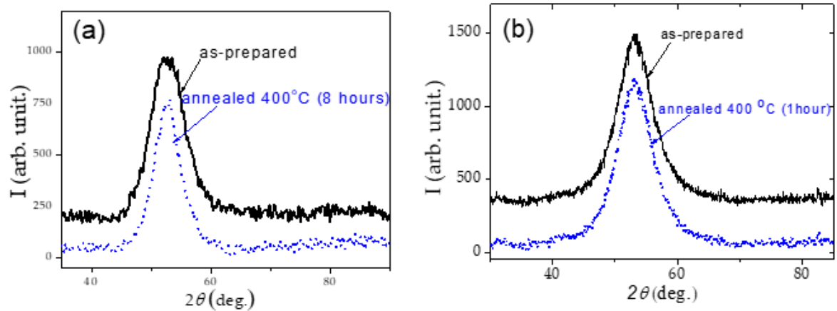
Figure 2. XRD patterns of as-prepared and annealed at 400 °C \text{Fe}_{47}\text{Ni}_{27}\text{Si}_{11}\text{B}_{13}\text{C}_2 (a) and \text{Co}_{67}\text{Fe}_{3.9}\text{Ni}_{1.5}\text{B}_{11.5}\text{Si}_{14.5}\text{Mo}_{1.6} samples (b).
