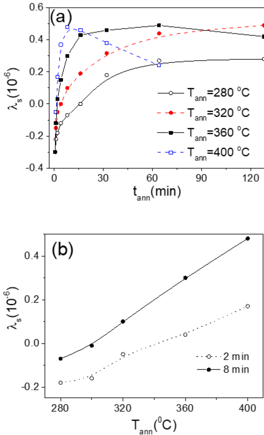
Figure 9. Effect of annealing conditions on magnetostriction, \lambda_s , in \text{Co}_{67}\text{Fe}_{3.9}\text{Ni}_{1.5}\text{B}_{11.5}\text{Si}_{14.5}\text{Mo}_{1.6} microwire: \lambda_s(t_{\text{ann}}) dependencies at different T_{\text{ann}} (a) and \lambda_s(T_{\text{ann}}) dependencies at t_{\text{ann}} = 2 and 8 min (b).
