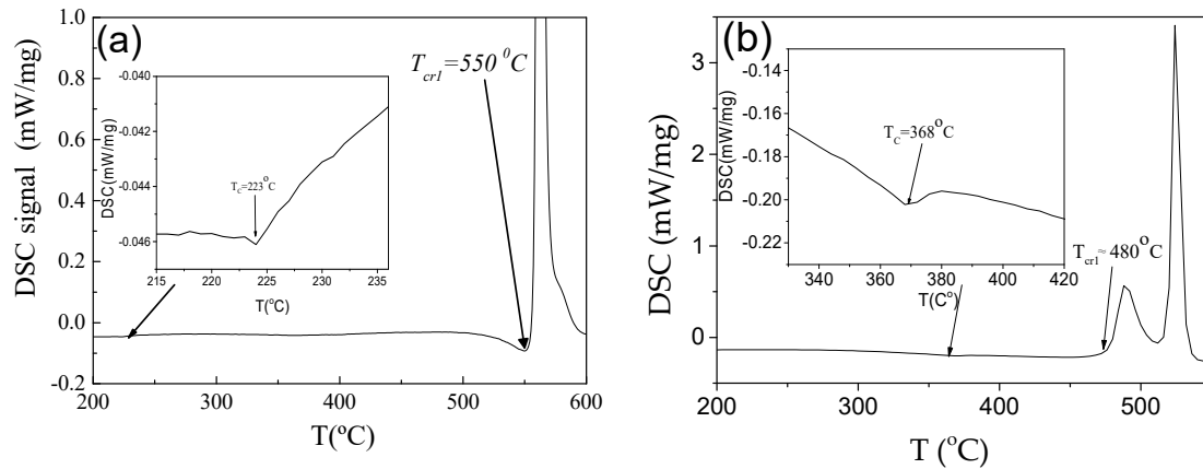
Figure 5. DSC curves of \text{Co}_{67}\text{Fe}_{3.9}\text{Ni}_{1.5}\text{B}_{11.5}\text{Si}_{14.5}\text{Mo}_{1.6} (a) and \text{Fe}_{47}\text{Ni}_{27}\text{Si}_{11}\text{B}_{13}\text{C}_2 (b) samples.
