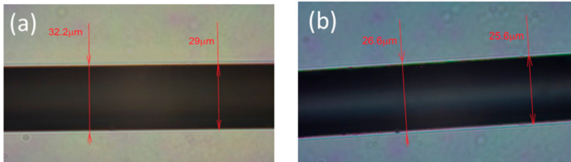
Figure 1. Optical microscopy images of \text{Fe}_{47}\text{Ni}_{27}\text{Si}_{11}\text{B}_{13}\text{C}_2 (a) and \text{Co}_{67}\text{Fe}_{3.9}\text{Ni}_{1.5}\text{B}_{11.5}\text{Si}_{14.5}\text{Mo}_{1.6} (b) samples.
