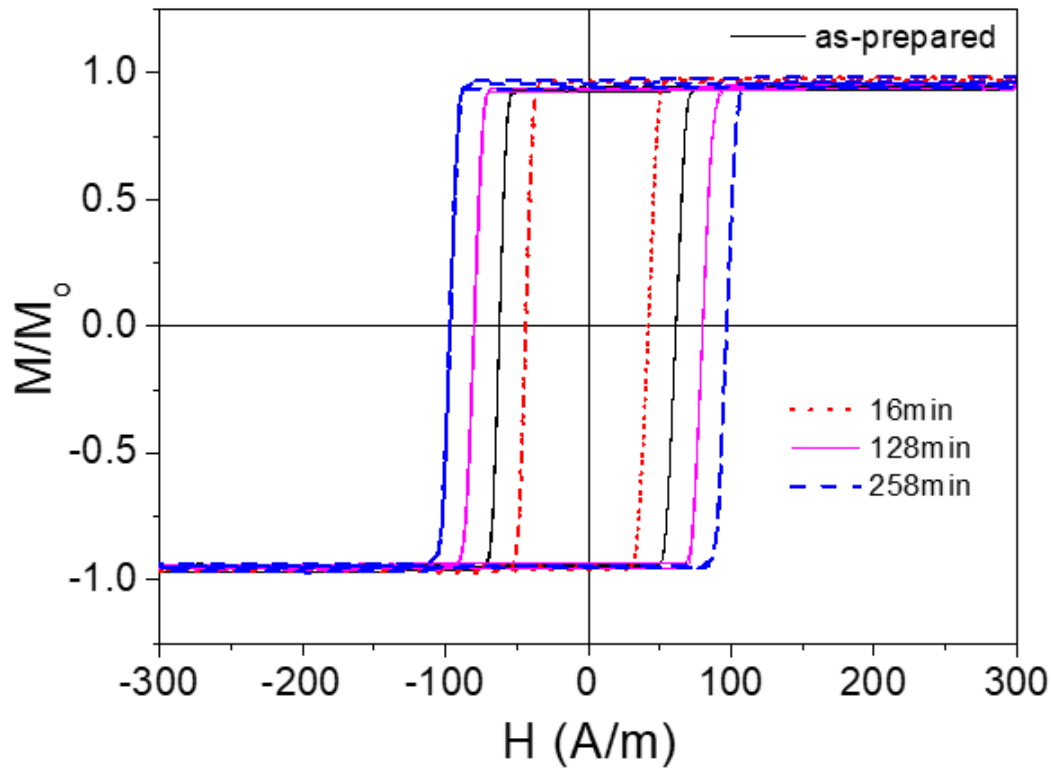
Figure 6. Hysteresis loops measured in as-prepared \text{Fe}_{47}\text{Ni}_{27}\text{Si}_{11}\text{B}_{13}\text{C}_2 microwires and annealed at 410^\circ\text{C} for different time.
