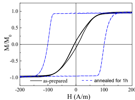
Figure 7. Change of the hysteresis loops of \text{Co}_{67}\text{Fe}_{3.9}\text{Ni}_{1.5}\text{B}_{11.5}\text{Si}_{14.5}\text{Mo}_{1.6} sample after annealing at 400^\circ\text{C} .
