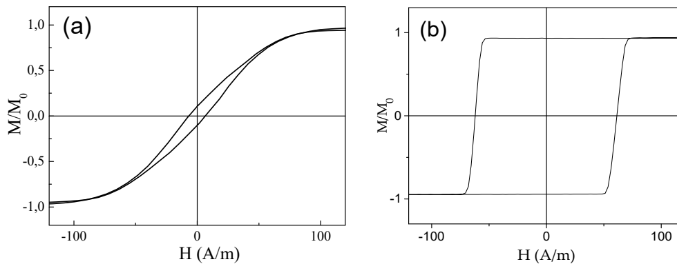
Figure 4. Hysteresis loops of \text{Co}_{67}\text{Fe}_{3.9}\text{Ni}_{1.5}\text{B}_{11.5}\text{Si}_{14.5}\text{Mo}_{1.6} (a) and \text{Fe}_{47}\text{Ni}_{27}\text{Si}_{11}\text{B}_{13}\text{C}_2 (b) samples.
