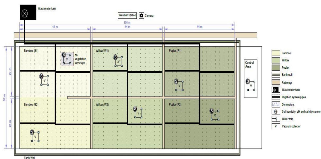
Figure 2. Design of the pilot wfSRC system at the AMU facilities in Aligarh
