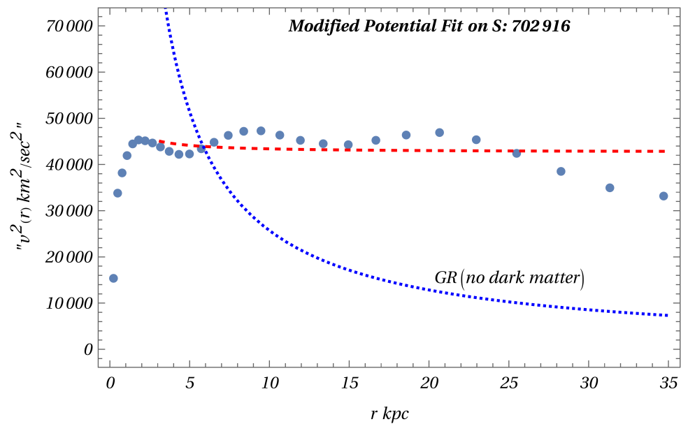
Figure 3. The best-fit form of the velocity profile Eq.(10) for S:702916. The red dashed curve is for the modified potential Eq.(5) obtained from our model. The plot obtained from GR is obviously poor.
