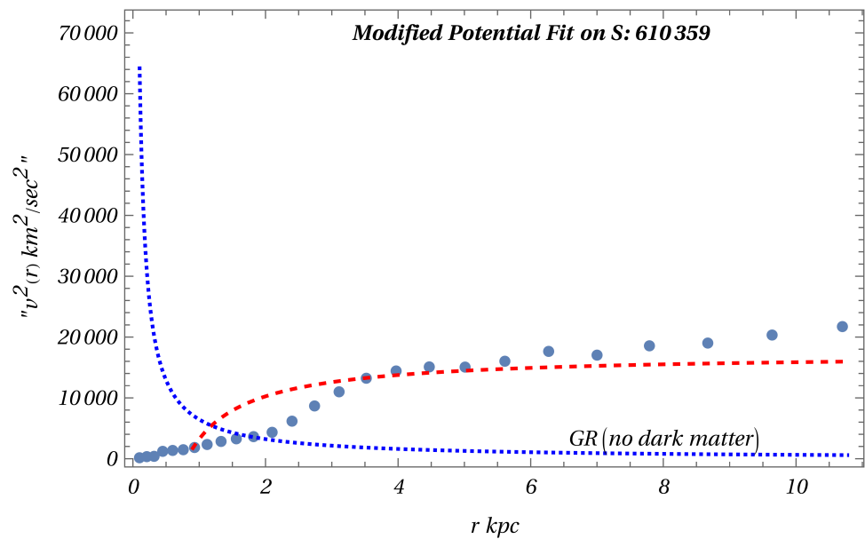
Figure 2. The best-fit form of the velocity profile Eq.(10) for S:610359. The red dashed curve is for the modified potential Eq.(5) obtained from our model. The plot obtained from GR is obviously poor.
