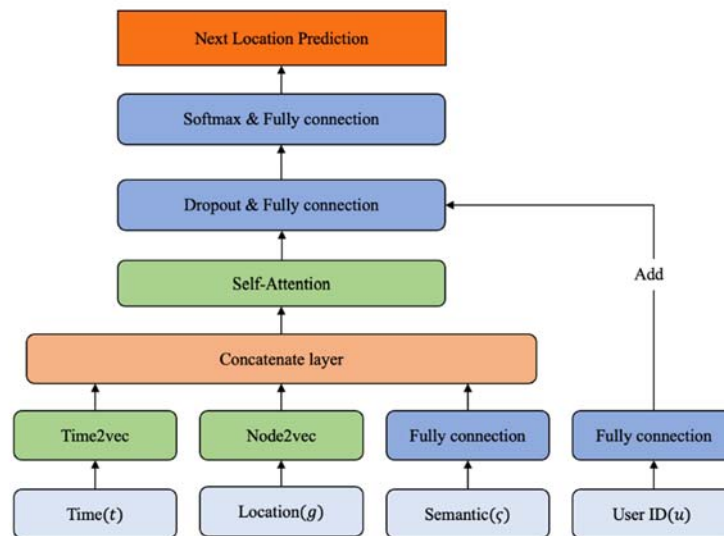
Figure 7. The proposed model.
