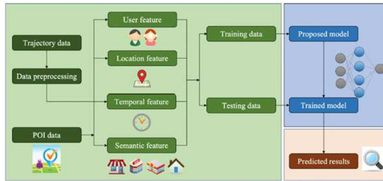
Figure 1. The framework of our research. Source: Icon made by Smashicons, Freepik, & dDara from www.flaticon.com.
