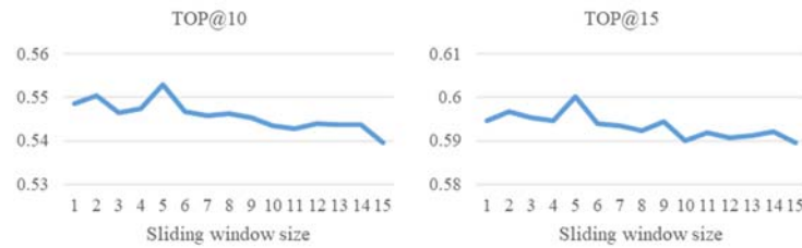
Figure 12. The comparison between different sliding window settings (without the time window).
