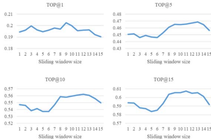
Figure 13. The comparison between different sliding window settings (have the time window).
