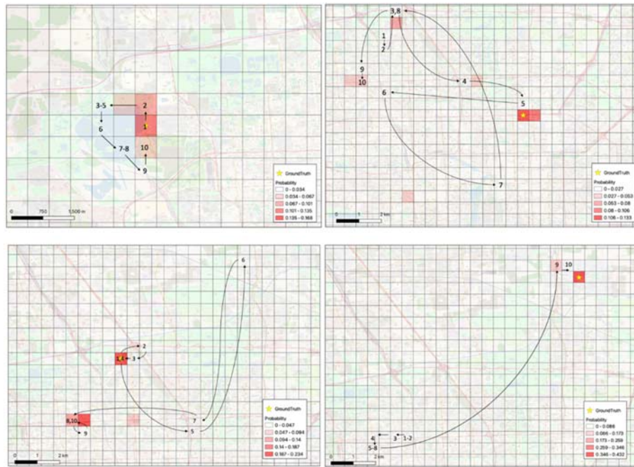
Figure 15. Location prediction visualization examples.
