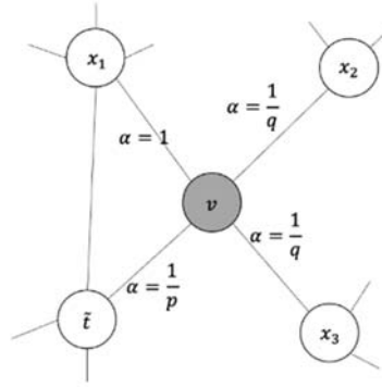
Figure 8. Random walk strategy Error! Reference source not found..
