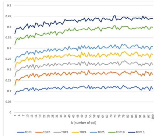
Figure 14. The comparison between different number of k (POI).
