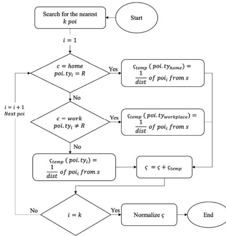
Figure 5. Semantic matching algorithm.
