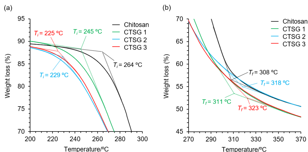
Figure S1. (a) Initial ( T_i ) and (b) final ( T_f ) degradation temperatures for the second degradation of chitosan hydrogels (CTSG 1–3) and chitosan determined by thermogravimetric analysis.
