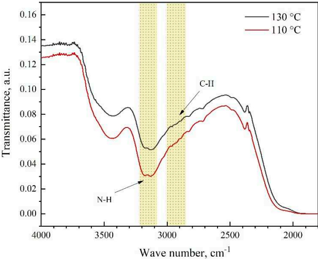
Figure 6. IR transmittance spectra of the CH 3 NH 3 PbI 3 perovskite films after crystallization at an annealing temperature of 110 °C and 130 °C.
