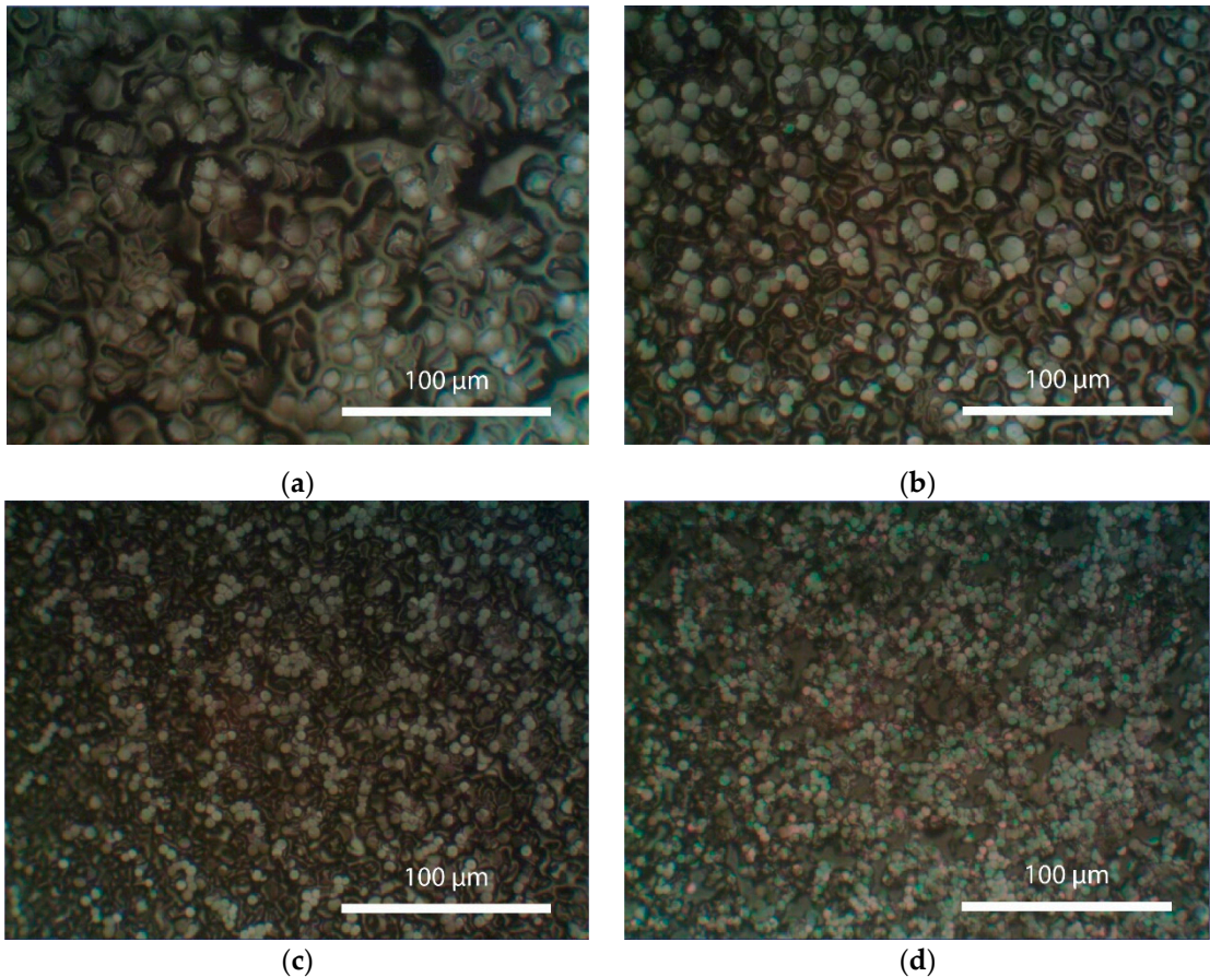
Figure 5. Morphology of perovskite films (pre-annealing at 110 °C) after partial dissolutionof the perovskitesurface in dimethylformamide and subsequent recrystallization in the temperature range of 120 to 150 °C. a - at 120 °C, b - at 130 °C, c - at 140 °C, d - at 150 °C.
