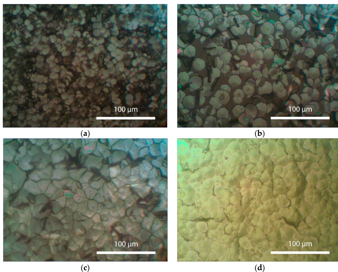
Figure 4. Morphology of perovskite films (pre-annealing at 110 °C) after partial dissolution of the perovskite surface in dimethylformamide and subsequent recrystallization in the temperature range of 80 to 110 °C. a - at 80 °C, b - at 90 °C, c - at 100 °C, d - at 110 °C.
