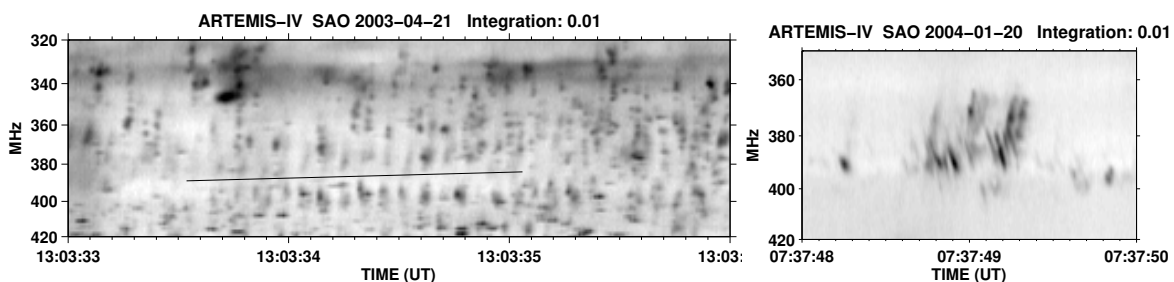
Figure 11. ARTEMIS/SAO high resolution (10 ms) dynamic spectra of drifting narrow-band structures. Left: A group of bi-directional spikes. Above the line there are negative drifting spikes and below are positive drifting spikes. Right: spikes with positive and negative drifts. [From 54, reproduced with permission.].
