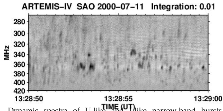
Figure 12. Dynamic spectra of U-like and J-like narrow-band bursts obtained by the ARTEMIS-JLS/SAO at high resolution. [From 54, reproduced with permission.].
