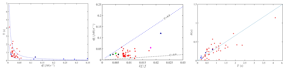
Figure 27. Left: Fiber repetition time plotted against the relative drift rate. The blue lines represent the upper and lower bound of the dimensionless parameter, \zeta , (see text). Typical fibers are shown as red stars, rope-like fibers as blue triangle and the FDBs as blue stars. Middle: Relative drift rate ( df/fdt ) versus relative instantaneous bandwidth ( \delta f/f ). The data points are colour-coded as in the left panel; in addition, the fiber burst points from [153] (magenta diamond), [81] (blue and green diamond), [91,167] (black diamond) are included in the same graph for comparison. The rope-like fibers from [90] are indicated with the black square. The dashed lines are the upper and lower bounds of the slope C = 0.8s^{-1} and C = 8.0s^{-1} . Right Panel: Duration at fixed frequency ( \delta t ) versus repetition time ( T ). The blue dashed line represents the linear relationship (see text). The data points are colour-coded as in the left panel [Adapted from 57].
