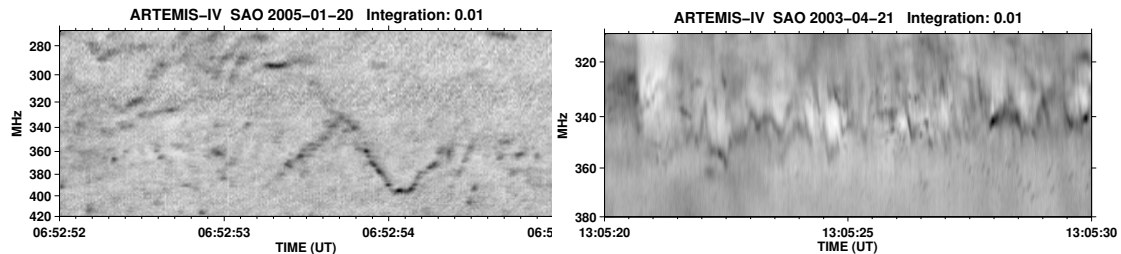
Figure 14. Examples of peculiar spike group recordings obtained by the ARTEMIS-JLS/SAO at high resolution (10ms): Left: "Type III(N)" spike chain. Right: Spike chain forming "Lace like" bands. [From 54, reproduced with permission.].
