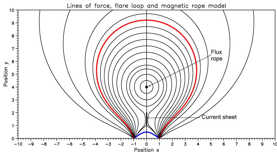
Figure 31. Lines of force of the magnetic field, according to the model of Reeves and Forbes [174]. The blue line marks a flare loop and the red line a large scale loop. The flux rope and the current sheet are marked by the arrows. Positions are in arbitrary units.
