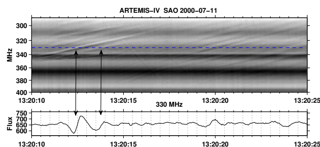
Figure 23. Typical fibers with an emission ridge and an LF absorption ridge. Adapted from [57]
