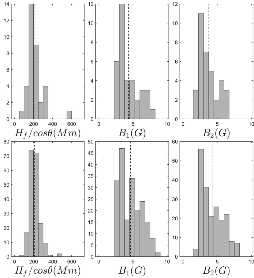
Figure 25. Histograms of fiber parameters derived from the least square fit of the drift rate of fiber groups (top) and the tracks of individual fibers (bottom). H_f/\cos\phi is the frequency scale length along the exciter trajectory and B_1, B_2 the magnetic field at the start and at the end of the fibers [Adapted from 57].
