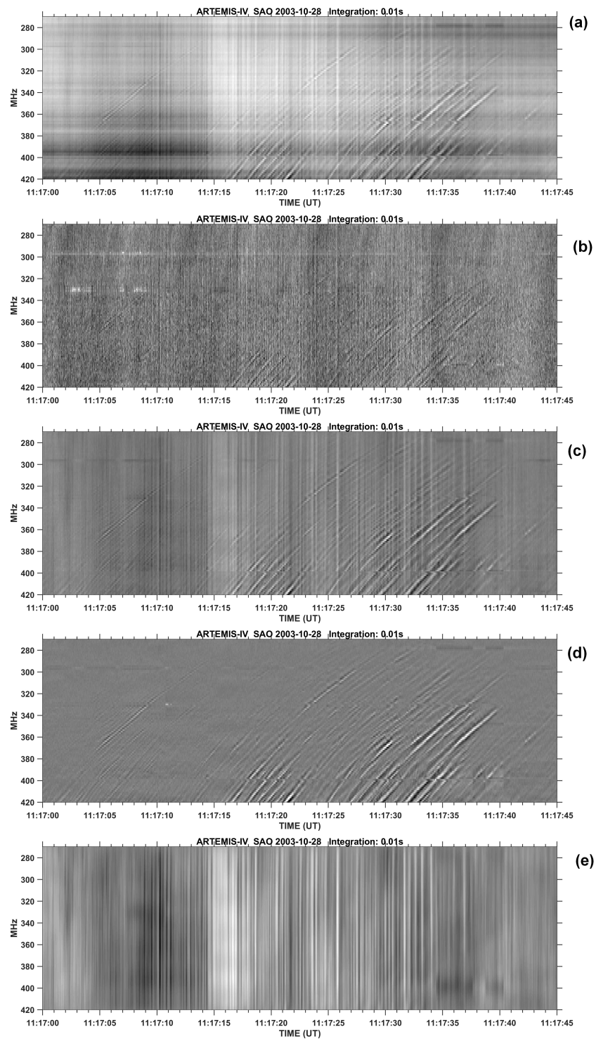
Figure 1. An example of ARTEMIS-IV/JLS/SAO dynamic spectrum at 10 ms resolution, showing fiber bursts overlapping pulsating structure. (a) Original Spectrum. (b) Differential spectrum (Time derivative of Flux). (c) After high pass filtering along the time axis, which suppresses the continuum emission. (d) After an additional high-pass filter along the frequency axis, suppressing broad-band pulsation features. (e) Same as (c), after low-pass filtering along the frequency axis suppressing short time-scale features, fiber bursts in this case.
