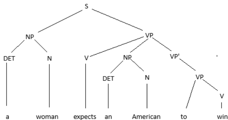
Figure 4. Syntactic tree.
