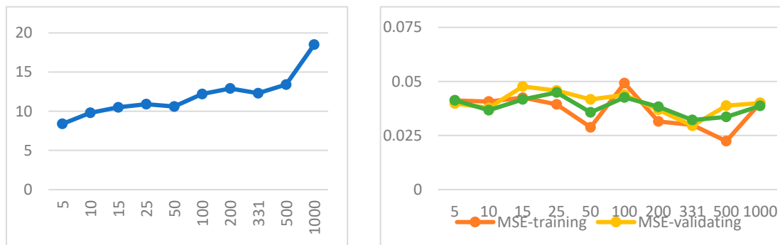
Figure 8. Training time and mean square error of training, validation, and testing for different values of hidden neurons in the simplicity network.
