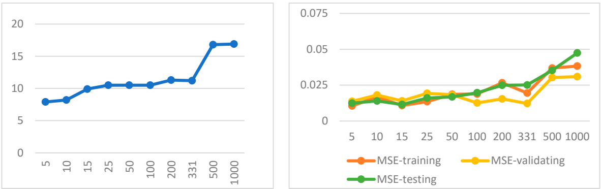
Figure 10. Training time and mean square error of training, validation, and testing for different values of hidden neurons in the practicality network.
