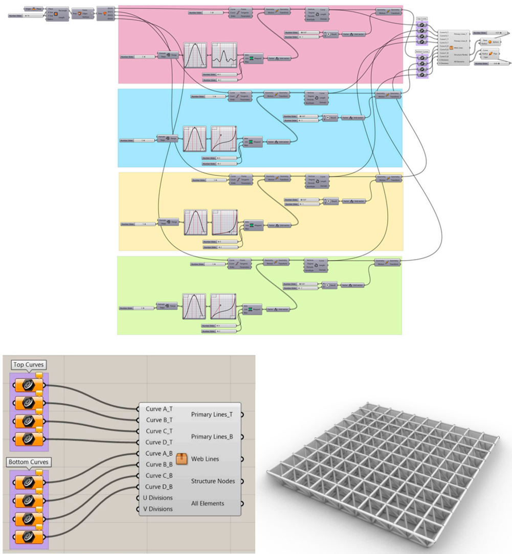
Figure 1. The code for assigning curves to the sides of squares (Left), the basic form, square on square offset grid space structure (Right)
