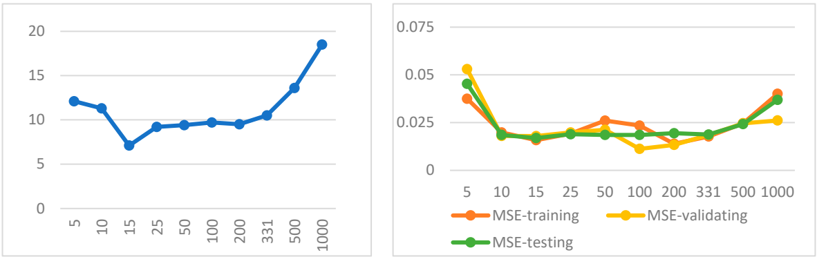
Figure 9. Training time and mean square error of training, validation, and testing for different values of hidden neurons in the complexity network.
