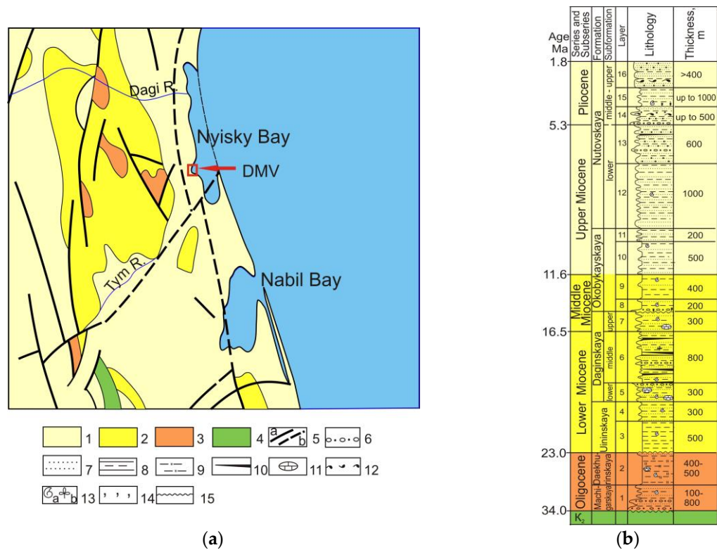
Figure 3. Scheme of geology (a) and stratigraphy (b) of the Dagi area of Eastern Sakhalin [19]. 1 – Upper Miocene–Pliocene; 2 – Lower to Middle Miocene; 3 – Paleogene; 4 – Mesozoic; 5 – faults (a – established, b – assumed); 6 – conglomerates, gravelites; 7 – sandstones; 8 – siltstones, mudstones; 9 – diatomites, including sandy-siltstone-clayey diatomites; 10 – coal beds; 11 – calcareous concretions; 12 – shell lenses; 13 – remains of fauna (a) and flora (b); 14 – glauconite; 15 – erosion. K2 – Upper Cretaceous, DMV – Daginsky Mud Volcano.
