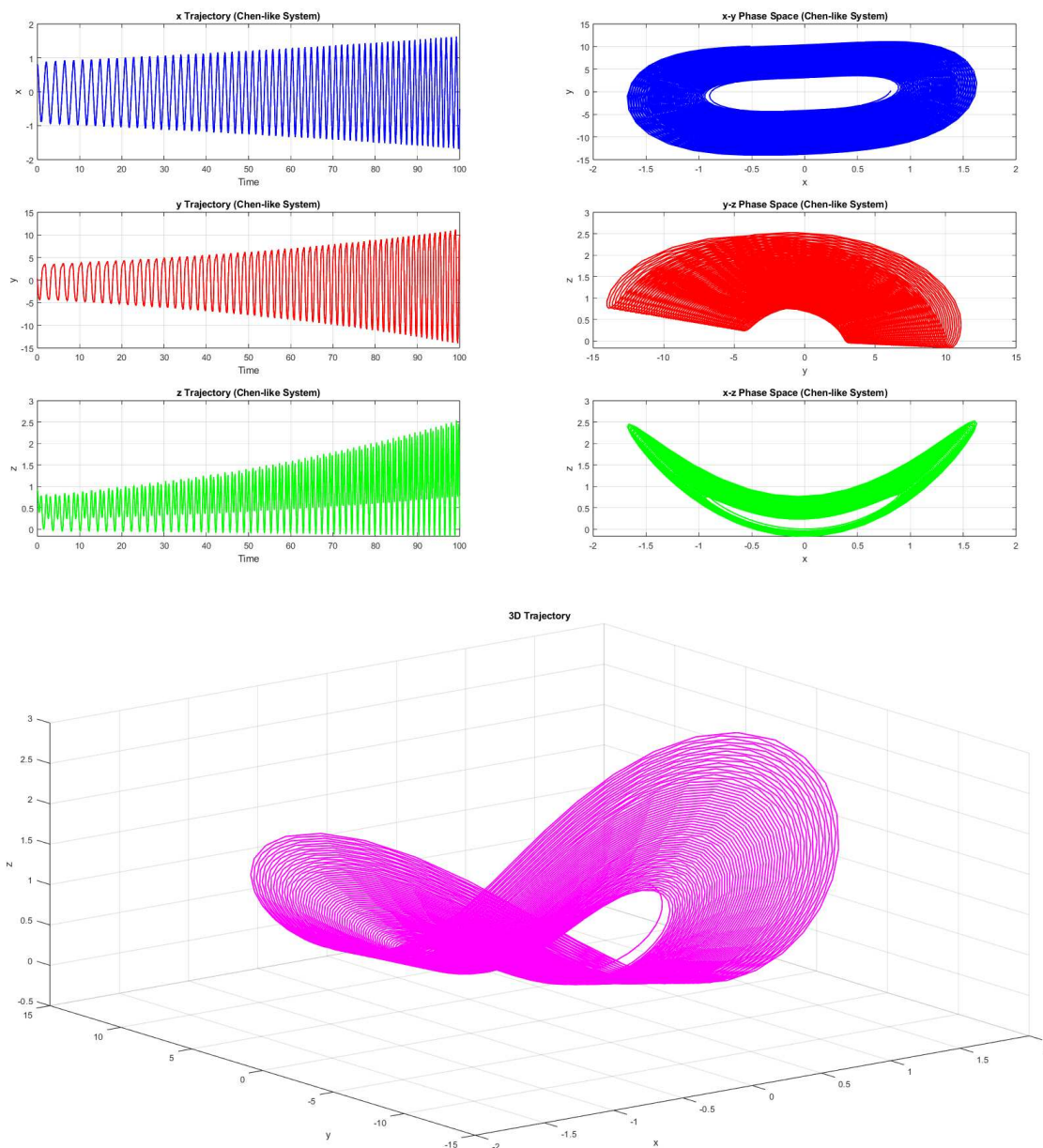
Figure 4. Non-hyperbolic trajectory in 3 dimension and two dimensional phase portraits
