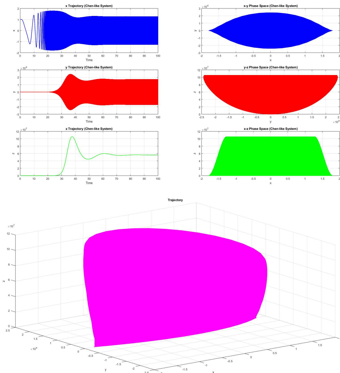
Figure 11. Chaotic trajectories with Lyapunov exponent ( \lambda=0.001220 ) and corresponding two dimensional phase portraits (Parameters: a=0.2575 , b=0.8407 , c=0.2543 , and d=0.8143 )
