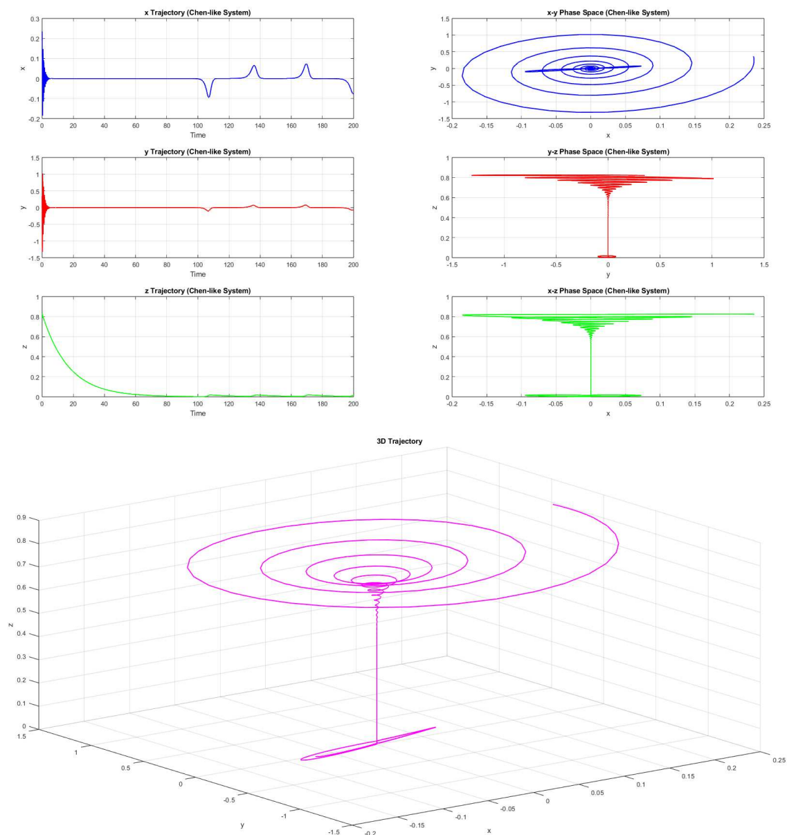
Figure 1. Sink trajectory in 3 dimension and two dimensional phase portraits
