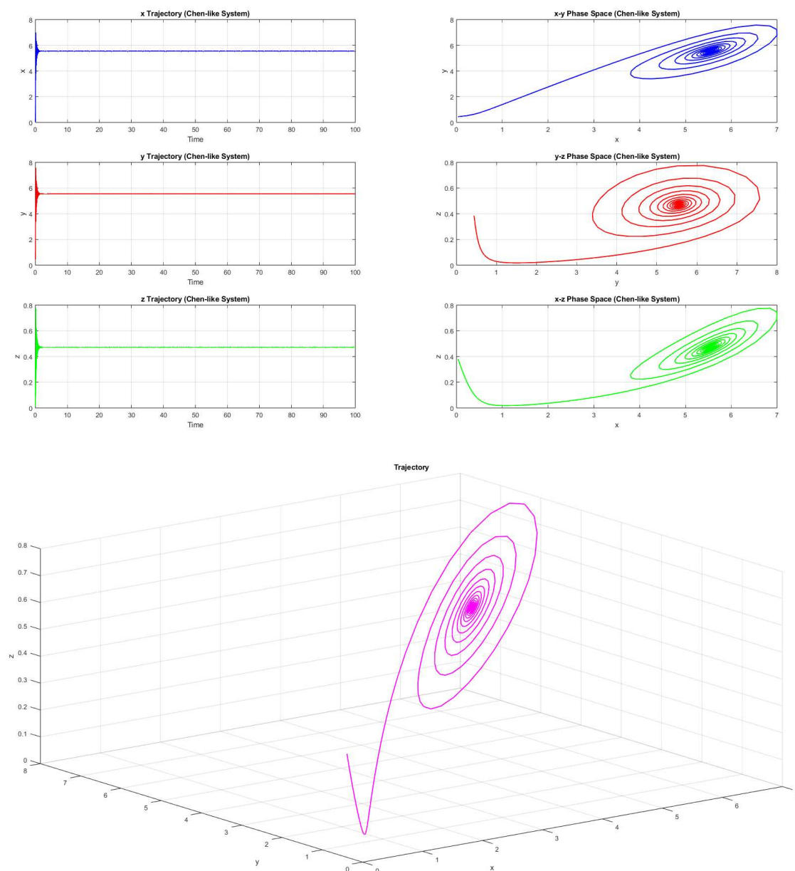
Figure 5. Convergent trajectory in 3-dimension and 2-dimensional phase portraits
