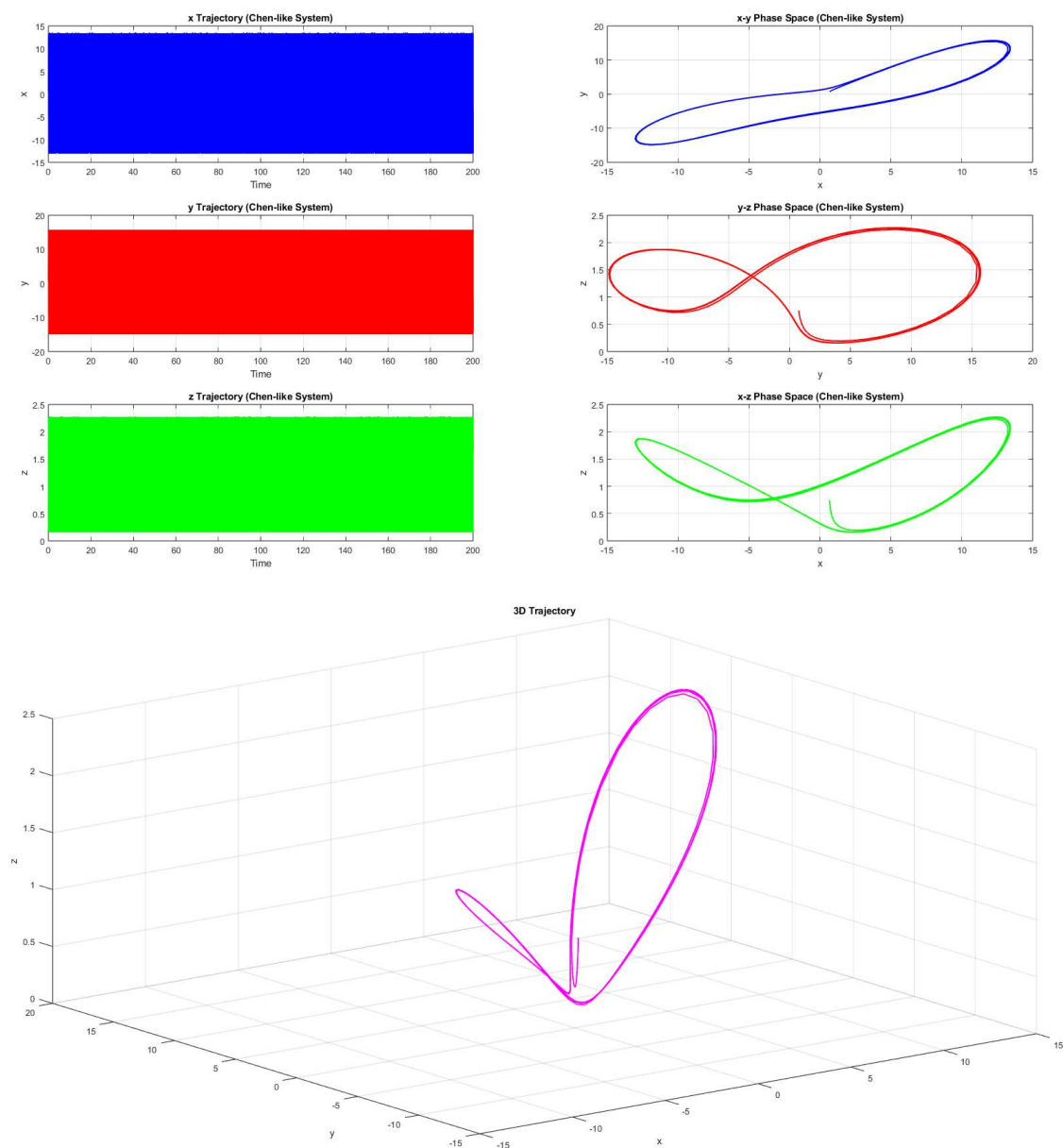
Figure 2. Source trajectory in 3 dimension and two dimensional phase portraits
