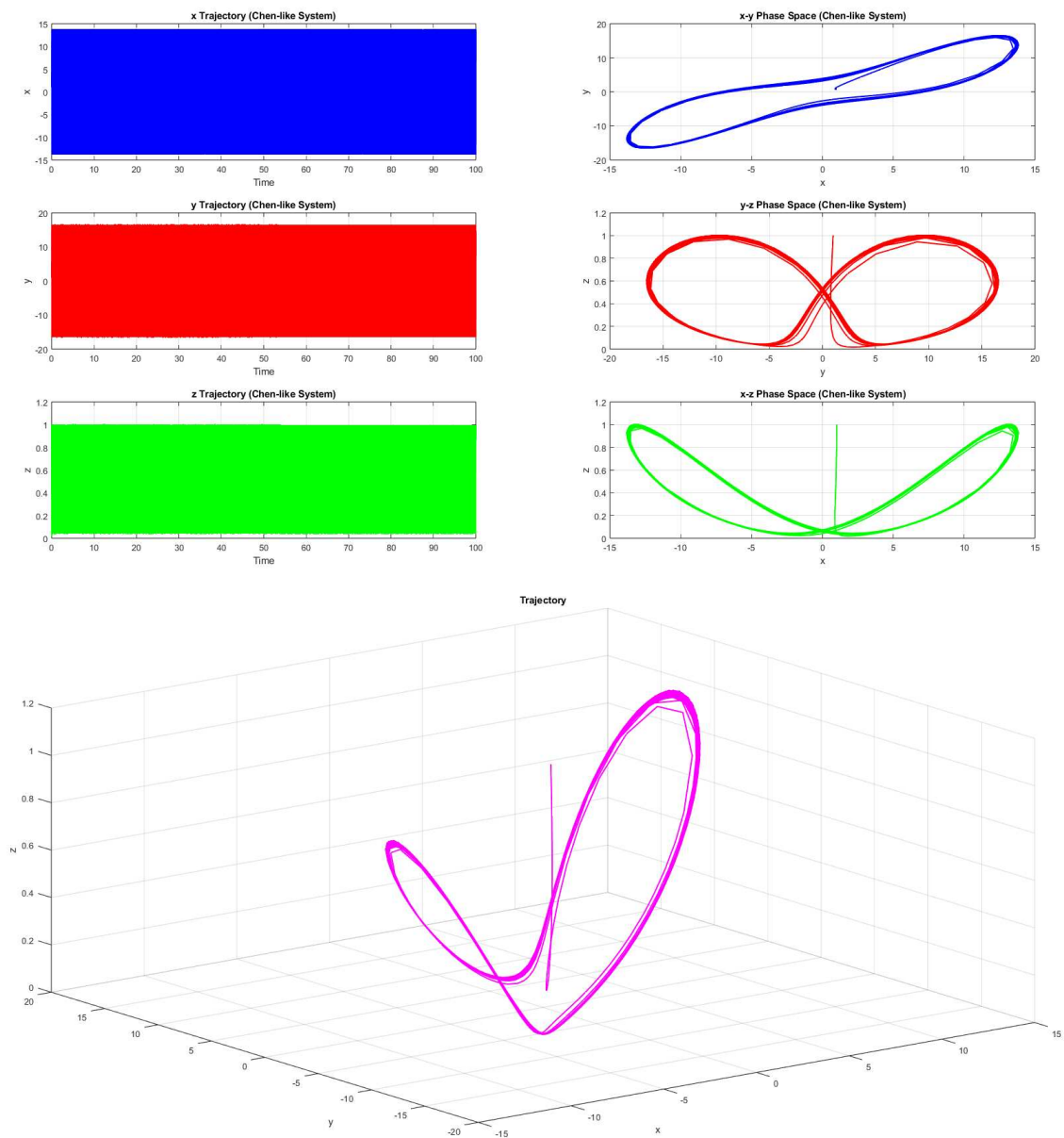
Figure 13. Chaotic trajectories with Lyapunov exponent ( \lambda=0.000088 ) and corresponding two dimensional phase portraits (Parameters: a=205 , b=298 , c=132 , and d=302 )
