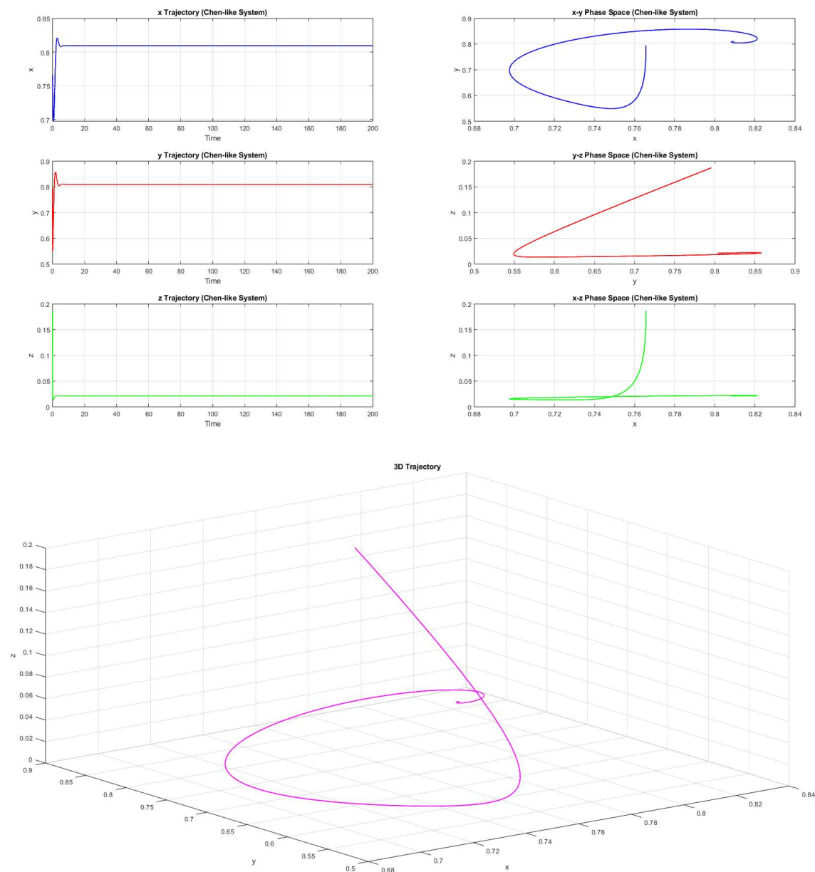
Figure 3. Saddle node trajectory in 3 dimension and two dimensional phase portraits
