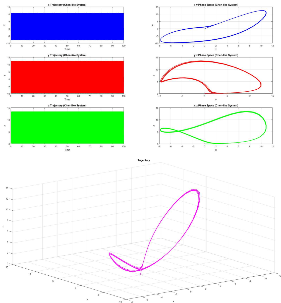
Figure 7. Periodic trajectories with periodicity 69 and corresponding two dimensional phase portraits
