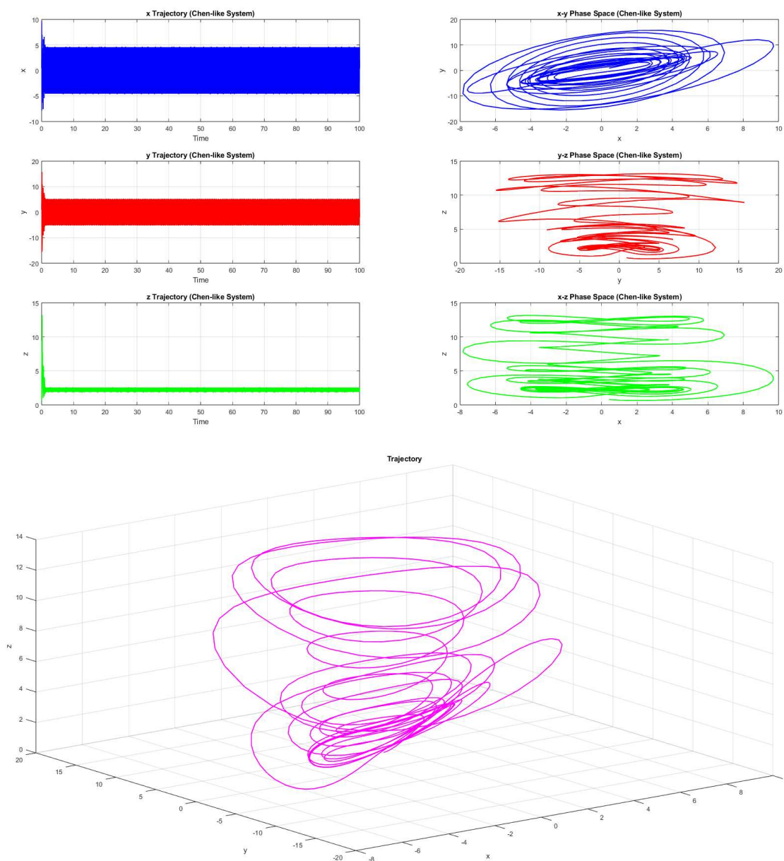
Figure 8. Periodic trajectories with periodicity 425 and corresponding two dimensional phase portraits
