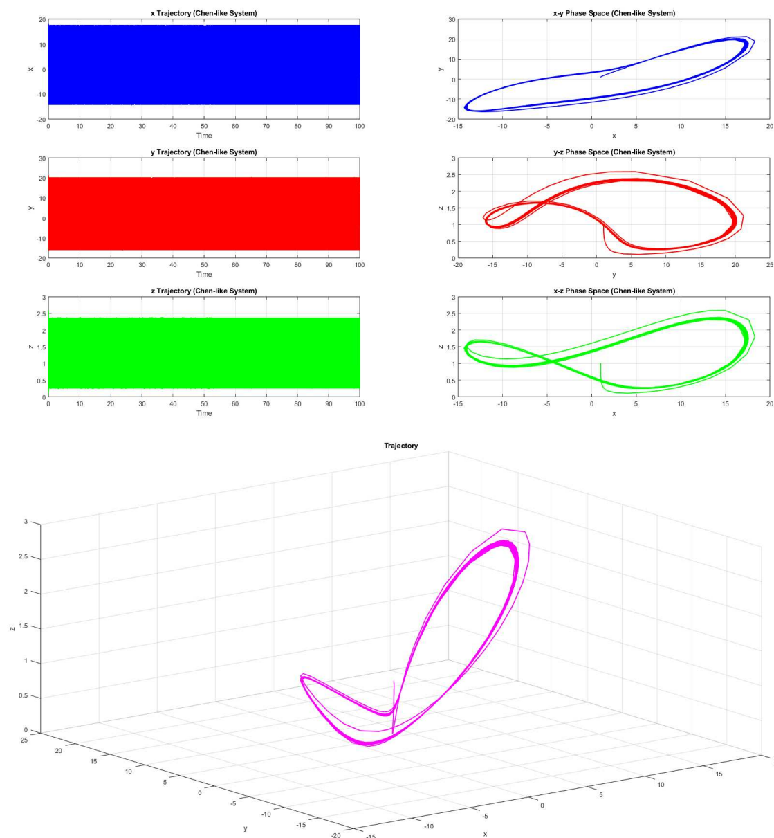
Figure 12. Chaotic trajectories with Lyapunov exponent ( \lambda=0.000094 ) and corresponding two dimensional phase portraits (Parameters: a=388 , b=244 , c=218 , and d=224 )
