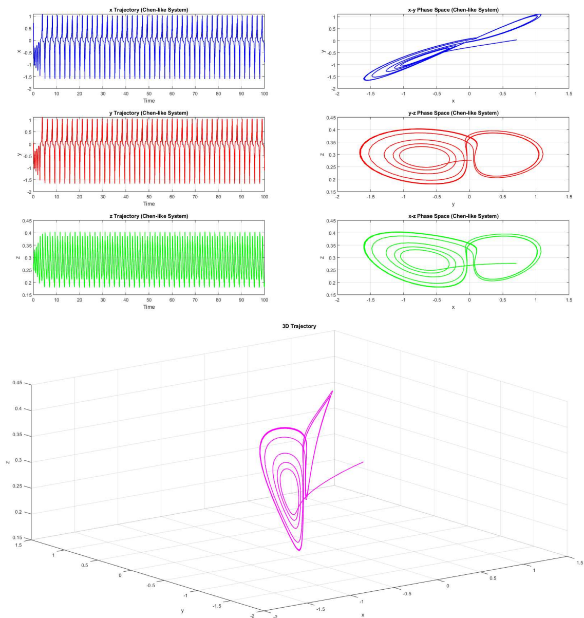
Figure 9. Periodic trajectories with periodicity 689 and corresponding two dimensional phase portraits
