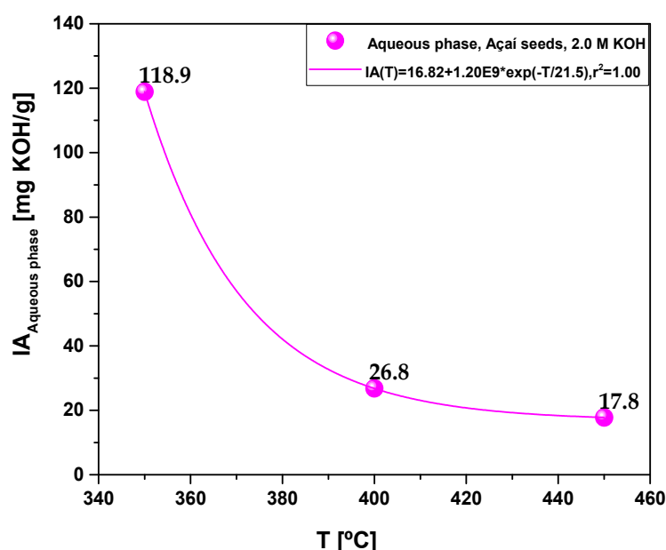
Figure 12. Acidity of aqueous phase obtained by pyrolysis of Açai seeds.
