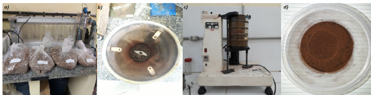
Figure 3. Açai seeds pre-treatment [Dried Açai seeds (a); Knife cutting mill (b); Mechanical sieve shaker (c); Dried, grinded and sieved Açai seeds (d)].
