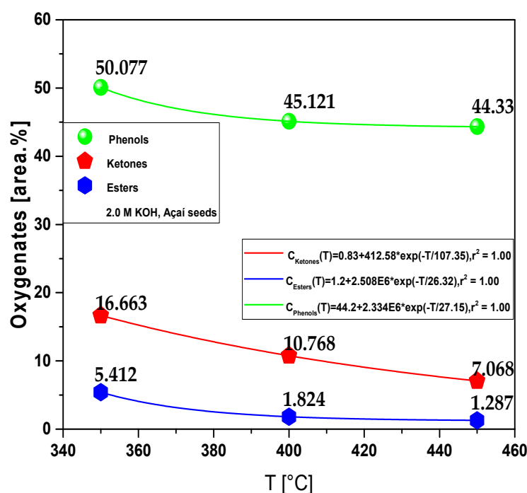
Figure 10. Concentration of oxygenates (phenols, ketones, and esters) in bio-oil by pyrolysis of Açai seeds ( Euterpe Oleracea , Mart), in the temperature range of 350-450 °C.
