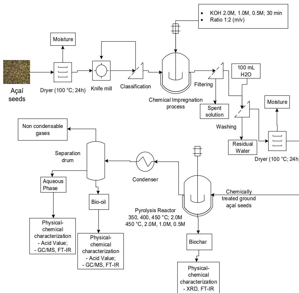
Figure 1. Process flow schema of bio-oil production by pyrolysis of Açai seeds at 350, 400, and 450 °C, 1.0 atm, 2.0 M KOH, and 450 °C, 1.0 atm, 0.5 M, 1.0 M, and 2.0 M KOH, using a fixed bed reactor, in laboratory scale.
