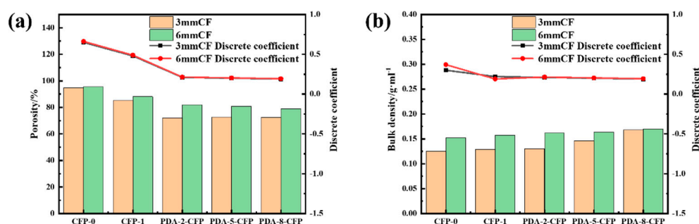
Figure 10. (a). Porosity of different CFPs; and (b) Bulk density of different CFPs.
