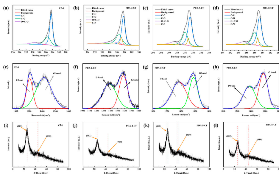
Figure 15. C1s XPS peak fit of CF-1 (a), PDA-2-CF (b), PDA-5-CF (c) and PDA-8-CF (d). Raman spectrum of the CF-1 (e), PDA-2-CF (f), PDA-5-CF (g) and PDA-8-CF (h). (i) XRD pattern of the CF-1 (i), PDA-2-CF (j), PDA-5-CF (k) and PDA-8-CF (l).
