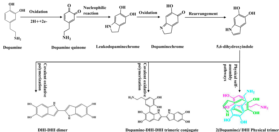
Figure 1. Dopamine oxidation mechanism process.
