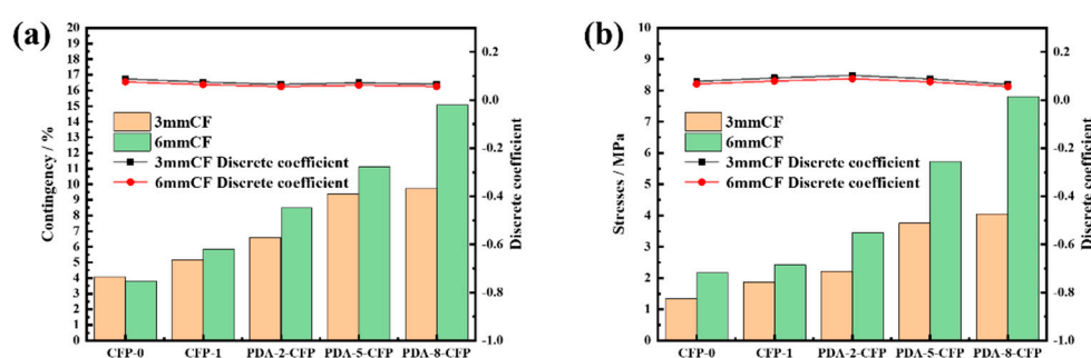
Figure 11. (a) Contingency of different CFP; and (b) Stresses of different CFPs.
