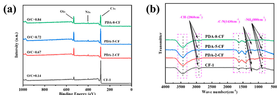
Figure 14. (a) Ratio of O/C contents of CFs after different treatments; and (b) Combined FTIR spectrum of different treated CFs.
