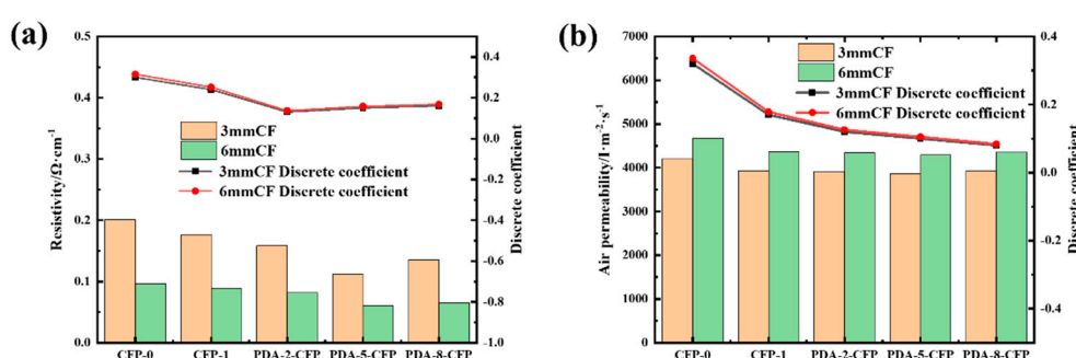
Figure 12. (a) Resistivity of different CFPs; and (b) Air permeability of different CFPs.
