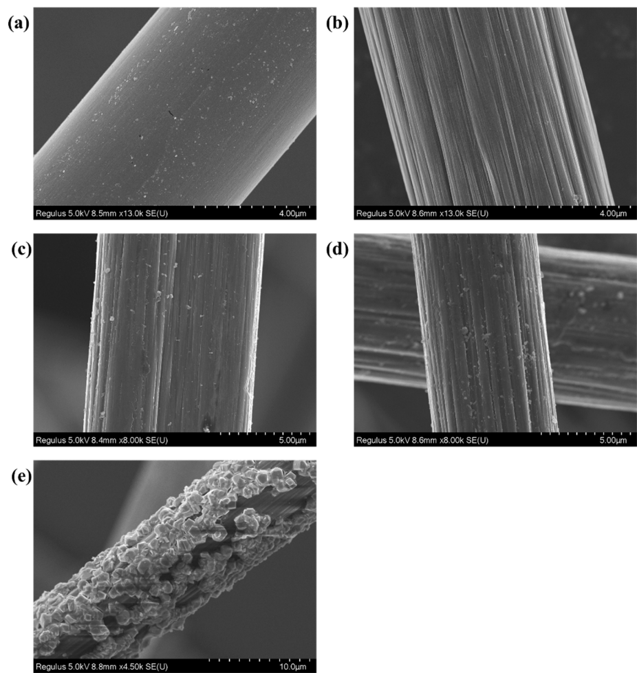
Figure 3. (a) SEM image of the virgin CF (CF-0) surface; (b) SEM image of the CF-1; (c) SEM images of the PDA-2-CF; (d) SEM images of the PDA-5-CF; and (e) SEM images of the PDA-8-CF.
