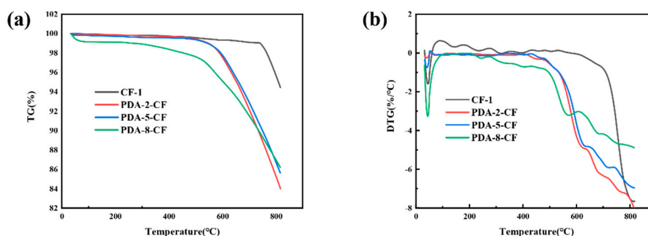
Figure 6. (a) TG curves of CF-1 and PDA-CF; and (b) DTG curves of CF-1 and PDA-CF.
