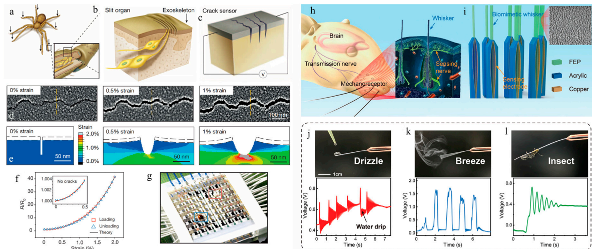
Figure 6. Flexible touch sensors inspired by structures of insects and animals. a-c) Illustrations demonstrating a spider's sensitive organs at its legs for detecting external stresses and vibrations (black arrows). The leg joint between the metatarsal and tarsal bones is the position where the sensory organs are located. d-e) SEM images and Finite-Element modelling results of the zip-like crack under different strains. f) Change in resistance of the sensor under different strains. g) Picture showing a 8×8 array of the crack strain sensor. (Reprinted with permission from Ref. [46], Copyright 2014, Nature) h) Schematic illustration showing a rat's whisker sensory system and the local schematic representation of the whisker mechanoreceptor. i) Schematic representation of the bionic structure of the BWMR. j-l) Response behaviors of BWMR to weak perturbations, such as drizzle (j), breeze (k), and insect crawling (l). (Reprinted with permission from Ref. [94], Copyright 2021, Adv Mater).
