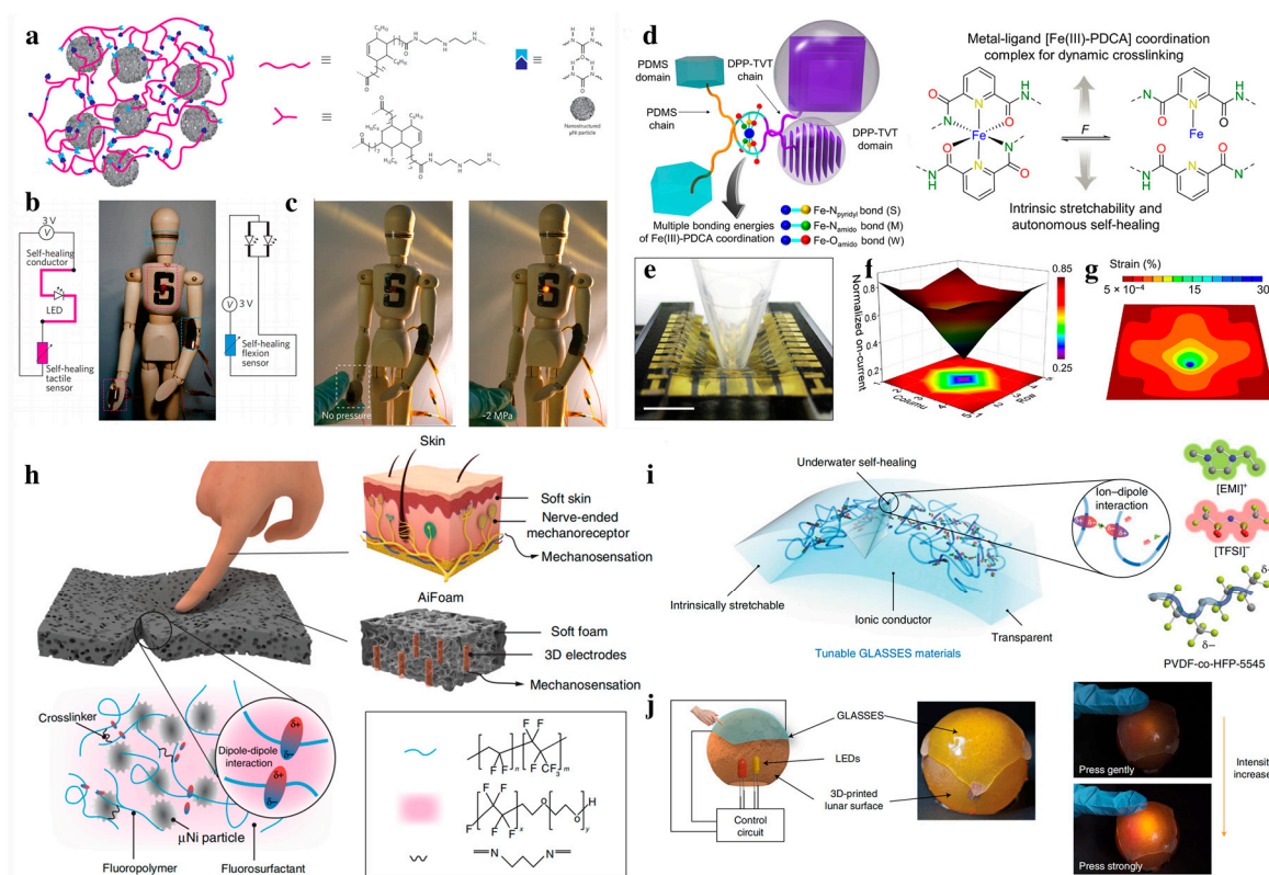
Figure 3. Construction of flexible touch sensors based on self-healing materials. a) Schematic diagram showing the interaction between oligomer chains and the \mu\text{Ni} particles in the developed supramolecular polymers. b) Schematic circuit and picture showing of the touch sensors attached on a wooden mannequin. c) Pictures showing that the LED intensity can be enhanced as tactile pressure increases. (Reprinted with permission from Ref. [65], Copyright 2012, Nat Nanotechnol) d) Schematic demonstrating the Fe(III)-PDCA complexation. e) Photograph showing a plastic rod poking the stretched active-matrix transistor array. f, g) Simulation result of f) Normalized on-current and g) strain distribution by poking the array. (Reprinted with permission from Ref. [66], Copyright 2019, Science) h) Schematic illustration of the AiFoam material created by replicating the somatosensory innervation system of human skin. (Reprinted with permission from Ref. [67], Copyright 2020, Nat
