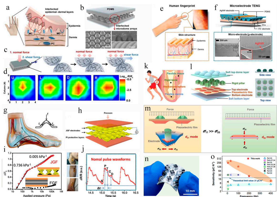
Figure 7. Flexible touch sensors inspired by the structures in human body. a) Schematic of human skin structure with interlocked epidermal-dermal layers. b) Schematic of an interlocked microdome array used for fabricating highly sensitive touch sensor. c) Schematic showing the deformation of the microdomes under stepwise application of normal and shear forces. d) Schematic diagram of the electronic skin for detecting different pressing directions of the finger: left (L), right(R), up(U), down(D). (Reprinted with permission from Ref. [45], Copyright 2014, Acs Nano) e) Picture and schematic illustration of human fingerprints. f) Illustration and SEM images of fingerprint-inspired u-TENGs. (Reprinted with permission from Ref. [39], Copyright 2022, Nano Energy) g) Anatomical model of the human foot with arch structure. h) Structural scheme of the fabricated pressure sensor. i) Sensitivity of JGF-based and FGF-based pressure sensors. j) Characteristic peaks of pulse waveforms measured by the JGF-based pressure sensors. (Reprinted with permission from Ref. [34], Copyright 2018, Advanced Electronic Materials) k) Illustration showing the anatomical structure of the fingers in human body with different compositions. l) Finger-inspired rigid-soft hybrid piezoelectric tactile sensor. m) Deformation modes and working principles of the tactile sensors made from different piezoelectric sensing structures. n) Photograph of a RSHTS array with 3 \times 3 sensing units. o) Comparison in sensitivity of the hybrid piezoelectric tactile sensor with other existing piezoelectric tactile sensors. (Reprinted with permission from Ref. [104], Copyright 2022, Nature Communications).
