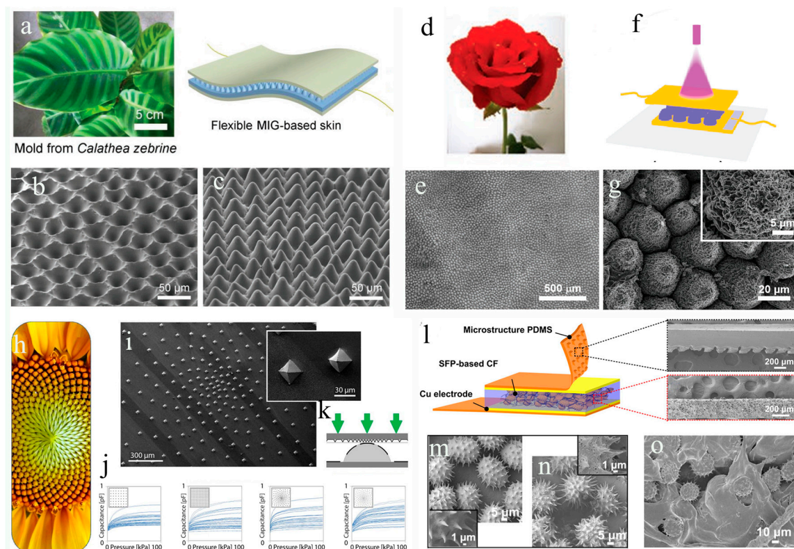
Figure 5. Bionic touch sensors based on the special structures of plants. a) A flexible sensor made with a MIG dielectric layer. b-c) SEM pictures of the molding templates. (Reprinted with permission from Ref. [43], Copyright 2018, Adv Mater) d) Schematic representation of the rose petal-shaped template. f) Schematic illustration of the pressure sensor. e-g) SEM images of the PPY/PDMS stamps. (Reprinted with permission from Ref. [81], Copyright 2020, Adv Mater) h) The organizational structure of sunflower. i) SEM images showing the top electrode layer with a pyramid-shaped spiral grid. j) Response characteristics of pyramidal orthogonal and spiral grid arrays. k) Lateral view of the electronic skin with a spiral grid. (Reprinted with permission from Ref. [41], Copyright 2018, Science Robotics) l) Conceptual illustration of flexible touch sensors based on an interlocking geometry with encapsulated SFP microcapsules. m-n) SEM images of SFP microcapsules and MWCNT/SFP microcapsules, respectively. o) SEM image of SFP-containing 3D composite film. (Reprinted with permission from Ref. [82], Copyright 2017, Nano Energy).
