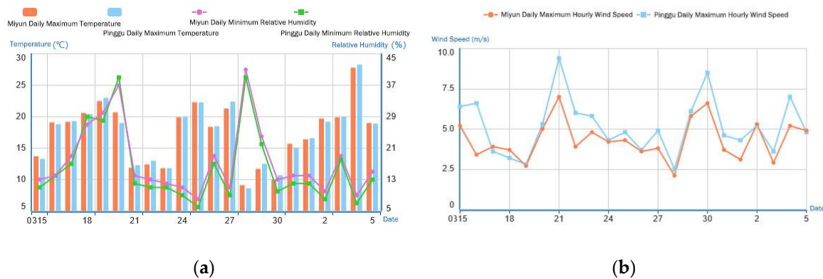
Figure 14. Trends in meteorological elements before and during the Miyun and Pinggu fires.
