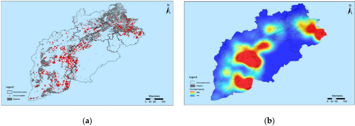
Figure 4. (a)Distribution of satellite monitoring forest fire points in the Beijing-Tianjin-Hebei- Shanxi region (from 2007 to 2017);(b)Satellite monitoring forest fire points kernel density map in the Beijing-Tianjin-Hebei-Shanxi region (from 2007 to 2017).
