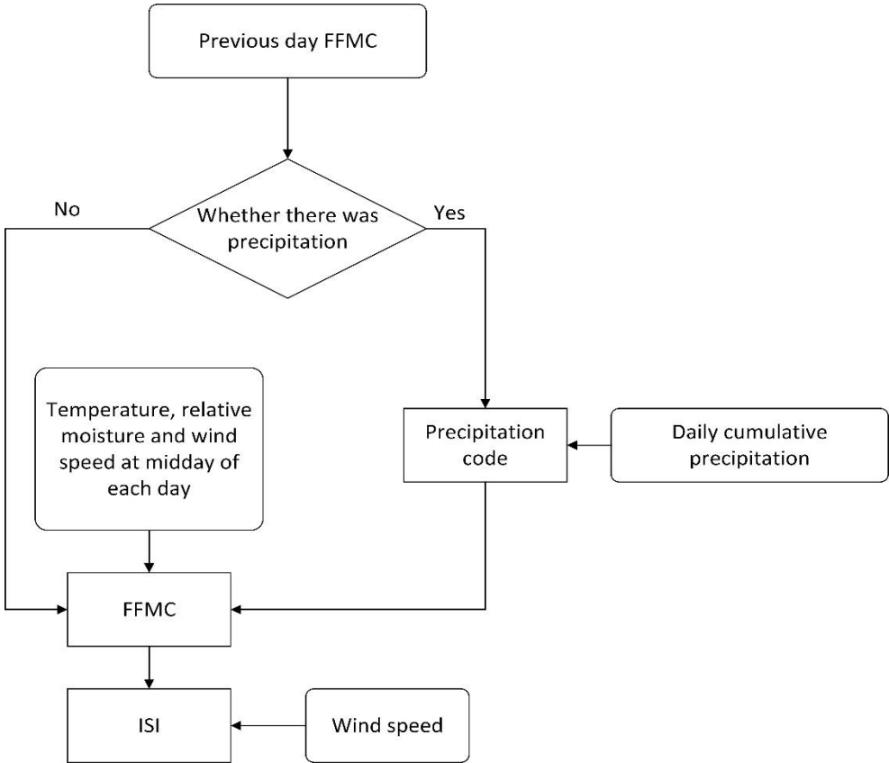
Figure 3. Flow chart of FFMCI and ISI calculation.
