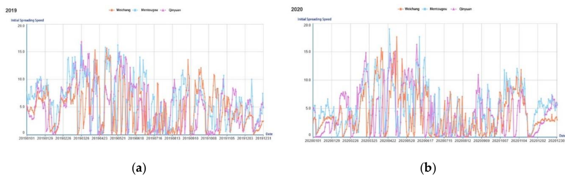
Figure 7. ISI line graph for Weichang Station, Mentougou Station and Qinyuan Station in 2019 and 2020.
