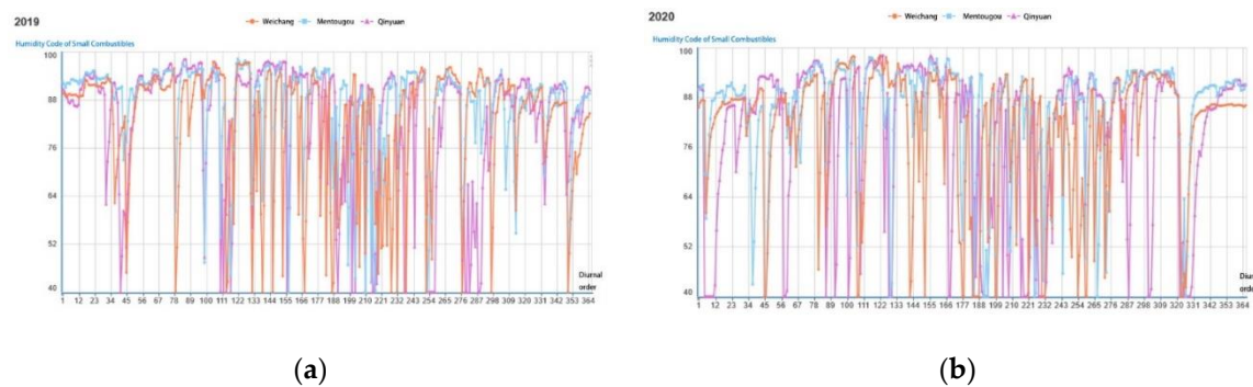
Figure 6. FPMC line graph for Weichang Station, Mentougou Station and Qinyuan Station in 2019 and 2020.
