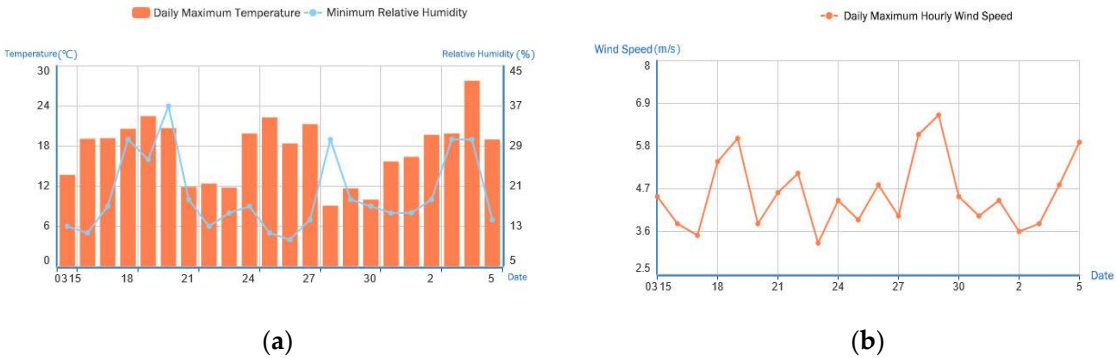
Figure 12. Trends of the meteorological elements before and during the fire (30 March) observed at the Qinyuan Station.
