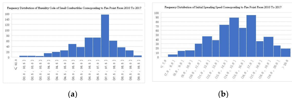
Figure 8. (a)Frequency distribution of humidity code of small combustibles corresponding to fire point from 2010 to 2017;(b)Frequency Distribution of Initial Spreading Speed Corresponding to Fire Point From 2010 To 2017.
