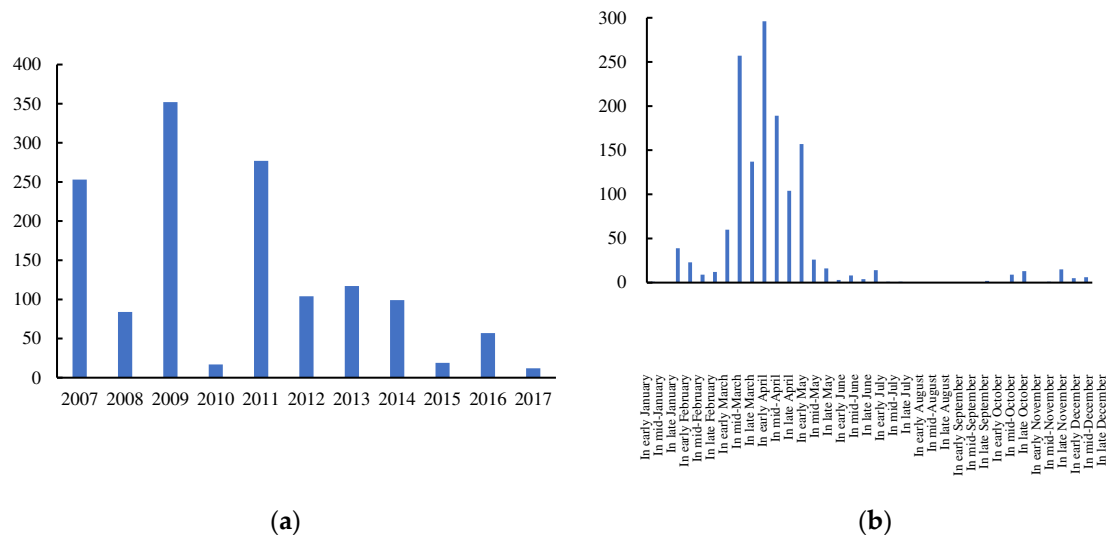
Figure 5. (a)Annual Fire Points From 2007 To 2017; (b)Annual distribution characteristics of accumulated fire points from 2007 to 2017.
