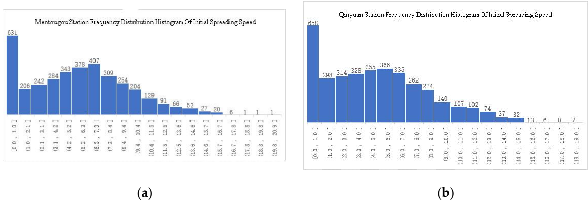
Figure 9. (a)Histogram of ISI frequency distribution at Mentougou Station (54505).(b) Histogram of ISI frequency distribution at Qinyuan Station (53875).
