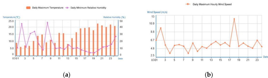
Figure 16. Trends in meteorological elements before and during the Yushe fire.
