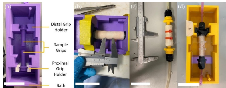
Figure 1. Developed ex vivo aortic treatment apparatus. (a) 3D printed apparatus, (b) measurement of localised 1 cm treatment region, (c) 'gripped' aorta for treatment, and (d) placement of aorta in 3D printed treatment apparatus. All scale bars are 5 cm.
