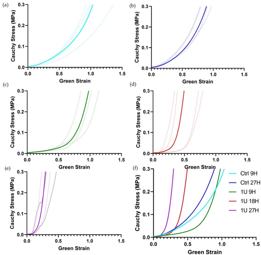
Figure 5. Cauchy stress-Green strain data from ring testing of control (Ctrl) and elastase (1U) treated samples at 9-, 18- and 27-hours. Data on graphs is color-coded by treatment group and all curves for each treatment group are shown with the median curve highlighted in bold. Cauchy stress-Green strain data is presented for (a) the 9-hour control, (b) 27-hour control, (c) 9-hour elastase, (d) 18-hour elastase, and (e) 27-hour elastase treatment groups. Stress strain curves from two rings in the 27-hour group, coloured in grey, were excluded from further analyses due to yielding prior to 300 kPa Cauchy stress – seen by the sharp dips in the curves. (f) The median curves from all groups are reproduced for comparison.
