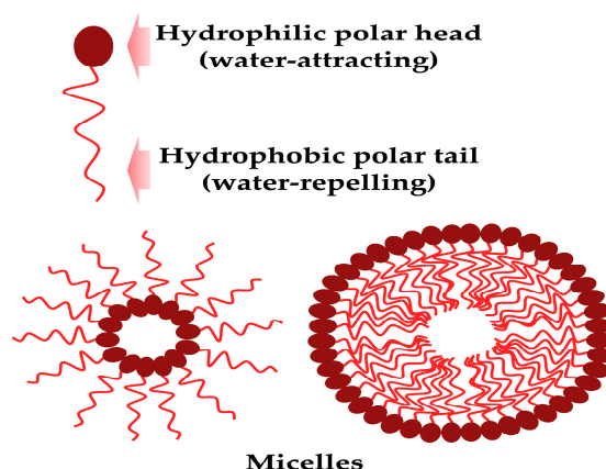
Figure 1. Biosurfactant general structure and micelles formation.
