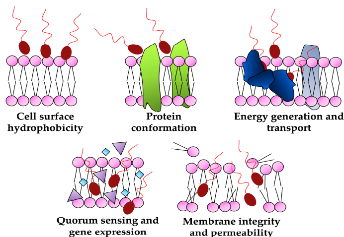
Figure 6. Biological targets of biosurfactants as antimicrobials.
