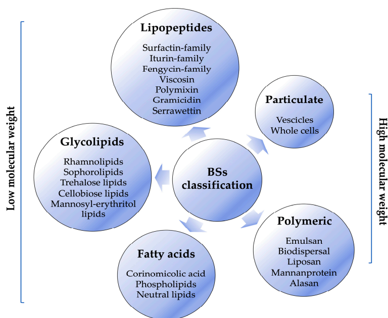
Figure 3. Biosurfactant classification.
