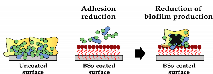
Figure 5. Antiadhesive/antibiofilm activity of biosurfactants.
