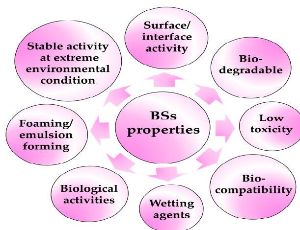
Figure 2. Biosurfactant properties.
