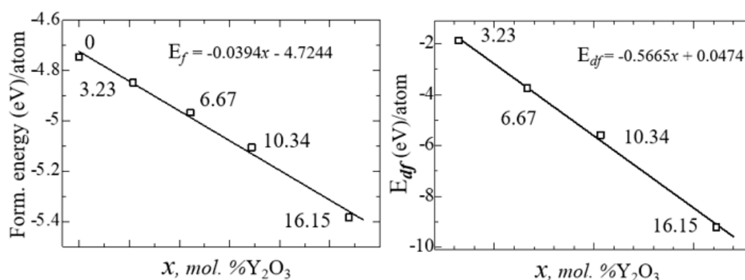
Figure 13. Formation energies and formation energy of an oxygen vacancy for YSZ as a function of \text{Y}_2\text{O}_3 concentration.
