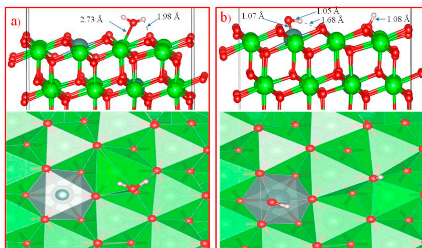
Figure 18. Molecularly adsorbed water (a) and dissociated surface hydroxyls. (b) in the \text{H}_2\text{O} -YSZ (101) model/.
