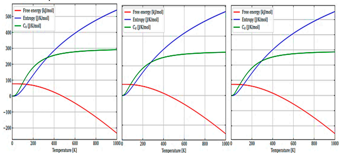
Figure 6. Temperature dependence of free energy, entropy and heat capacity of a 12-atomic supercell for: m- \text{ZrO}_2 (a), t- \text{ZrO}_2 (b), and m- \text{ZrO}_2 (c).
