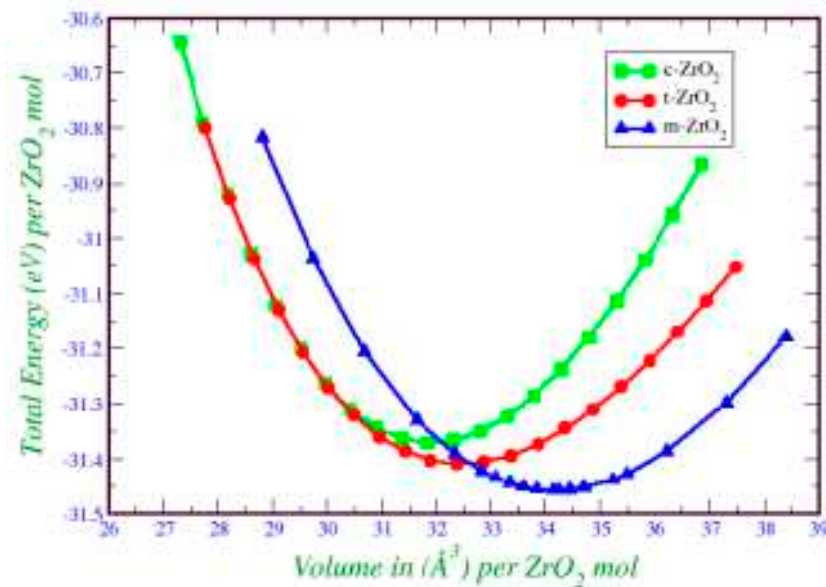
Figure 8. Total energy as function of volume [54].
