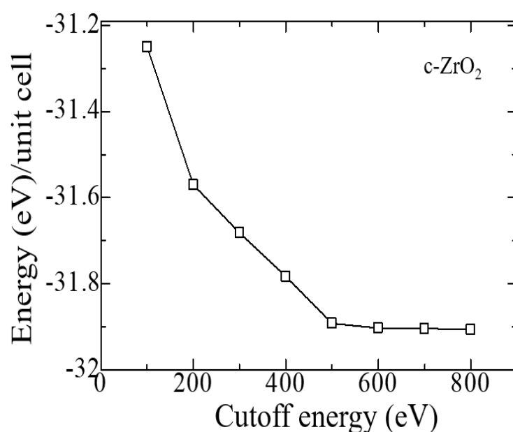
Figure 3. Total energy of the c-ZrO 2 unit cell as a function of the cutoff energy ( 4 \times 4 \times 4 k-points).
