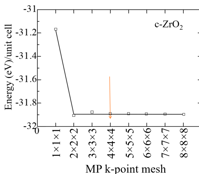
Figure 2. The total energy of the c- ZrO_2 unit cell as a function of the number of k-points under the condition ENCUT=1.3 \cdot ENMAX .
