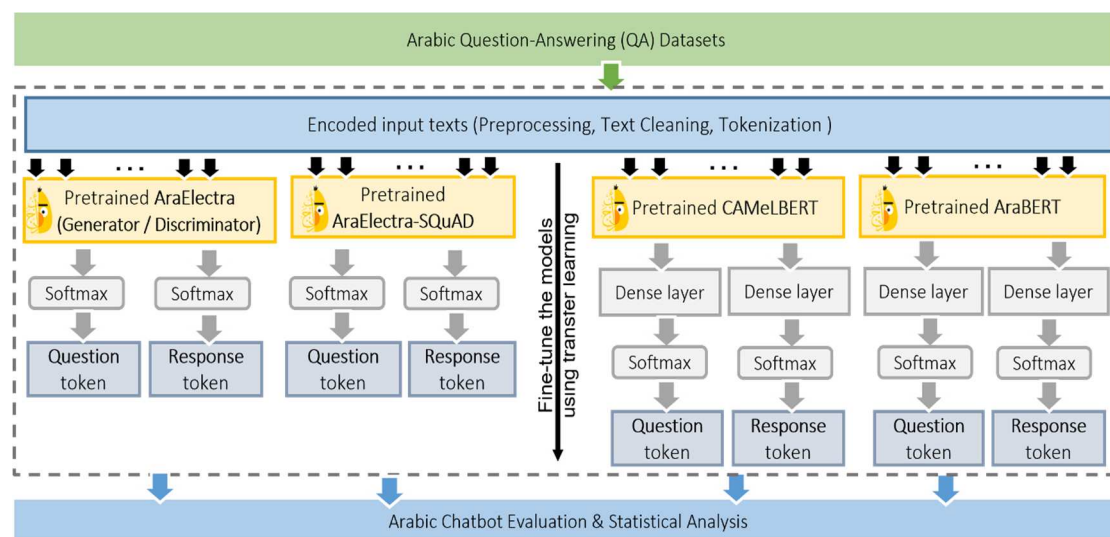
Figure 2. General framework of the methodology used in this study.
