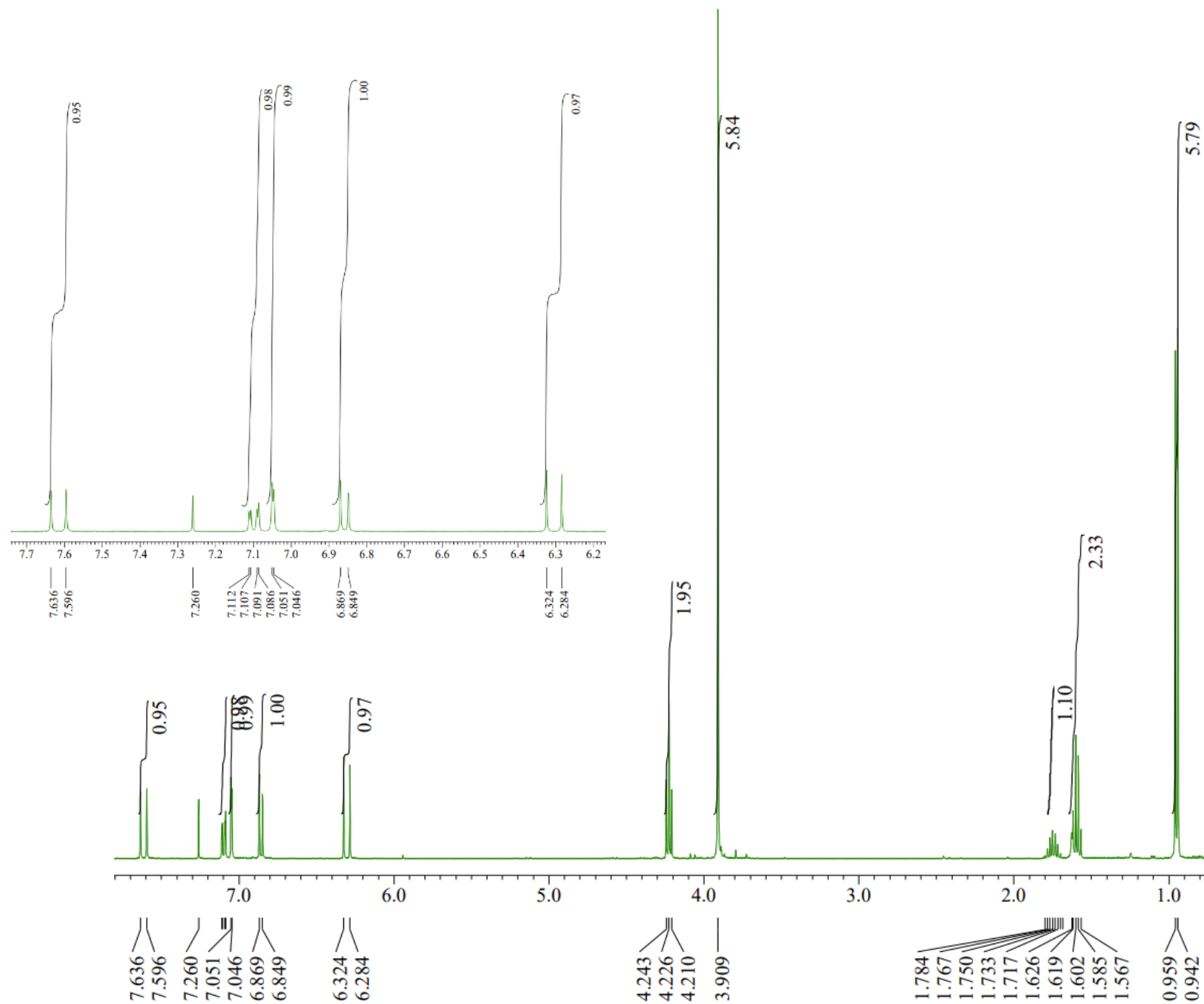
Figure S2. ^1\text{H} -NMR Spectrum of isoamyl ( E )-3-(3,4-dimethoxyphenyl)acrylate ( 1 )
