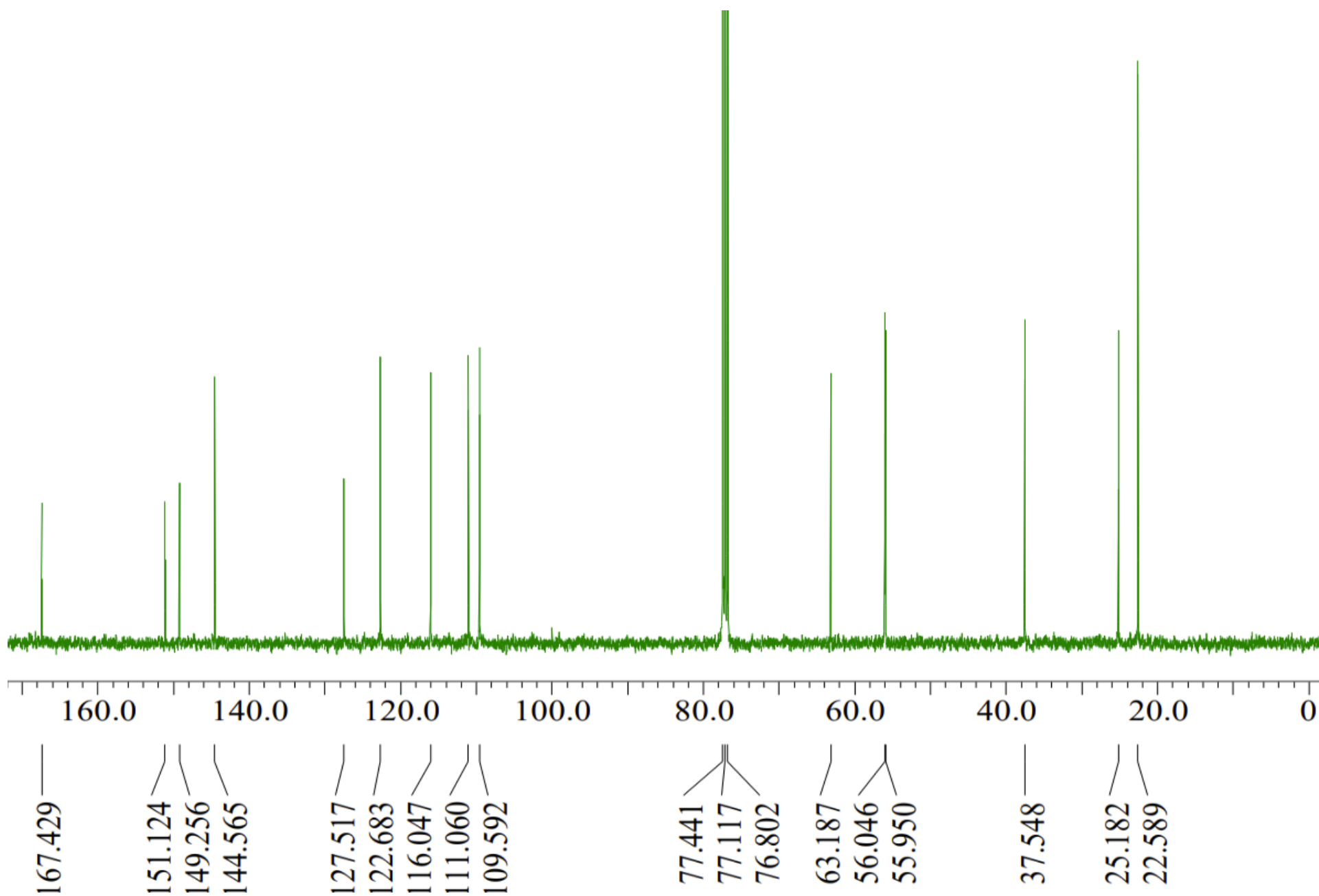
Figure S3. ^{13}\text{C} -NMR Spectrum of isoamyl ( E )-3-(3,4-dimethoxyphenyl)acrylate ( 1 )
