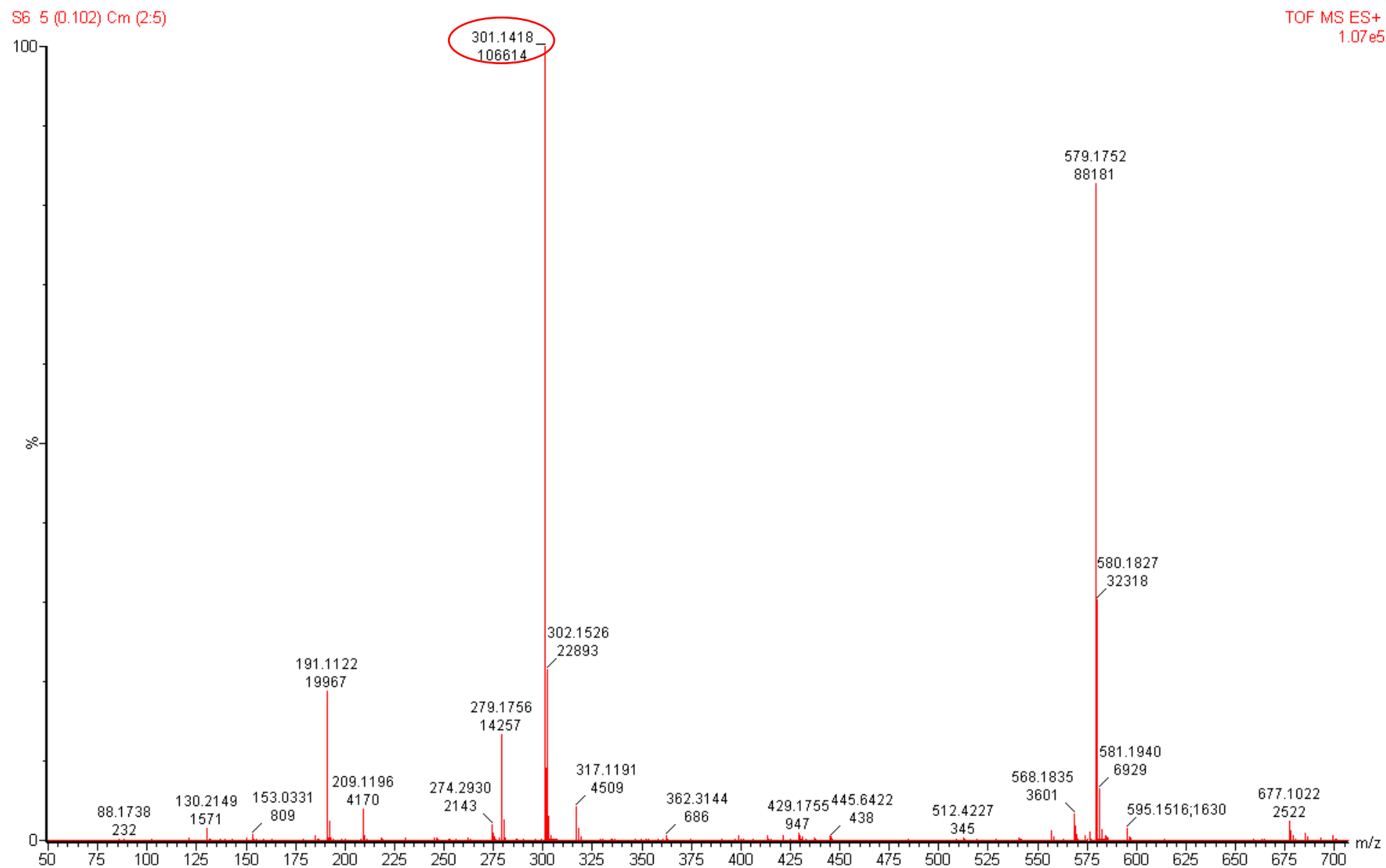
Figure S4. High Resolution Mass Spectrum of isoamyl ( E )-3-(3,4-dimethoxyphenyl)acrylate ( 1 )
