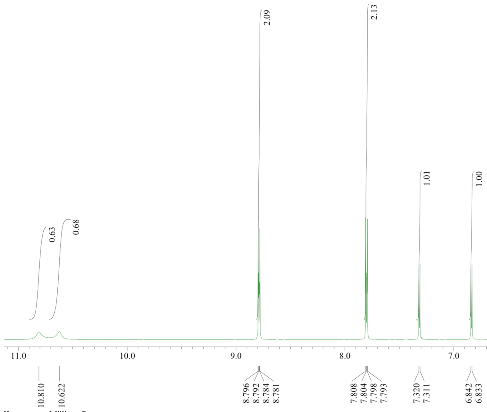
Figure S2. ^1\text{H} NMR Spectrum of N' -(5-bromofuran-2-carbonyl)isonicotinohydrazide ( 1 )
