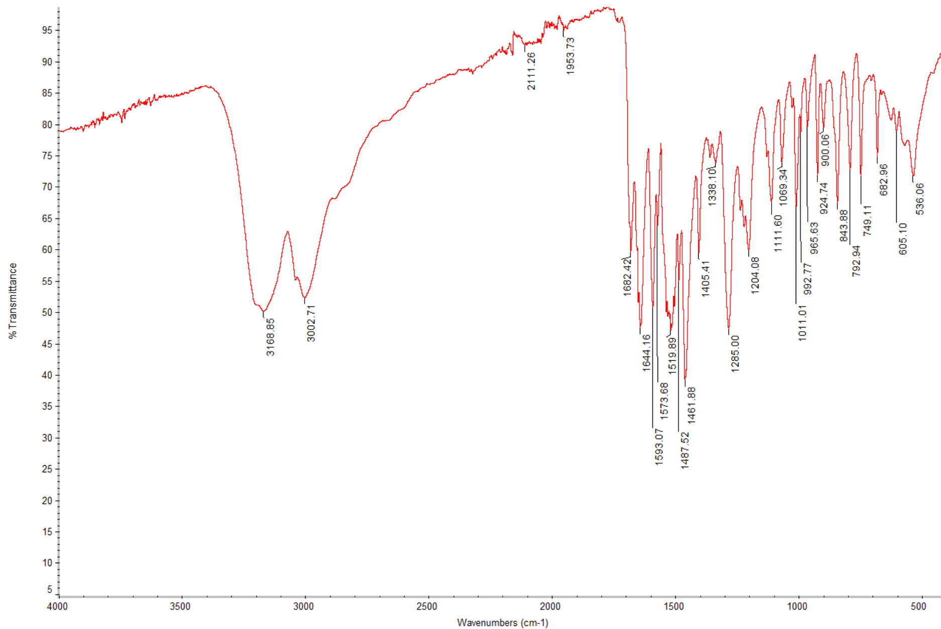
Figure S1. IR Spectrum of N' -(5-bromofuran-2-carbonyl)isonicotinohydrazide ( 1 )
