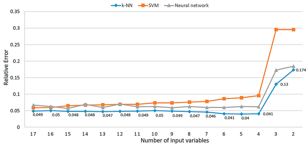
Figure 10. Relative error of ML models testing.
