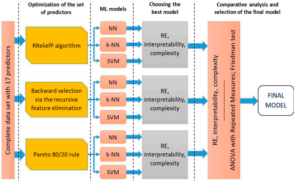
Figure 7. Steps of the methodological procedure from the optimization of the set of predictors to the selection of the final model
