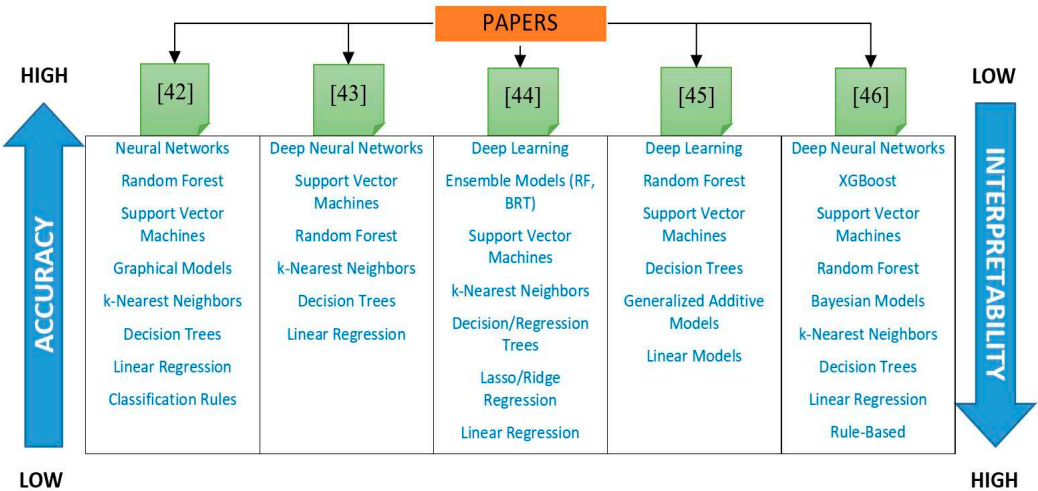
Figure 8. ML models ranked by accuracy and interpretability in various published research papers.
