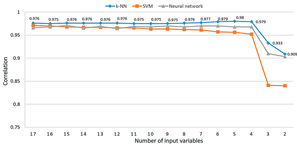
Figure 11. Correlation of ML models prediction results with data test set.
