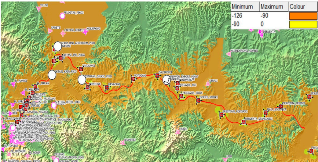
Figure 2. Layout of eNodeB locations with marked signal propagation in the research area.
