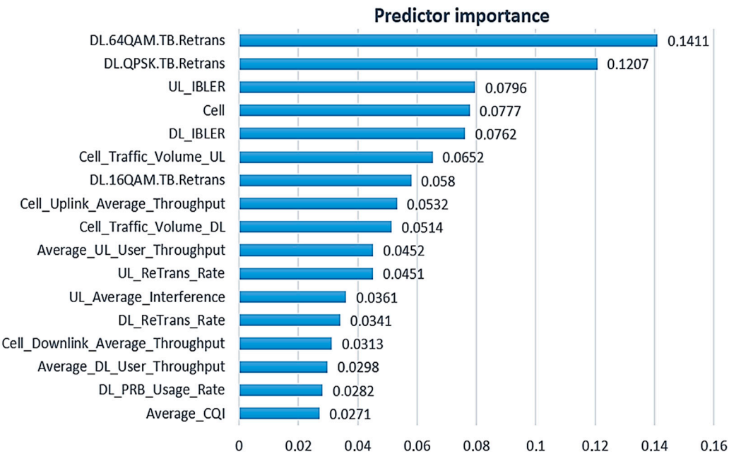
Figure 9. Independent variables ranked by PI.
