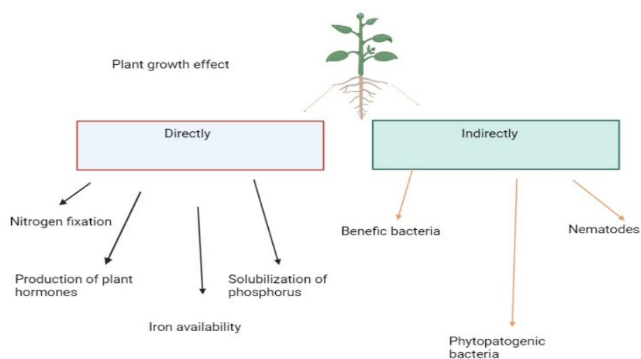
Figure 1. Plant growth is facilitated by PGPB, which produces siderophores, increases iron availability, and produces hormones like auxins, gibberellins, and cytokinin which influence plant
