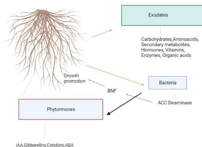
Figure 2. Microorganisms and plants produce metabolites that act as signaling molecules and substrates when they interact. Besides fixing nitrogen and solubilizing nutrients (phosphate and iron), microorganisms also produce hormones, which stimulate plant growth. A dashed line indicates a
