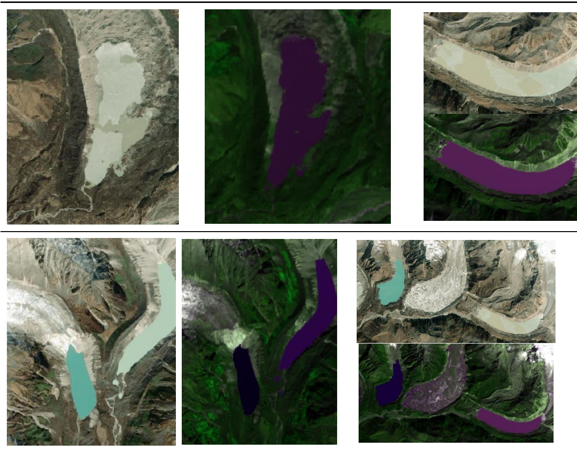
Figure 3. Glacial lake classification using NDWI on sentinel-2 with false color composite.
