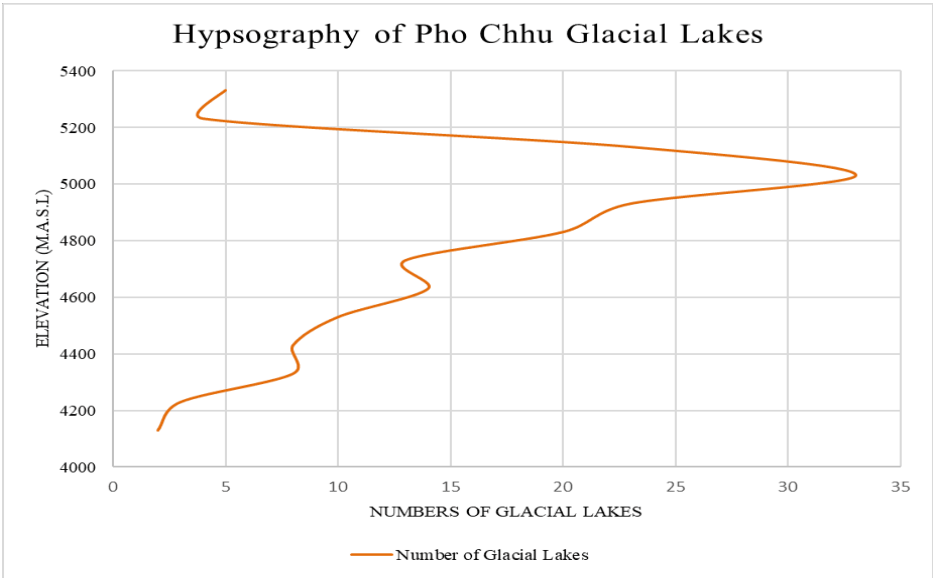
Figure 6. Hypsometry of Phochhu glacial lake distributions.
