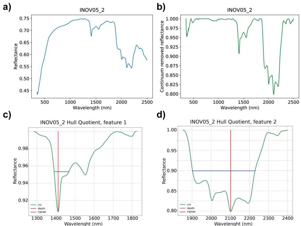
Figure 9. Example of the graphical products of the spectra INOV5_2, available in the spectral library, for consultation and analysis: (a) Raw_spectra; (b) Processed_spectra (with removed continuum); (c) and (d) Spectra_absortions, with different wavelengths and depths, where crs is the continuum removed spectra; depth is the absorption depth and FWHM is the full width at half maximum.
