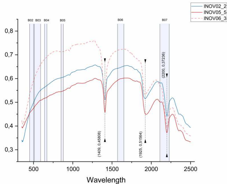
Figure 11. Absorption features and reflectance peaks of reference spectra from the samples of the Aldeia pegmatite. Three Aplite-Pegmatite spectra were used as examples. The blue rectangles represent the spectral range of the Landsat 8 and 9 bands superimposed on the raw spectra.
