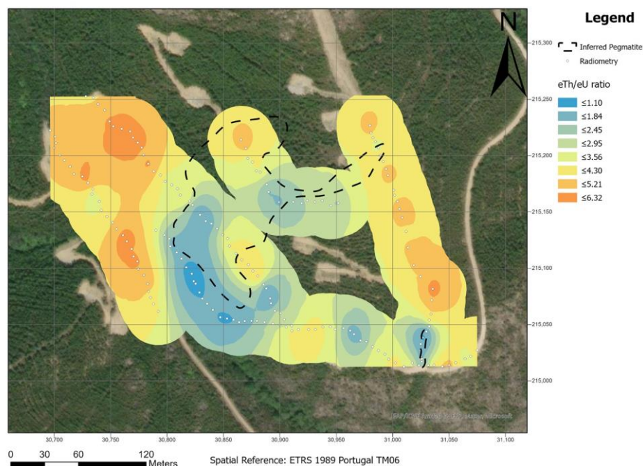
Figure 8. Map of equivalent Thorium – equivalent Uranium (eTh/eU) ratio on the Aldeia area. A 30 m buffer was applied to the Kriging interpolation.
