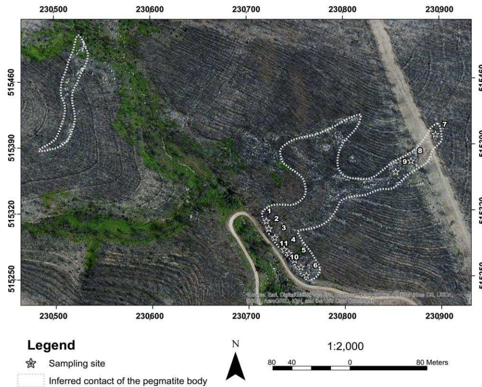
Figure 2. The zoomed map of the sampling area within the Aldeia pegmatite, on the Mina do Barroso concession.
