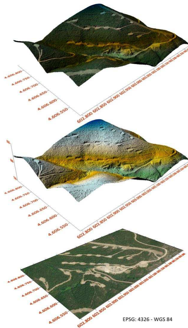
Figure 5. Stacked images created with Surfer® (Golden Software, LLC): ArcGIS World Imagery Basemap (bottom); hillshade image of the area (middle); World Imagery Basemap draped over the
