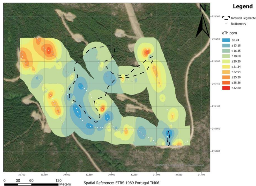
Figure 7. Map of equivalent Thorium (eTh) concentration in the Aldeia area. A 30 m buffer was applied to the Kriging interpolation.
