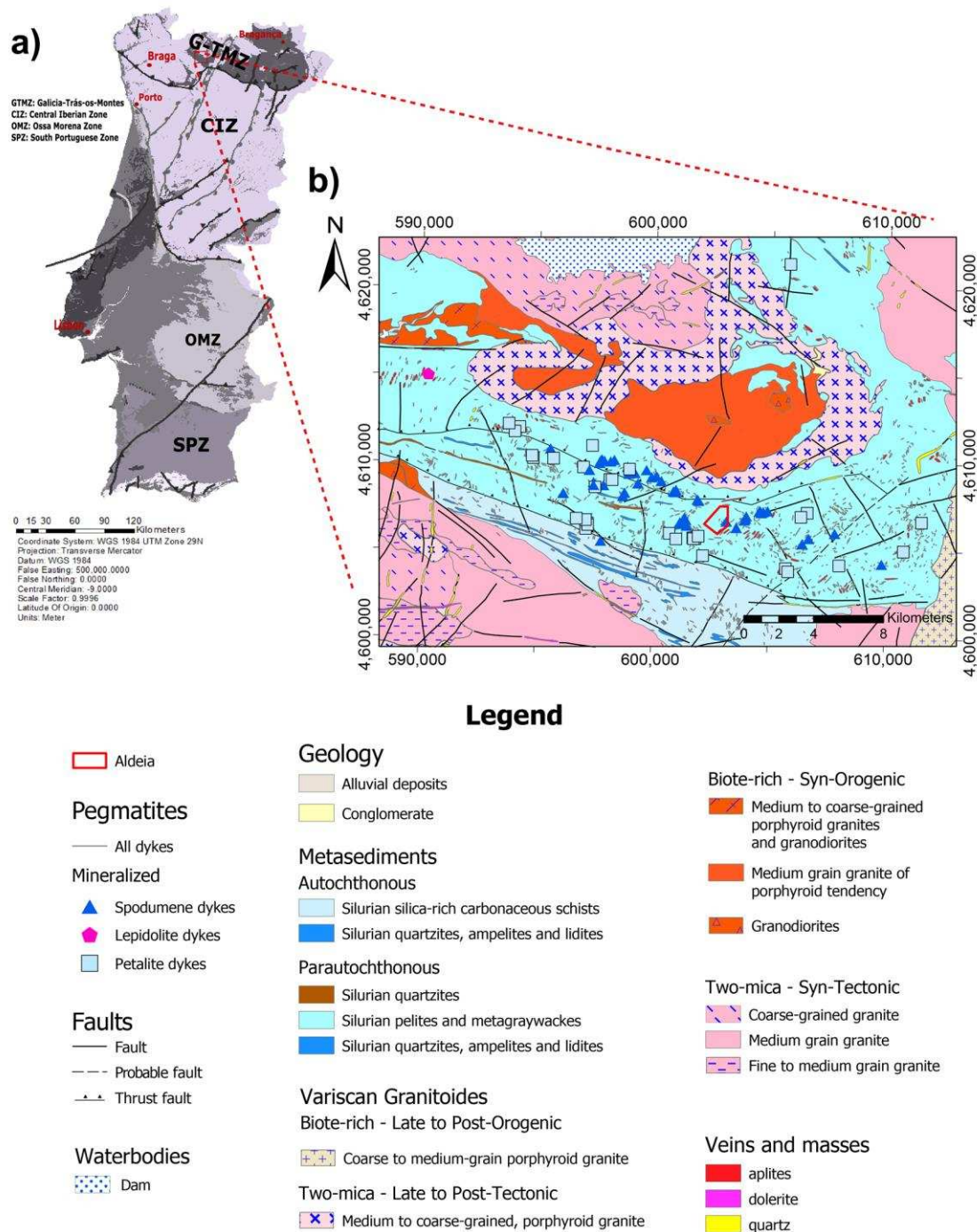
Figure 1. (a) The geotectonical map of Portugal, demonstrating that the study area belongs to the Galicia-Trás-os-Montes zone [29]; (b) Geological setting of the study area from the Portuguese Geological Map at the scale 1:2000,000, sheet 2 ( https://www.lneg.pt/en/product/geological-map-of-portugal-scale-1200-000/ ).
