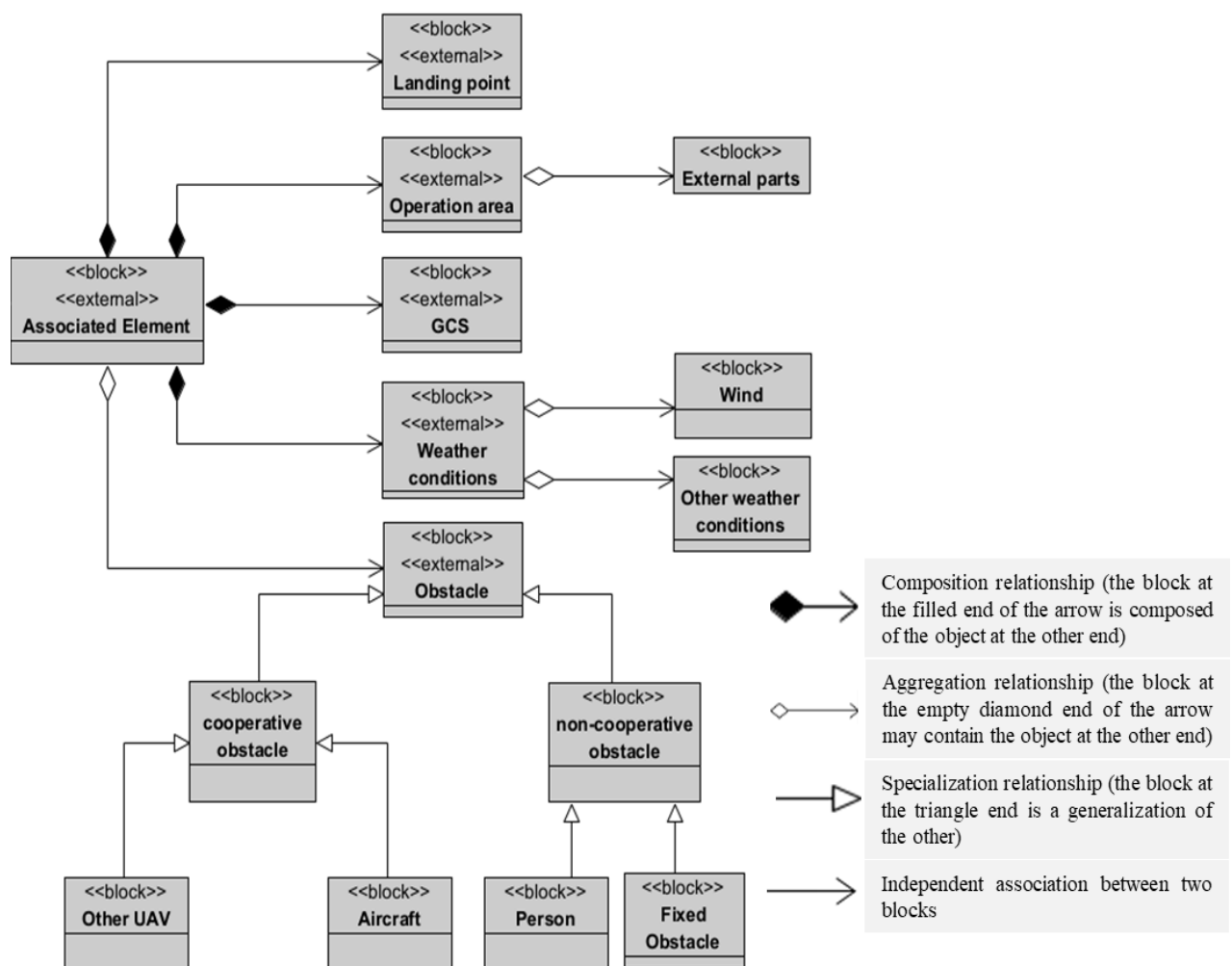
Figure 12. Description of the "Associated Element" block included in the block definition diagram of the advanced air mobility.
