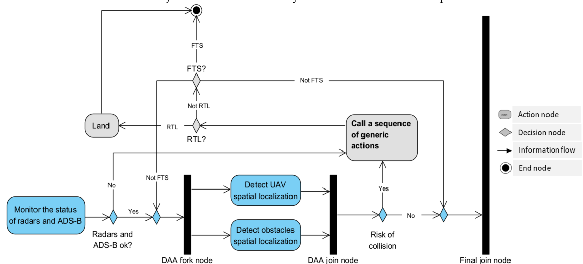
Figure 16. Modeling of the sub-activity Detect and avoid obstacles containing the sequence of actions to achieve the second SA goal.
