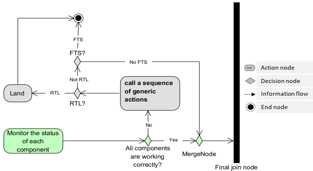
Figure 18. Modeling of the sub-activity Monitor the state of the UAV containing the sequence of actions to achieve the fourth SA goal.
