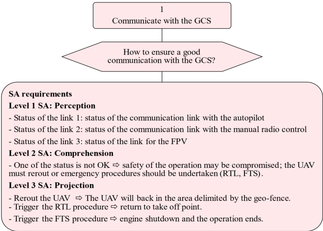
Figure 4. Decomposition of the first sub-goal of the UAV's GDTA: (1) communicate with the GCS. The hexagonal shape represents the decision about how to ensure a good communication with the GCS. The answer to this question leads to the description of the three SA levels associated with communication with the GCS.
