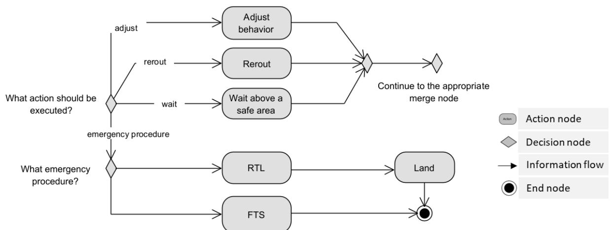
Figure 14. Modeling of the sub-activity Call a sequence of generic actions , containing the sequence of actions to resolve a problem detected during the verification of the situational awareness requirements.
