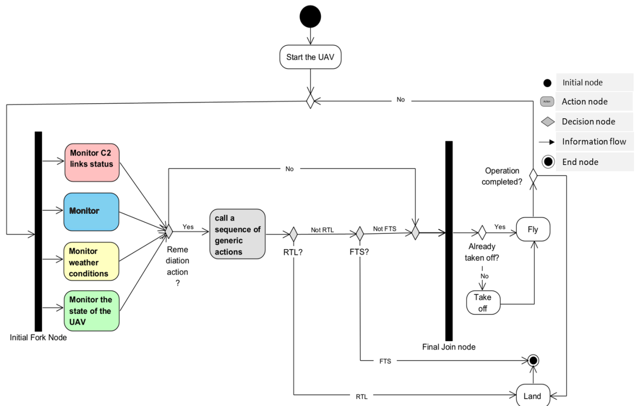
Figure 13. High-level modelling of the UAV behavior in the AAM system, shown in an activity diagram. Before taking off, the UAV must verify that it has achieved all its SA goals. To do so, it must follow sequences of parallel sub-activities which allow it to maintain SA and ensure the safety of the AAM system. The first step is followed by a fork node (labeled Initial Fork Node ) which represents the main goal: ensuring the safety of the AAM system. From this node, a parallel branch is made to the sub-activities Monitor C2 links status , Monitor threats , Monitor weather conditions , Monitor the state of the UAV , which are related, respectively, to the C2 management system, the DAA management system, the weather detection system, and the system responsible for monitoring the state of the UAV. If the execution of one of these four actions leads to a need for remediation, the process continues through the sub-activity Call a sequence of generic actions and an appropriate remediation action is executed. These generic actions and each of the four other sub-activities are described below.
