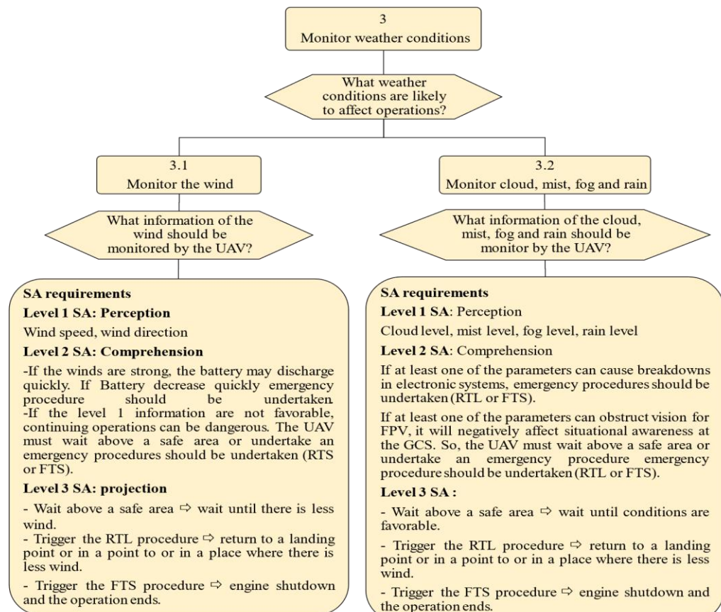
Figure 9: Decomposition of the decision about weather conditions to be monitored. These are wind cloud, mist fog and rain.
