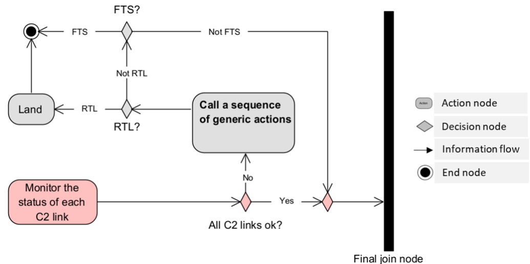
Figure 15. Modeling of the sub-activity Monitor C2 links status containing the sequence of actions to achieve the first SA goal.
