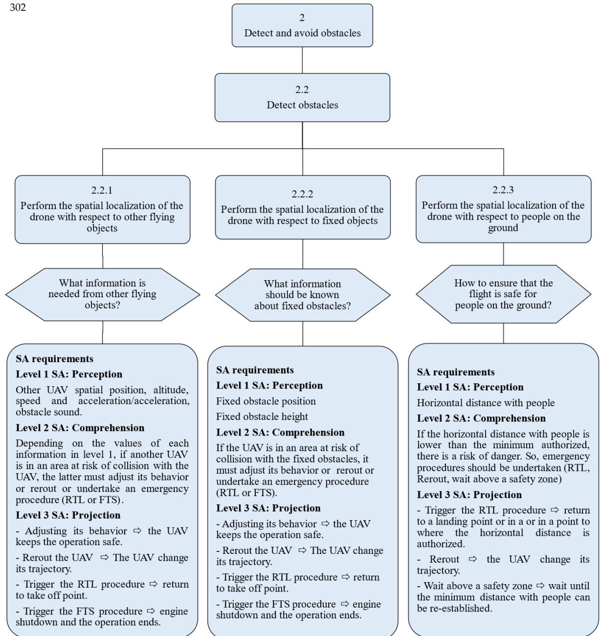
Figure 7. Decomposition of sub-goal 2.2 of the UAV's GDTA. The achievement of this sub-goal requires three other sub-goals to be achieved. The decomposition of sub-goal 2.2.1 allows spatial information relating to other flying obstacles to be identified, which is necessary to assess the risk of collision. The decomposition of sub-goal 2.2.2 allows identification of information relating to nearby fixed obstacles in order to assess the risk of collision with them. The decomposition of sub-goal 2.2.3 allows identification of the information necessary to assess the proximity between the UAV and people on the ground.
