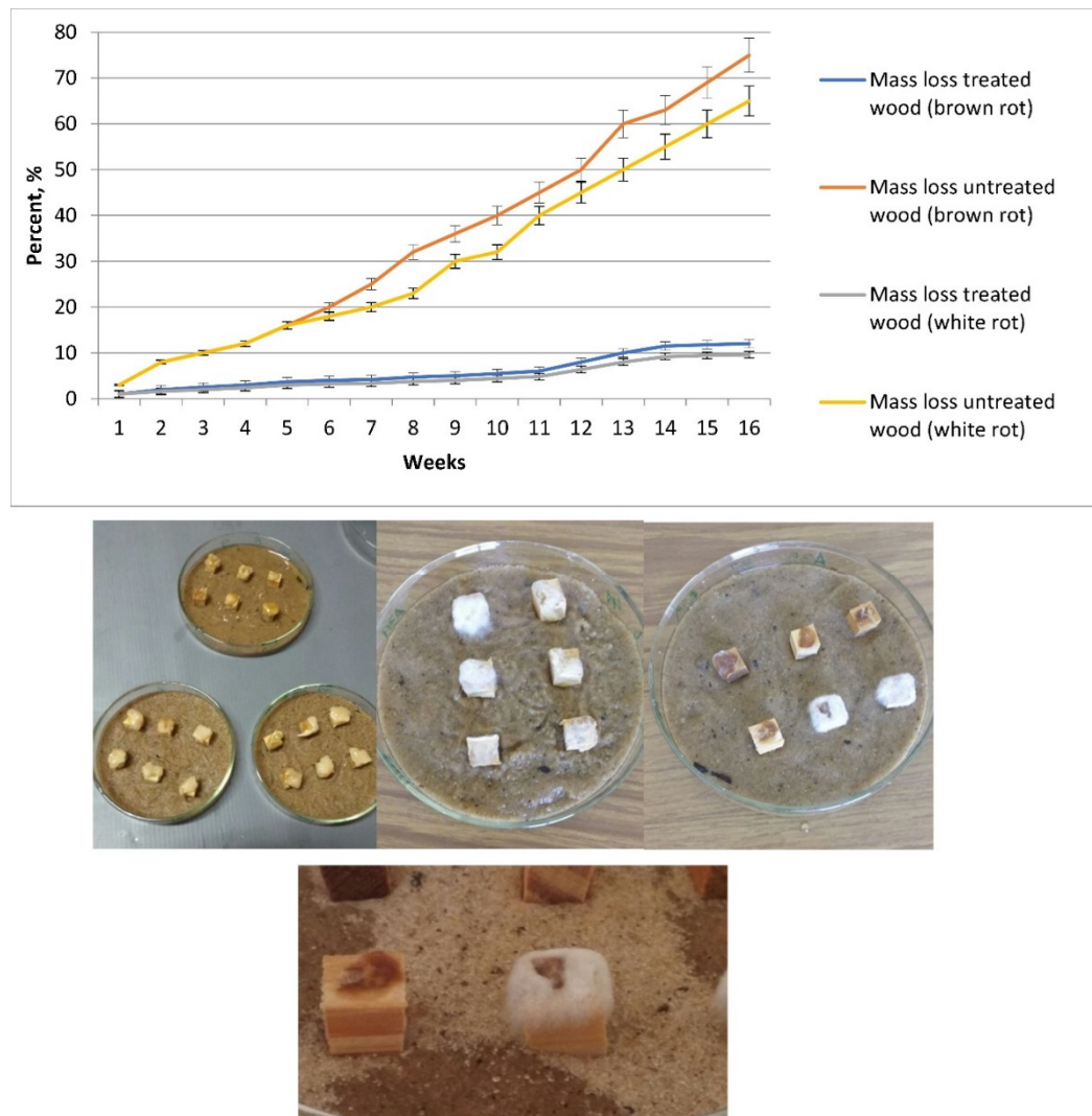
Figure 1. Decay resistance test.
