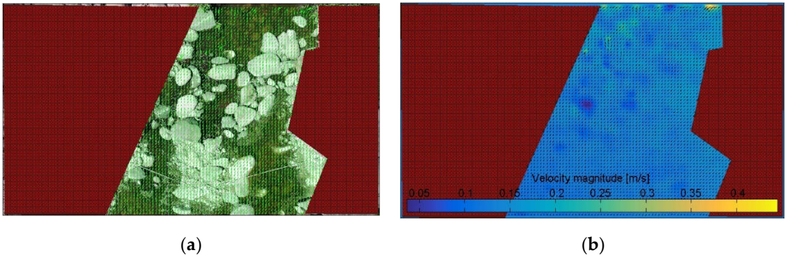
Figure 9. The studied section of Eresos captured by the UAV (a) the vectors of velocity are depicted in green color and the red area was excluded from analysis; (b) the vectors of velocity are depicted in a colorized scale where dark blue corresponds to 0 and yellow up to 0.45 m/s.
