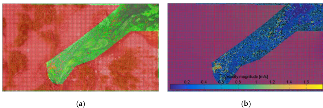
Figure 7. The studied section of Evergetoulas – Kerameia captured by the UAV (a) the vectors of velocity are depicted in green color and the red area was excluded from analysis; (b) the vectors of velocity are depicted in a colorized scale where dark blue corresponds to 0 and yellow up to 1.8 m/s.
