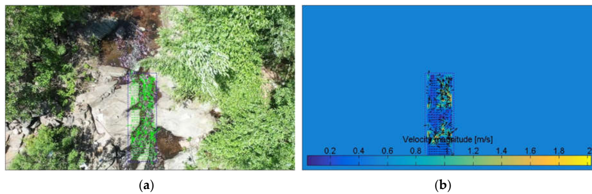
Figure 11. The studied section of Kremasti Bridge – Agia Paraskevi captured by the UAV (a) the vectors of velocity are depicted in green color; (b) the vectors of velocity are depicted in a colorized scale where dark blue corresponds to 0 and yellow to 2 m/s.
