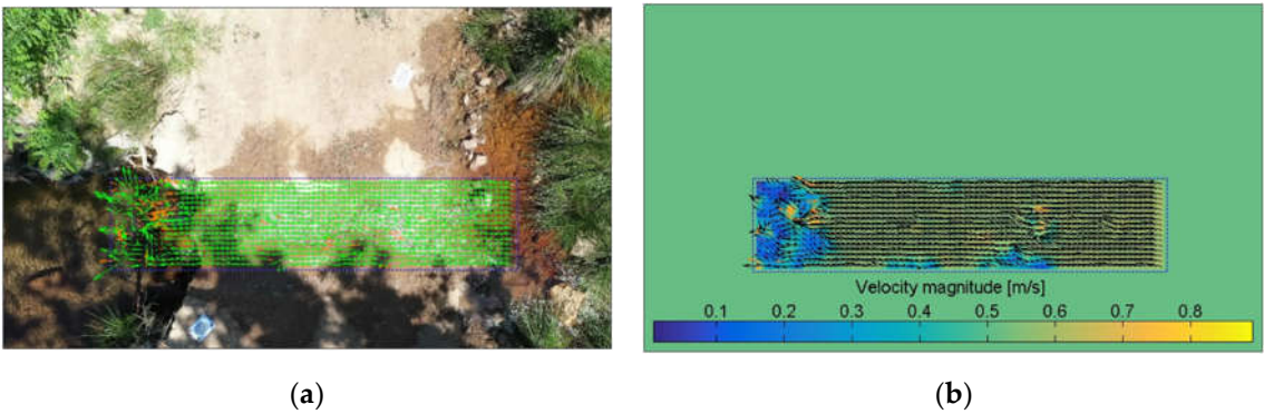
Figure 8. The studied section of Pterounta – Vathilimno captured by the UAV (a) the vectors of velocity are depicted in green color; (b) the vectors of velocity are depicted in a colorized scale where dark blue corresponds to 0 and yellow to >0.8 m/s.
