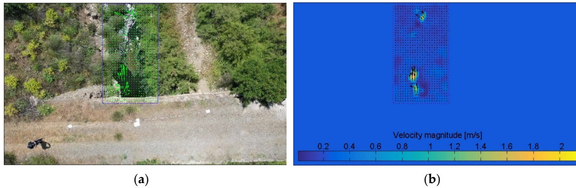
Figure 5. The studied section of Agia Anna – Polichnitos captured by the UAV (a) the vectors of velocity are depicted in green color; (b) the vectors of velocity are depicted in a colorized scale where dark blue corresponds to 0 and yellow to >2 m/s.
