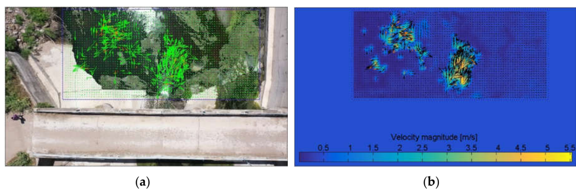
Figure 13. The studied section of Prinis Bridge – Agia Paraskevi captured by the UAV (a) the vectors of velocity are depicted in green color; (b) the vectors of velocity are depicted in a colorized scale where dark blue corresponds to 0 and yellow up to 5.5 m/s.
