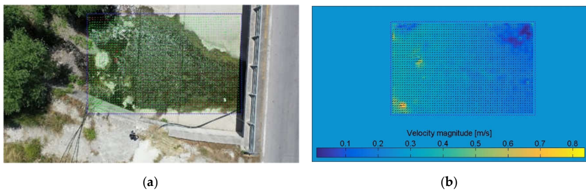
Figure 6. The studied section of Kalloni captured by the UAV (a) the vectors of velocity are depicted in green color; (b) the vectors of velocity are depicted in a colorized scale where dark blue corresponds to 0 and yellow up to 0.8 m/s.
