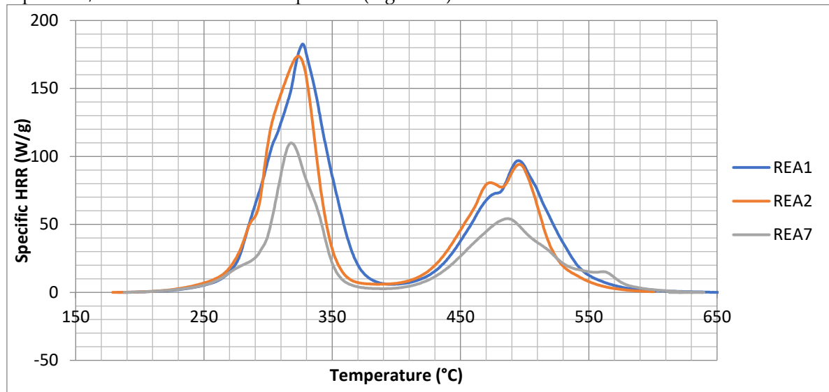
Figure 16. Comparison between REA1 (no flame retardants), REA2 (3 phr of ATO, 90 phr CaCO_3 ), and REA7 (3 phr of ATO and 90 phr of MDH).
