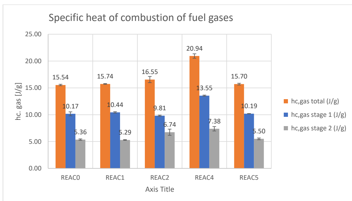
Figure 19. Comparison of h_{c, \text{gas}} in REAC0 – REAC5. Specifically, REAC4 contains an HCl scavenger, while REAC5 a trivial GCC.
