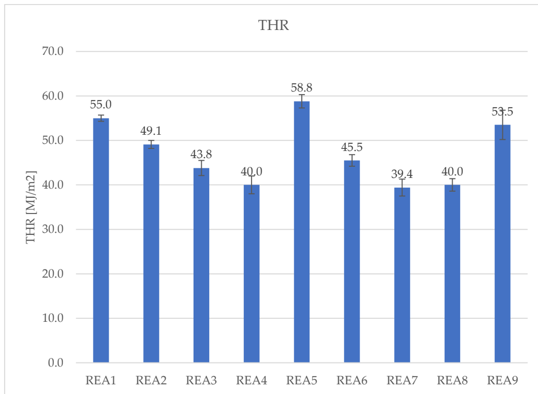
Figure 5. THR of the formulations in Table 1, REA1-REA9.
