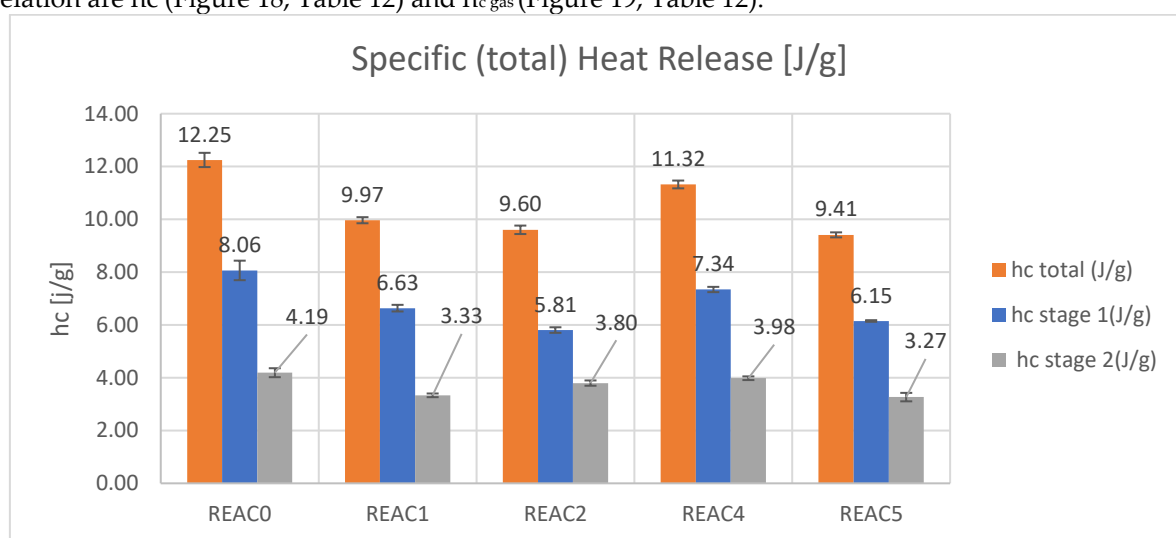
Figure 18. Comparison of h_c in REAC0 – REAC5. Specifically, REAC4 contains an HCl scavenger, while REAC5 a trivial GCC.
