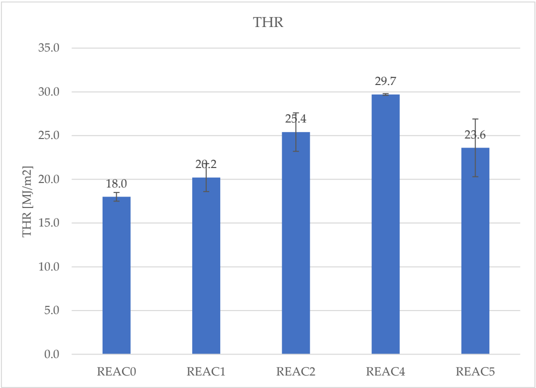
Figure 11. THR of the formulations REAC0-5.
