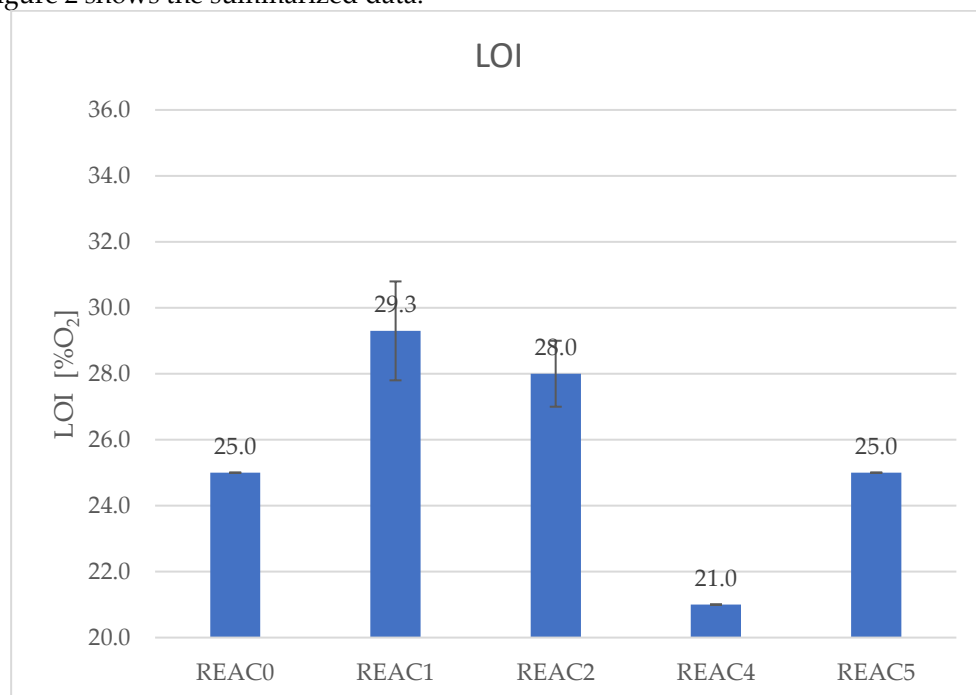
Figure 2. LOI of the formulations in Table 2, REAC0-REAC9.
