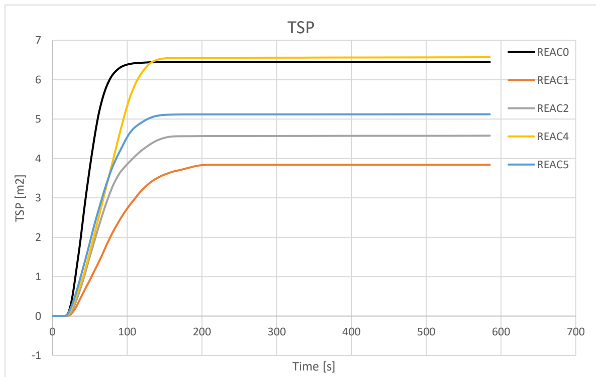
Figure 15. TSP(t) of the formulations REAC0-5.
