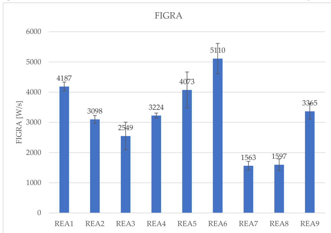
Figure 4. FIGRA of the formulations in Table 1, REA1-REA9.
