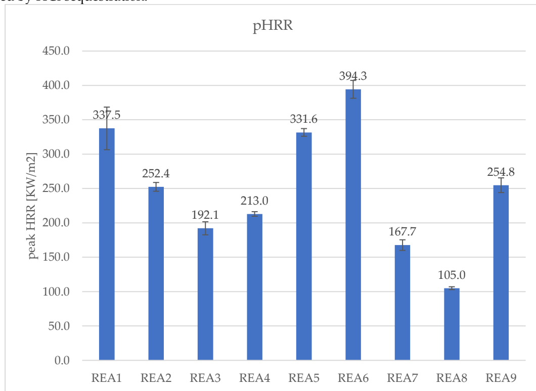
Figure 3. pHRR of the formulations in Table 1, REA1-REA9.
