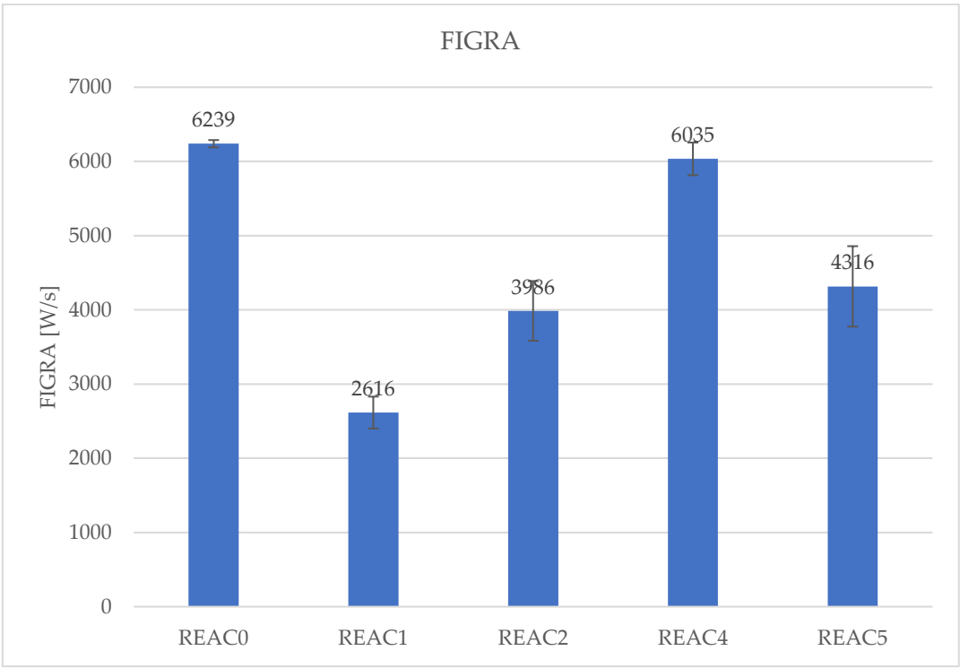
Figure 10. FIGRA of the formulations REAC0-5.
