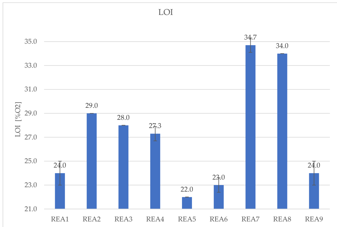
Figure 1. LOI of the formulations in Table 1, REA1-REA9.
