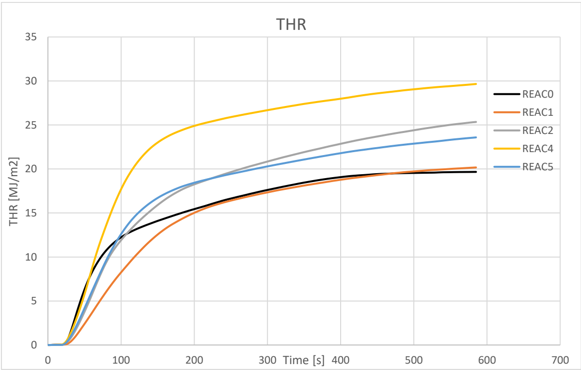
Figure 13. THR(t) of the formulations REAC0-5.
