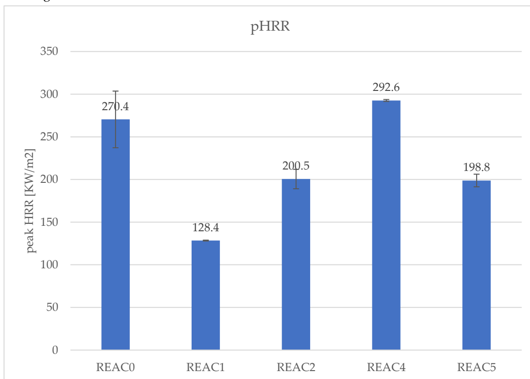
Figure 9. pHRR of the formulations REAC0-5.
