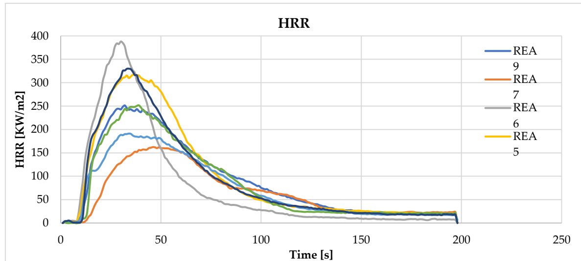
Figure 7. HRR (t) of the formulations in Table 1, REA1-REA9.
