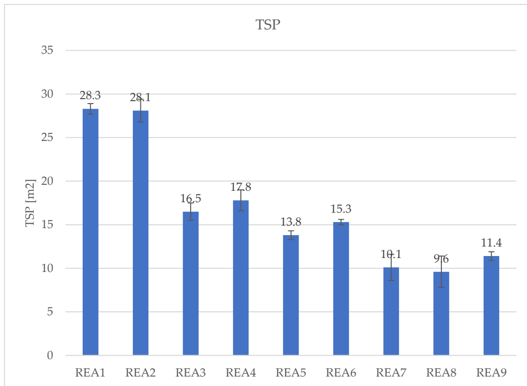
Figure 8. TSP of the formulation REA1-REA9.
