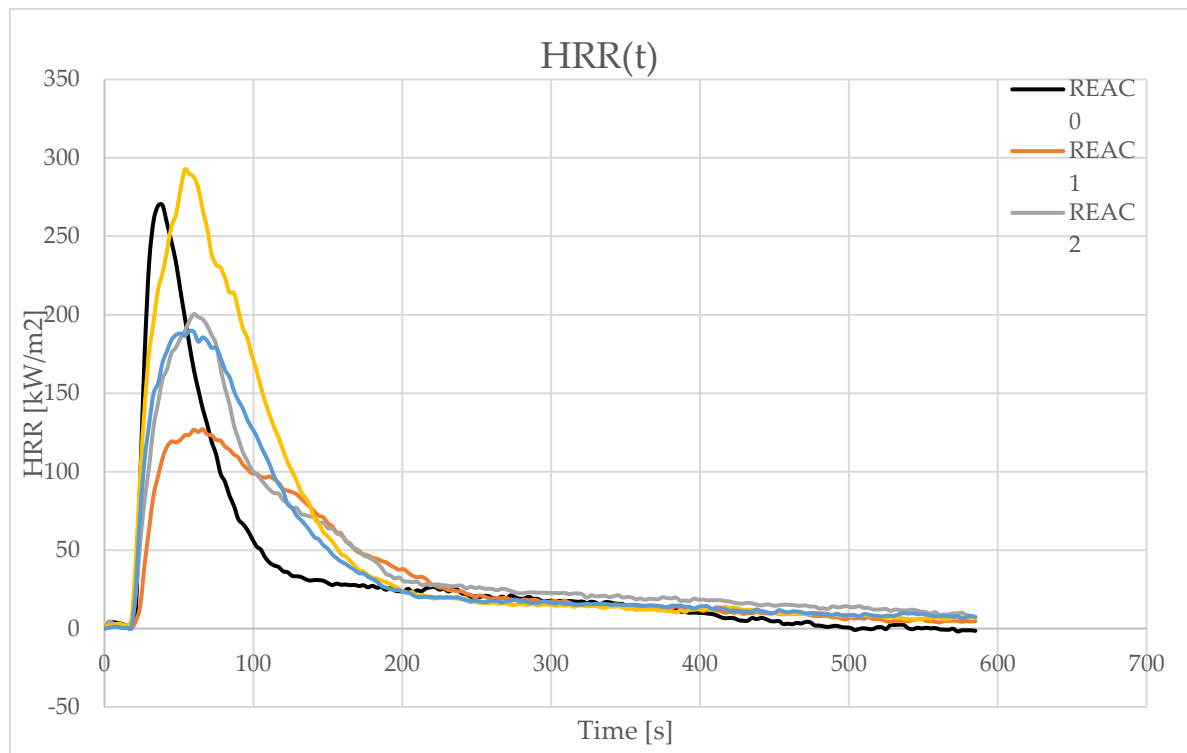
Figure 14. HRR(t) of the formulations REAC0-5.
