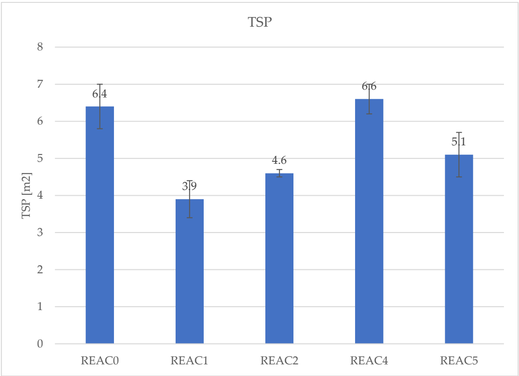
Figure 12. TSP of the formulations REAC0-5.
