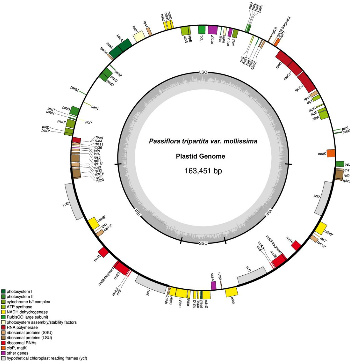
Figure 1. Plastid genome of Passiflora tripartita var. mollissima . The thick lines indicate the IR1 and IR2 regions, which separate the SSC and LSC regions. Genes marked inside the circle are transcribed clockwise, and genes marked outside the circle are transcribed counterclockwise. Genes are color-coded based on their function, shown at the bottom left. The inner circle indicates the inverted boundaries and GC content.
