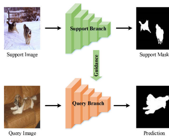
Figure 1. Typical structure of the few-shot semantic segmentation.
