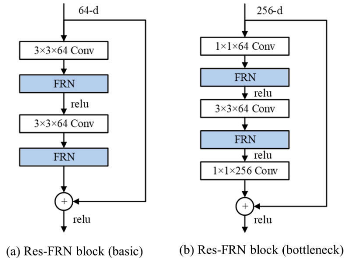
Figure 4. Schematic diagram of the designed Res-FRN block. (a) Res-FRN block (basic); (b) Res-FRN block (bottleneck).
