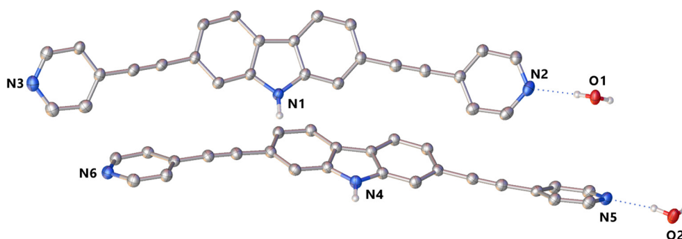
Figure 1. X-ray crystal structure of 1·H 2 O with thermal ellipsoids drawn at 30 % probability level. Only H-atoms located on heteroatoms and water molecules are shown for clarity.
