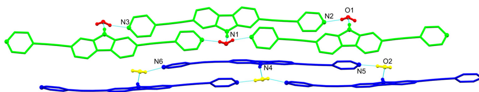
Figure 2. View along the c -axis of the hydrogen-bonded chains found in 1·H 2 O with moieties colored according to their symmetry equivalence.
