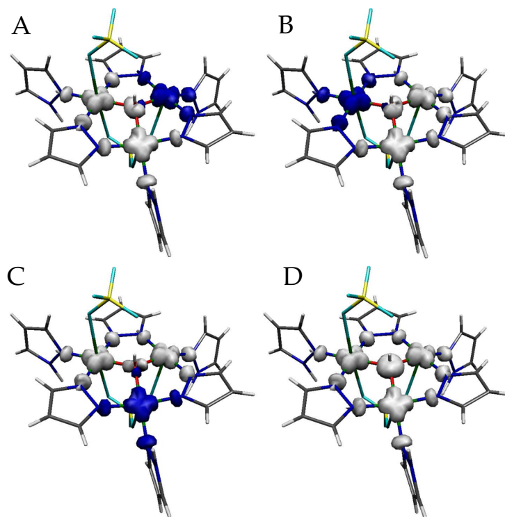
Figure S3. Spin density surfaces for 1-Cu 3 of the antiferromagnetic configurations (A-C) and the ferromagnetic one (D). Grey colour corresponds to alpha spin density and blue colour to beta spin density
