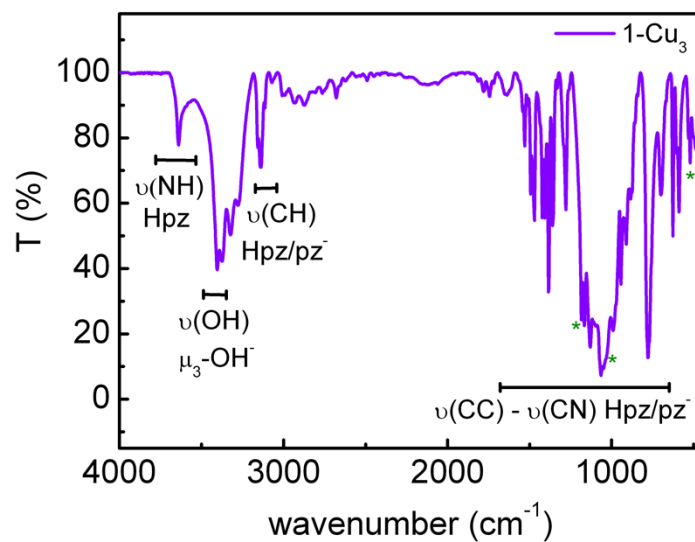
Figure S2. FTIR Spectrum of 1-Cu 3 highlighting the bands of the protonated (Hpz) and deprotonated (pz - ) pyrazolato ligand. The stretching of the μ 3 -OH - unit is also observed. The green asterisks show the vibrations associated to the [BF 4 ] - group.
