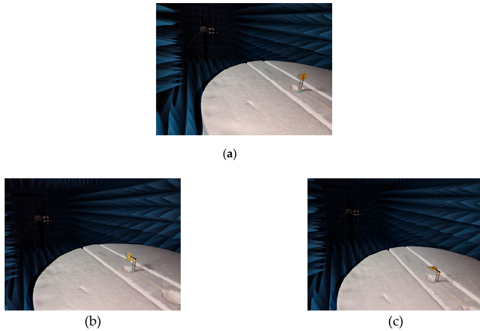
Figure 11. The measurement setup for radiation patterns. (a) x-y plane; (b) x-y plane; (c) x-y plane.
