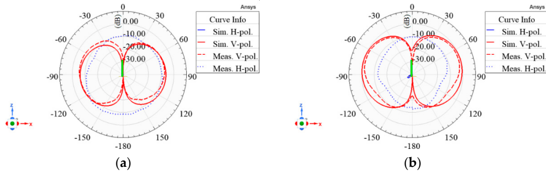
Figure 14. The comparison of the simulated and measured radiation patterns of the proposed antenna in the x-z plane. (a) 2.4 GHz; (b) 5.8 GHz.
