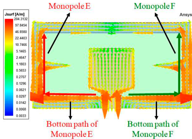
Figure 6. The simulated surface current density at 2.4 GHz.
