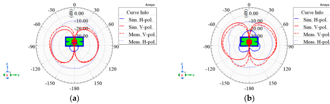
Figure 15. The comparison of the simulated and measured radiation patterns of the proposed antenna in the y-z plane. (a) 2.4 GHz; (b) 5.8 GHz.
