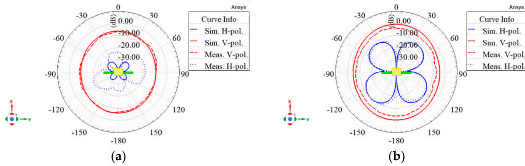
Figure 13. The comparison of the simulated and measured radiation patterns of the proposed antenna in the x-y plane. (a) 2.4 GHz; (b) 5.8 GHz.
