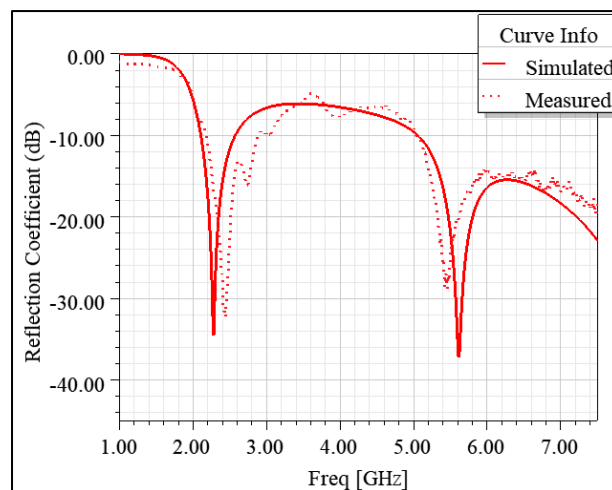
Figure 12. The comparison of the simulated and measured reflection coefficients of the proposed antenna.
