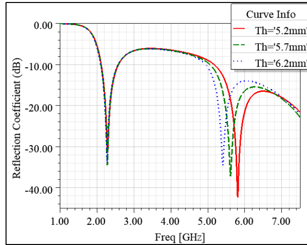
Figure 7. The simulated reflection coefficients for different values of T_h .
