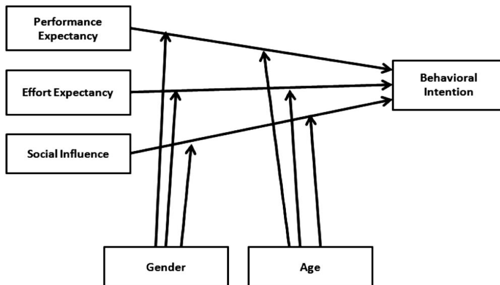
Figure 1. Empirical Model.
